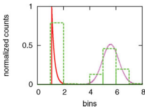
Fig. 10. With pulsed excitation, in the absence of jitter, a lifetime value much shorter than the bin size gives “delays” all in the same bin so that small changes in lifetime result in identical histograms. The solid curve at bin 1 represents this case in which the center of mass of the distribution cannot be determined with a precision better than the bin size. In the presence of jitter, the broadening of the distribution of delays gives different bin contents even if the changes in lifetime are very small. The dotted curve, which is the convolution of the solid curve with a Gaussian jitter, shows that bin 4 contains less counts than bin 6 so that the center of mass of the distribution can be determined with precision better than the bin size. [Color figure can be viewed in the online issue, which is available at www.interscience.wiley.com .]
