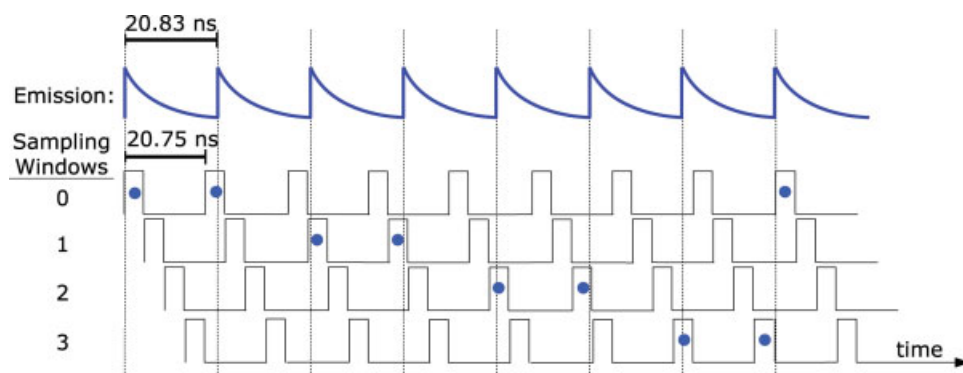
Fig. 1. An illustration of the digital heterodyning principle, with exaggerated heterodyning such that f_{cc} = f_s/8 instead of f_{cc} = f_s/256 which we used in our implementation. Arriving photons (dots) are assigned to one of four sampling windows according to their arrival
