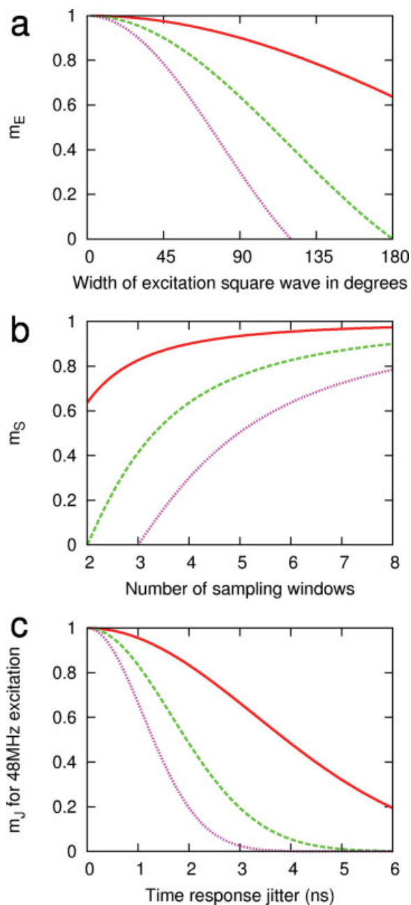
Fig. 6. Plots showing the contribution to the modulation of the instrument response for the first three harmonics. (a) Square wave excitation of variable width (in degrees). (b) Number of digital sampling windows. (c) Gaussian time-response jitter of a given width (in ns). Solid, dashed, and dotted lines are for the 1st, 2nd, and 3rd harmonics, respectively. [Color figure can be viewed in the online issue, which is available at www.interscience.wiley.com .]
