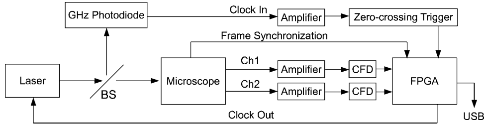
Fig. 3. Experimental setup with the FLIMBox attached to a microscope. The microscope provides the signals from two detectors Ch1 and Ch2 and a Frame Synchronization signal. The FPGA unit is programmed by custom firmware to perform the digital frequency domain acquisition.
