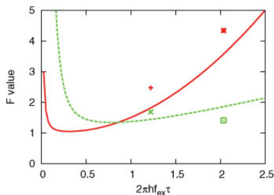
Fig. 8. The theoretical minimum F values for \tau_p (solid line) and \tau_m (dashed line) are shown as a function of 2\pi h f_{ex} \tau for instrument response modulation values of 0.99. The + and x symbols show the F values for the \tau_p and \tau_m of fluorescein in pH 10 solution taken with the FLIMBox at 48 MHz, while the * and □ symbols show the F values for the same sample measured with the TCSPC system at 80 MHz. The F value for \tau_m of the TCSPC measurement is anomalously low due to a clustering of the modulation values resulting from the dead zones at the edges of the card's phase histogram. [Color figure can be viewed in the online issue, which is available at www.interscience.wiley.com .]
