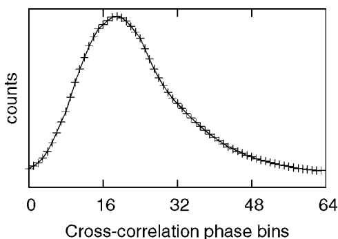
Fig. 2. A histogram of counts received at each phase value of the cross-correlation period. For this figure the phase values have been divided into 64 bins. Plots such as this one contain the exponential decay of a fluorophore, convolved by the instrument response function.
