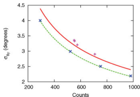
Fig. 7. A comparison of the phase uncertainty for fluorescein measurements as a function of counts between a Becker & Hickl card Model 830 on an 80 MHz 2-photon system (solid line, + symbol) and the FLIMBox on a diode laser system driven at 48 MHz (dashed line, x symbol). Per equal counts, the uncertainty for the B&H card is higher than the FLIMBox card due to the increased demodulation of the fluorescein signal at 80 MHz with respect to 48 MHz. However, all the uncertainties are close to the values predicted by the mathematical model when this demodulation is taken into account. [Color figure can be viewed in the online issue, which is available at www.interscience.wiley.com .]
