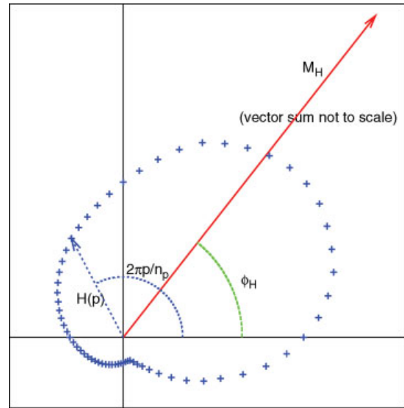
Fig. 5. The cross-correlation phase histogram bins (crosses) for fluorescein are plotted in polar coordinates, forming n_p = 64 vectors. One vector H(p) of the series is identified in the figure. The M_H vector which represents the phase and modulation of the first harmonic is produced by the vector sum of each vector in the phase histogram series.
