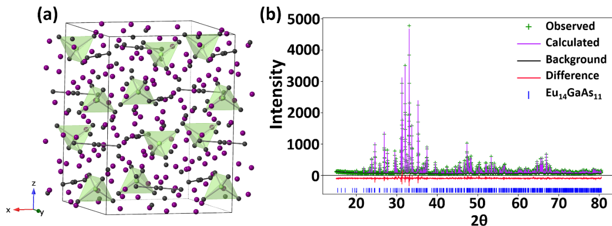
Fig. 1 (a) The crystal structure of tetragonal \text{Eu}_{14}\text{GaAs}_{11} , where purple spheres represent Eu, mint green spheres represent Ga, and black spheres represent arsenic. (b) Rietveld refinement of the PXRD pattern of \text{Eu}_{14}\text{GaAs}_{11} . The green markers correspond to observed data, the magenta line represents the calculated diffraction pattern, the red line represents the difference between observed and calculated data, and the blue lines represent the expected peaks from the crystal structure.
