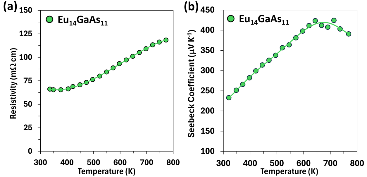
Fig. 4 Temperature-dependent (a) electrical resistivity and (b) Seebeck coefficient of \text{Eu}_{14}\text{GaAs}_{11} .
