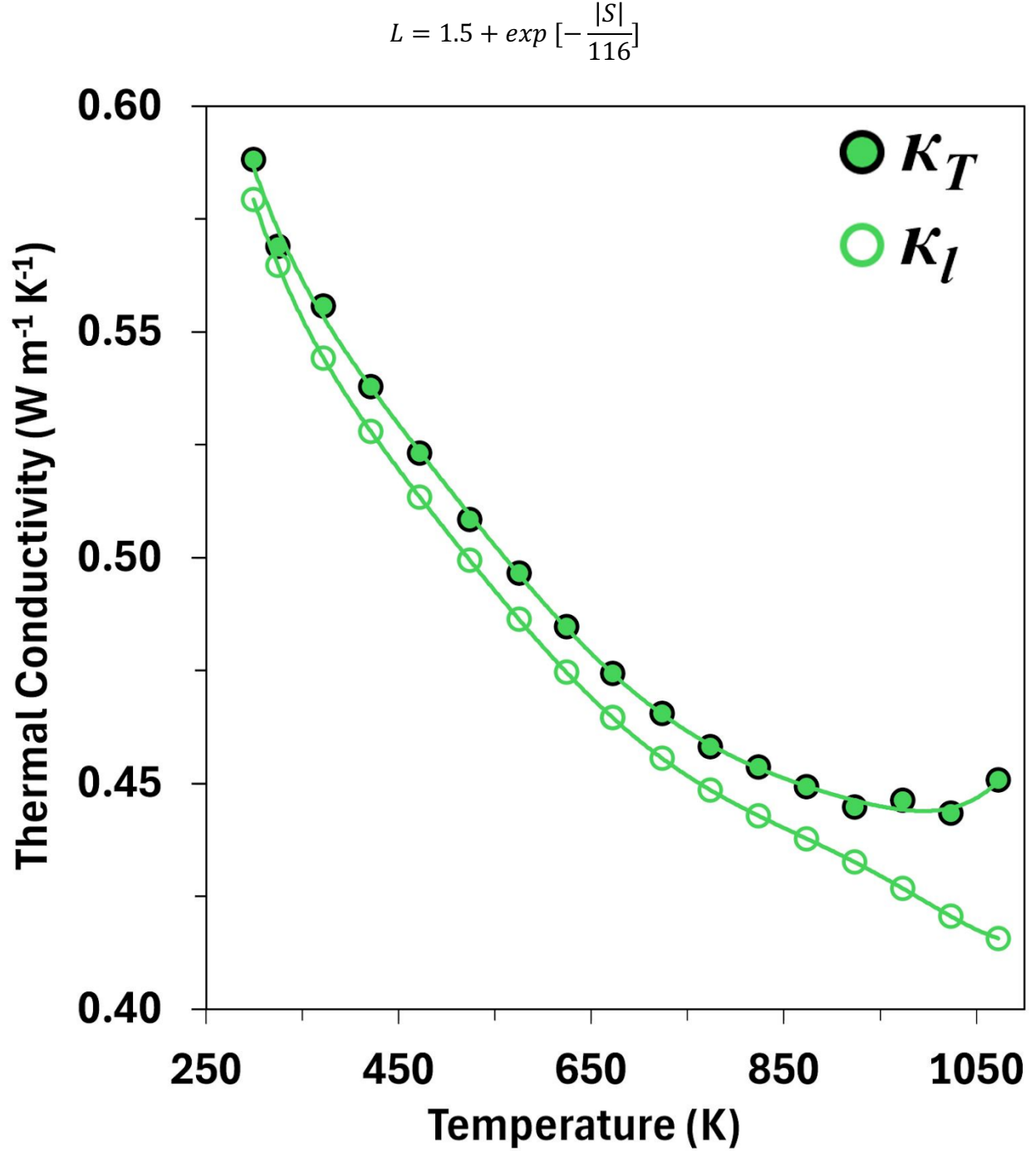
Fig. 7 The total thermal conductivity ( \kappa_T ) and the lattice thermal conductivity ( \kappa_l ) of \text{Eu}_{14}\text{GaAs}_{11} as a function of temperature.
