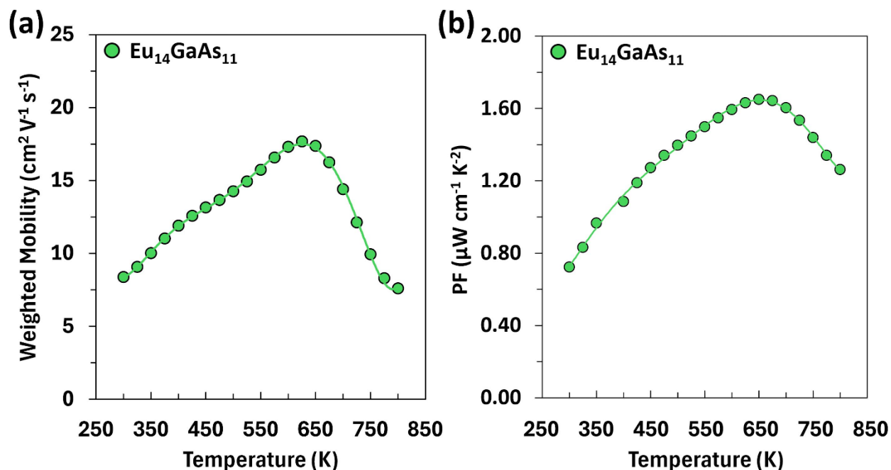
Fig. 6 The (a) weighted mobility and (b) power factor ( PF ) as a function of temperature of \text{Eu}_{14}\text{GaAs}_{11} .
