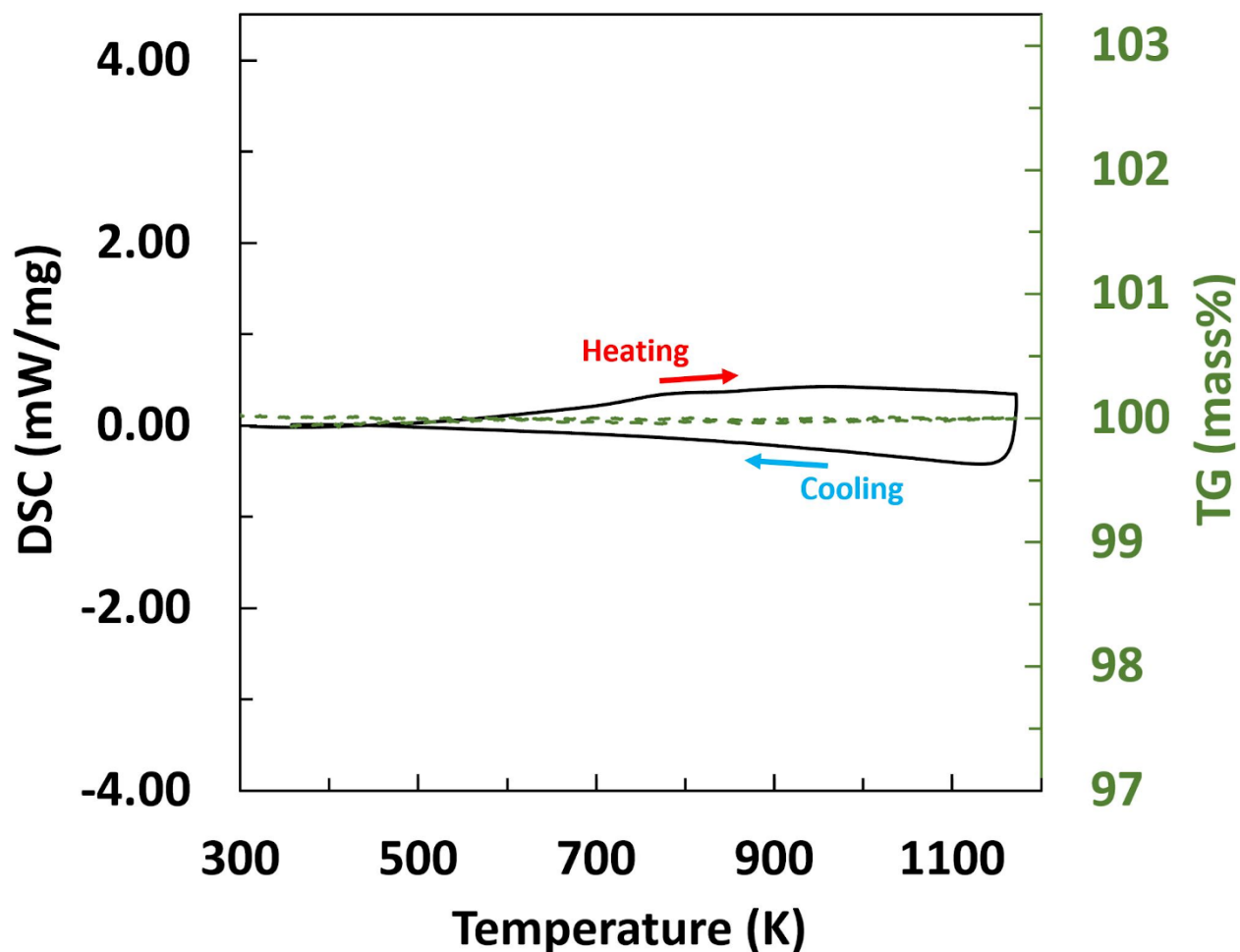
Fig. 3 Thermogravimetry (TG) and differential scanning calorimetry (DSC) of a piece of pressed pellet of \text{Eu}_{14}\text{GaAs}_{11} from room temperature to 1175 K under Ar flow.
