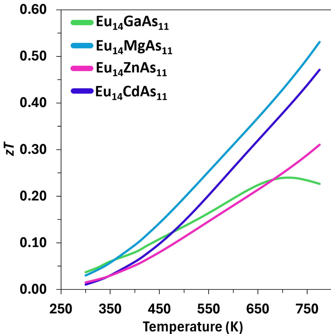
Fig. 8 Temperature-dependent figure of merit zT of \text{Eu}_{14}\text{GaAs}_{11} , \text{Eu}_{14}\text{MgAs}_{11} , 25 \text{Eu}_{14}\text{ZnAs}_{11} , 25 and \text{Eu}_{14}\text{CdAs}_{11} . 25
