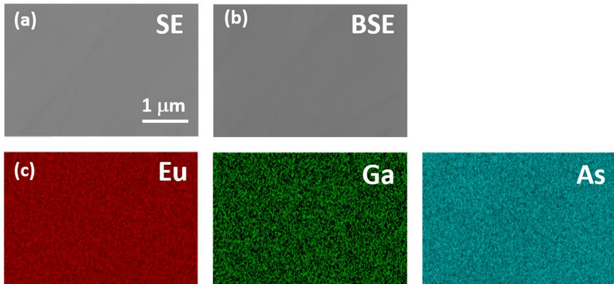
Fig. 2 (a) Secondary electron (SE) image, (b) backscattered electron (BSE) image of a pressed pellet of \text{Eu}_{14}\text{GaAs}_{11} , and (c) corresponding elemental mapping images of Eu, Ga, and As, respectively. The scale bar is the same for all images.
