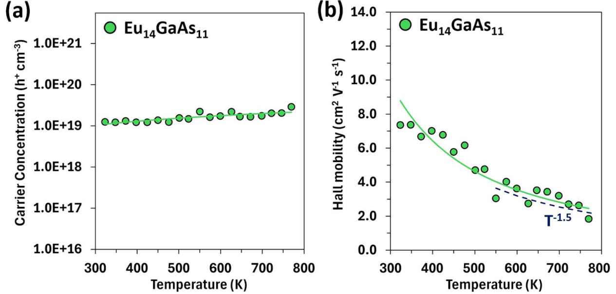
Fig. 5 Temperature-dependent (a) Hall carrier concentration and (b) Hall mobility of \text{Eu}_{14}\text{GaAs}_{11} .
