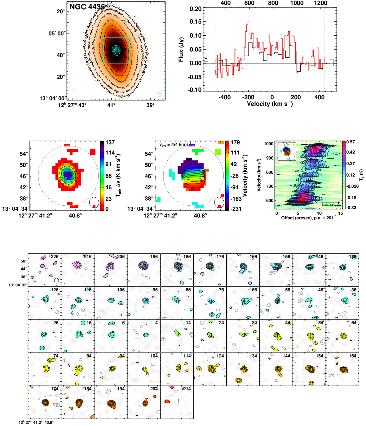
Figure A.17 NGC 4435 is a Virgo regular rotator ( M_K = -23.82 ) that includes two velocity maxima, with a normal stellar morphology. It contains a dust disc. The moment0 peak is 20 \text{ Jy beam}^{-1} \text{ km s}^{-1} . The moment1 contours are at 30 \text{ km s}^{-1} intervals.
