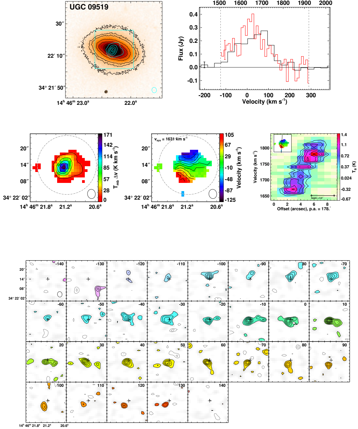
Figure A.30 UGC 09519 is a field regular rotator ( M_K = -21.98 ) with normal stellar morphology. It contains dust filaments. The moment0 peak is 18 \text{ Jy beam}^{-1} \text{ km s}^{-1} .
