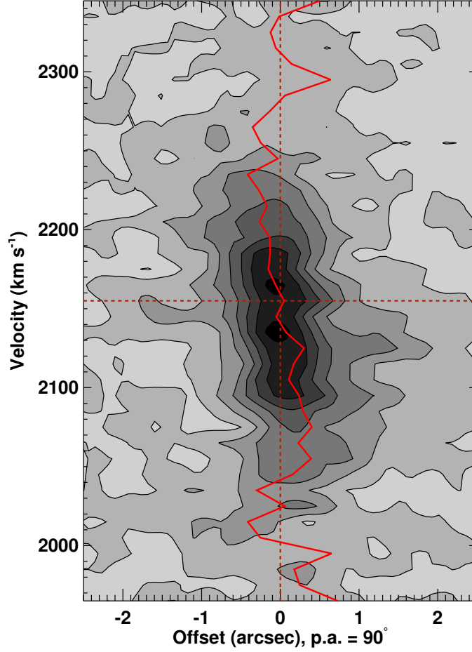
Figure 3.11 Position-velocity diagram of NGC 1266 for our CO(1–0) A and B array CARMA data, taken at position angle of 90°. The observed lack of a turnover is indicative of the gas not reaching the flat part of the rotation curve. The data are consistent with rotation with a gradient of 1.8 \text{ km s}^{-1} \text{ pc}^{-1} in the inner parts. The red line is a trace of the peak at each velocity. The dark red dashed lines indicate v_{\text{sys}} and the center.
