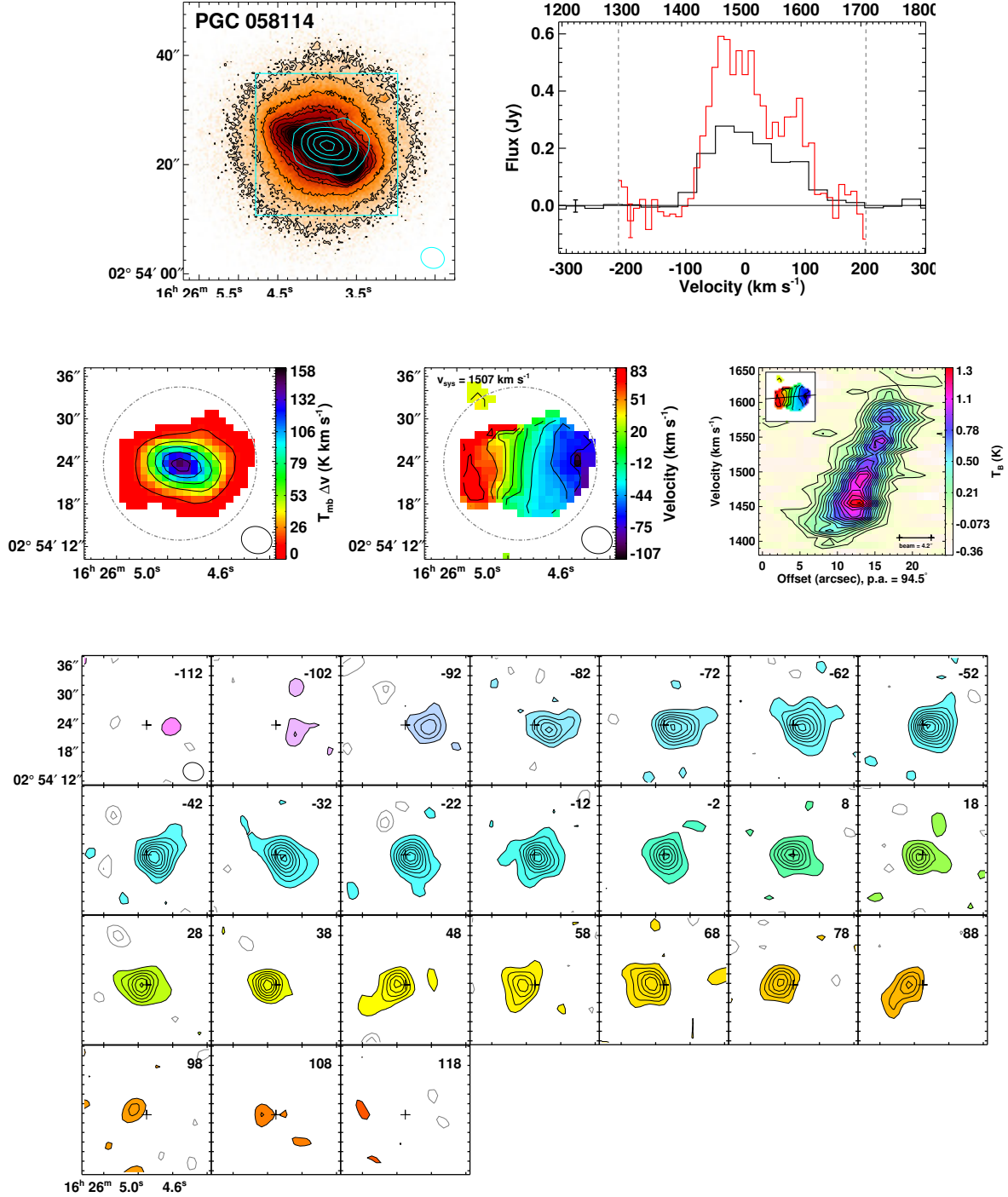
Figure A.27 PGC 058114 is a field galaxy ( M_K = -21.57 ) with unknown kinematic structure or morphology. The moment0 peak is 28 \text{ Jy beam}^{-1} \text{ km s}^{-1} . Channel map and PVD contours are placed at 2\sigma intervals.
