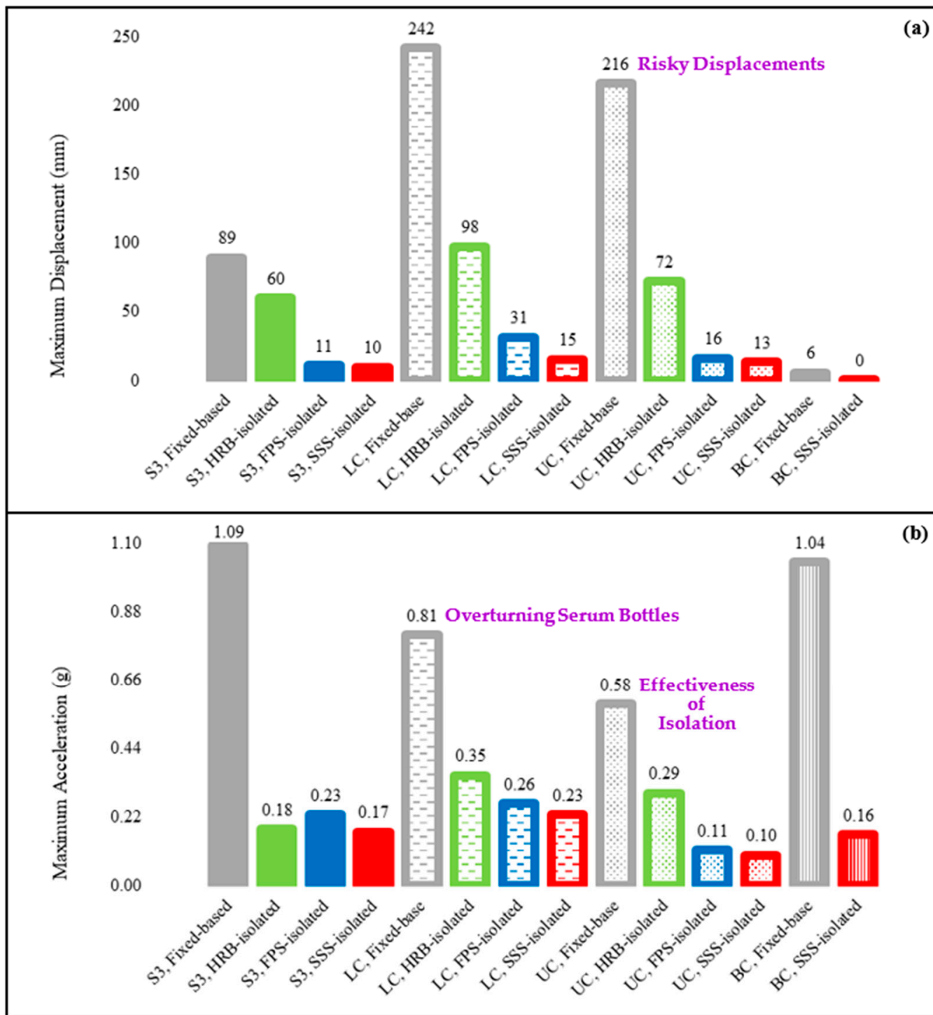
Figure 12. Maximum (a) displacements and (b) accelerations of the ground motion GM4 (used to generate the input excitations for the shaking table tests), the third story (S3) of the hospital building in all the fixed-base and base-isolated (HRB, FPS, and SSS-isolated) cases subjected to GM4, and the cart in all the locked (LC), unlocked (UC), and braced (BC) conditions in the fixed-base and base-isolated cases.
