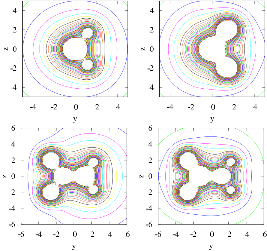
Figure 9: Potential energy functions in the static-exchange approximation with exchange represented by the local Hara free-electron gas approximation. Top left CH 4 in the HCH plane. Top right CF 4 in the FCF plane. Bottom left difluoroethylene in molecular plane with 1s vacancy in C H . Bottom right difluoroethylene with 1s vacancy in C F . Contours begin at -2 hartrees in increments of 0.2 hartrees with distances in bohr.
