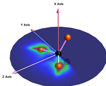
Figure 1: Distribution of momenta of the F^+ ions measured in coincidence from the dissociation of CF_4 after core hole ionization followed by Auger decay, plotted in the FCF molecular plane.
