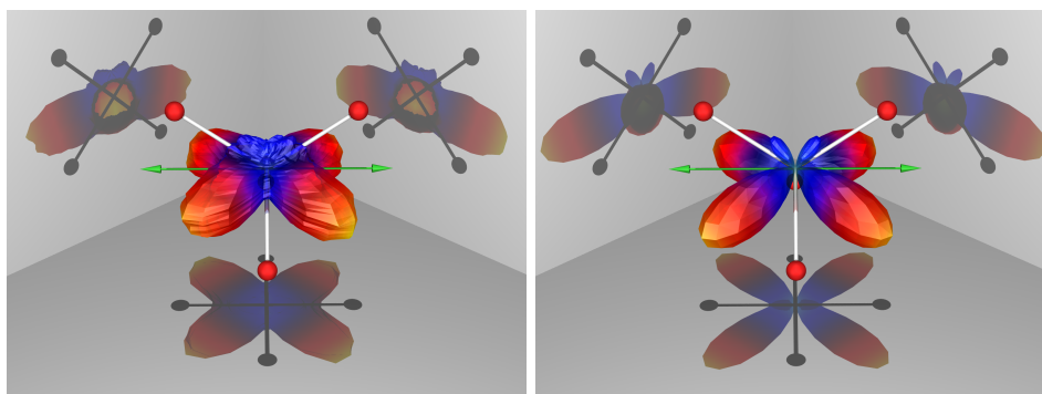
Figure 6: MFPAD for K-shell ionization of \text{CF}_4 with the polarization fixed perpendicular to the \text{C}_2 axis and in the plane of two C-F bonds. Left: the observed photoelectron distribution measured in coincidence with \text{F}^+ + \text{F}^+ following Auger decay. Right: the MFPAD calculated using the complex Kohn variational method. The equilibrium molecular geometry is represented by the ball and stick models and the polarization axis by the double headed arrow.
