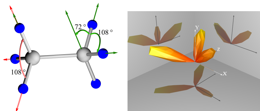
Figure 3: Left: Approximate relative angles between the momenta of three emerging protons under the assumption of recoil along the directions of bonds. Dashed arrows indicate three protons from the same carbon, and solid arrows indicate two protons from one side and one from the other. Right: Observed proton angular distribution that was used to produce the experimental MFPAD in Figure 2 .
