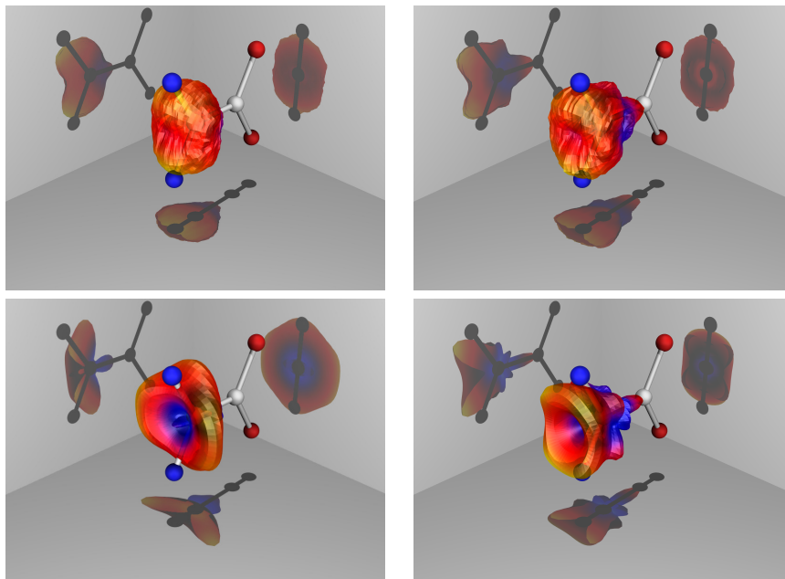
Figure 7: MFPADs of C_2H_2F_2 where the carbon on H_2 side was ionized in experiments performed at two different photon energies: h\nu = 296 eV and h\nu = 301 eV. Top row: experiment 4-6 eV and 8-12 eV photoelectrons. Bottom row: complex Kohn results at photoelectron energies of 5.44 eV and 10.88 eV.
