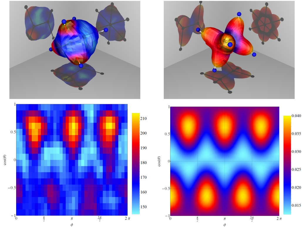
Figure 2: MFPAD for C_2H_6 at 4.5 eV above the C 1s threshold from analysis of the experimental data assuming the three protons in the breakup channel C_2H_6 + h\nu \rightarrow H^+ + H^+ + H^+ + \text{neutrals} + 3e^- originated from the same carbon atom (left column) and complex Kohn calculations at 4.35 eV (right column).
