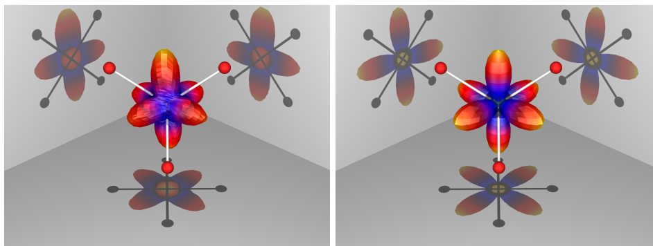
Figure 5: MFPAD for K-shell ionization of \text{CF}_4 . Left: the observed photoelectron distribution measured in coincidence with \text{F}^+ + \text{F}^+ following Auger decay. Right: the MFPAD calculated using the complex Kohn variational method. Data and theory are integrated over all orientations of the polarization vector. The equilibrium molecular geometry is represented by the ball and stick models.
