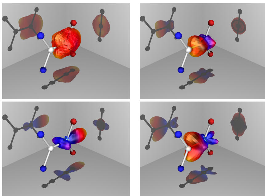
Figure 8: MFPADs of C_2H_2F_2 where the carbon on F_2 side was ionized in experiments performed at two different photon energies: h\nu = 296 eV and h\nu = 301 eV. Top row: experiment 0-2 eV and 3-6 eV photoelectrons. Bottom row: complex Kohn results at photoelectron energies of 1.09 eV and 4.35 eV.
