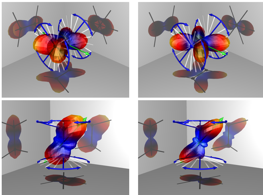
Figure 4: RFPADs for the \text{CH}_3^+ + \text{CH}_3^+ break up channel from experiment (left column) and complex Kohn calculations (right column) with polarization perpendicular to the C-C bond (top row) and at 45^\circ to the C-C axis (lower row). The curved arrows indicate the effective averaging around the C-C bond axis that occurs in this RFPAD measurement.
