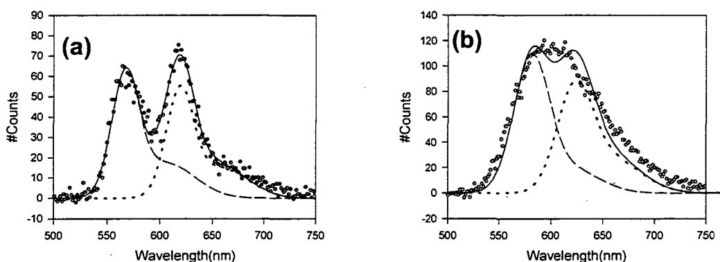
Fig.6.11. Typical spectra (gray circles) obtained on single TMR-20-TR (a) and single TMR-10-TR (b) samples. A small background remains after bleaching of both molecules, and has been subtracted. TMR and TR base-functions are used to fit (a) and (b). The data in (a) can be fit well (solid line) to a superposition of donor (dashed-line) and acceptor (dotted-line) emission, while the broad and featureless spectrum in (b) cannot be fit well
