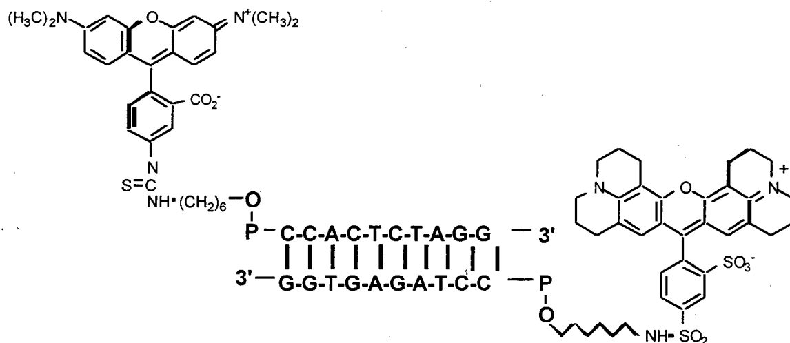
Fig.6.7. Model system of single pair of donor and acceptor fluorophore. The donor is tetramethylrhodamine (TMR) and is attached to the 5' end of a single strand of DNA (10mer or 20mer) through a flexible link of 6 carbon chain. The acceptor is Texas red (TR) and is also bound to a single strand of DNA complementary to the donor strand.
