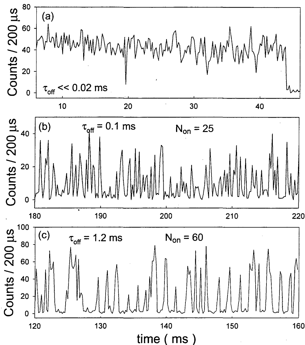
Fig.5.10. Time traces of three TR-DNA molecules measured with the far-field excitation. (a) Relatively quiet emission meaning triplet state lifetime much shorter than 0.02ms. Telegraph noise, arising from on-off transitions is evident in (b) and (c). \tau_{\text{off}} and N_{\text{on}} are estimated by building histograms of on-state counts and off-state duration..
