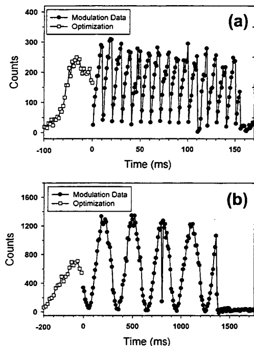
Fig.A.5. Intensity (a) and polarization (b) modulation spectroscopy performed after successful positioning. The modulation was done with an electro-optic modulator combined with a polarizer and/or a quarter-waveplate. Noise due to intrinsic molecular properties such as dark states and spectral jumps is evident both during the positioning and the modulation spectroscopy.
