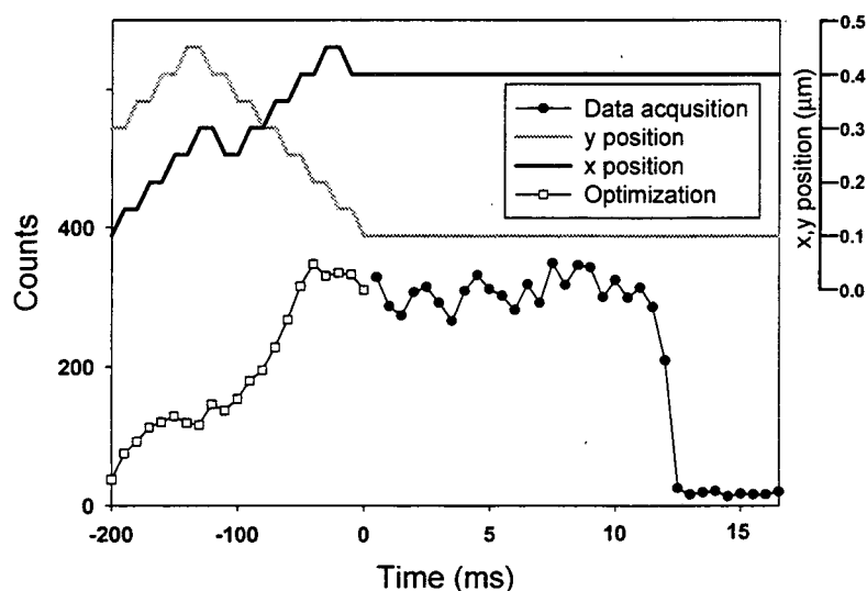
Fig.A.3. Time sequences of photon counts (squares during positioning, circles after positioning is completed), of x -position (solid black line), and of y -position (solid gray line). Note the difference in time scale. The step size for x,y increments was 0.125' w_{PSF} (50nm). The integration time was reduced from 10ms to 0.5ms and the excitation intensity was increased by a factor of 20 after the positioning subroutine was completed.
