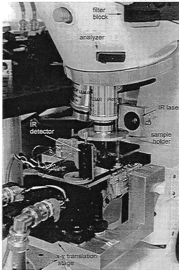
Fig.2.8. Scan head and collection optics.
