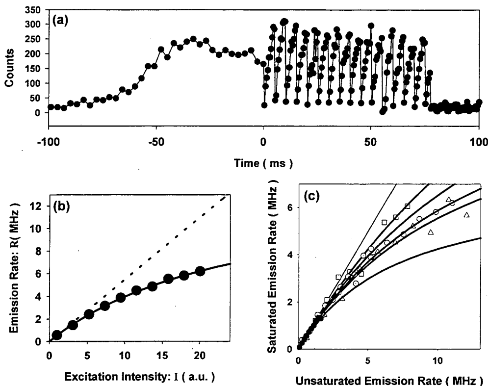
Fig.5.13. Saturation of single molecule emission due to triplet state. (a) After an automated search, intensity modulation up to 20 fold is performed until the photodestruction. (b) Intensity dependent emission rate showing clear saturation (filled circles). The data is obtained by averaging the first 13 modulation periods in (a). The data is fit to the saturation equation discussed in the text. From the curve-fit, a saturation emission rate of 6.5 MHz is extracted. Detector response and detection efficiency are corrected for. The straight line is the emission level expected without saturation due to the triplet state. (c) The result of saturation measurements on six molecules are shown with the saturation curves. The excitation intensity is normalized to the emission rate expected without saturation.
