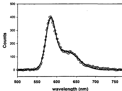
Fig.4.6. Emission spectrum of a single TR-DNA (empty circles). Solid line is a two-gaussian fit to the data. Integration time = 5s.
