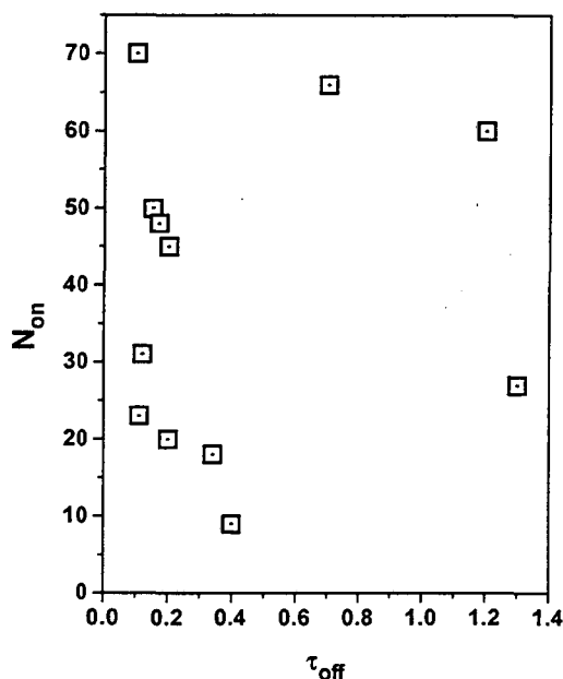
Fig.5.12. Relation between \tau_{\text{off}} and N_{\text{on}} . For each molecule with measurable \tau_{\text{off}} and N_{\text{on}} , a square is plotted. No simple relation between them could be found.
