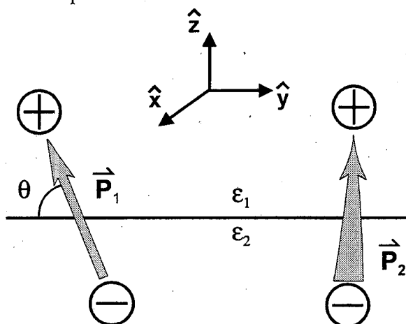
Fig.6.6. Interaction of two dipoles at the interface between two media.
