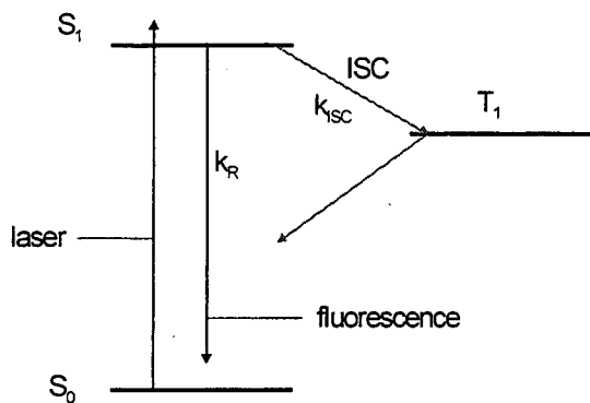
Fig.5.9. Energy level diagram for typical fluorescent molecules. Main transitions happen between singlet ground state ( S_0 ) and singlet excited state ( S_1 ). Spin forbidden transition to the triplet state ( T_1 ) or intersystem crossing (ISC) happens with a low probability. The molecule returns to the singlet ground state via intersystem crossing or phosphorescence.
