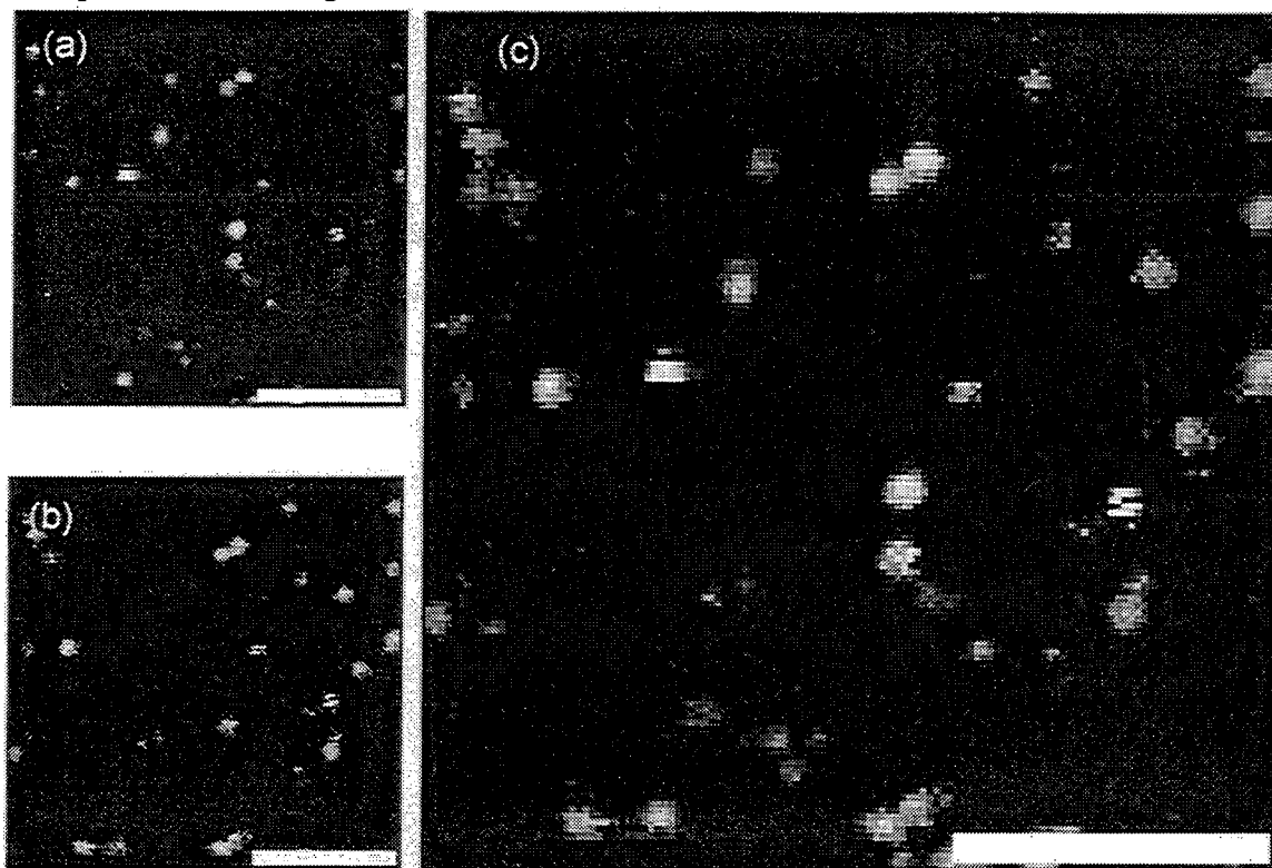
Fig.6.10. Two-color near-field scanning fluorescence images of doubly labeled DNA molecules (scale bar is 1 \mu\text{m} ). (a) is for the donor channel image and (b) is for the acceptor channel. Both images were obtained simultaneously by separating the emission with a dichroic mirror. The two color images are overlaid to form the composite image of (c). The correlation between (a) and (b) can be used as a crude estimate of the degree of DNA hybridization on the dry surface.
