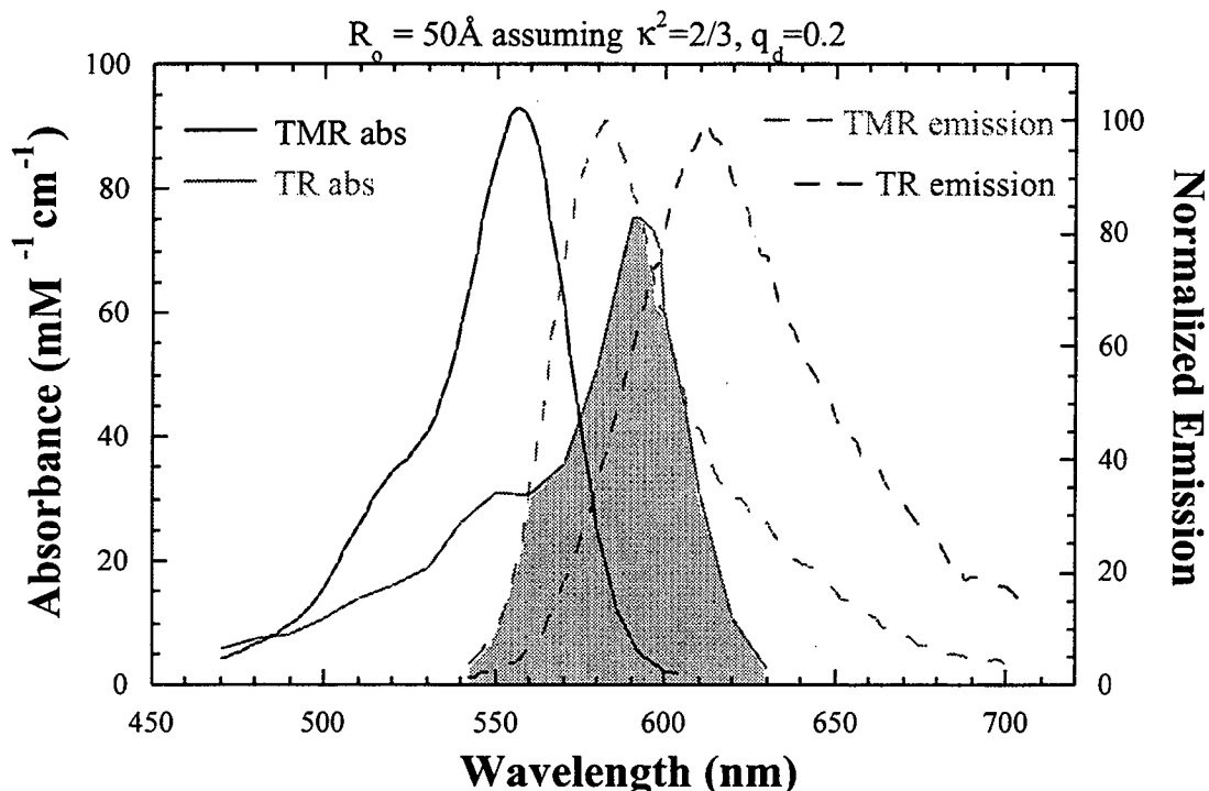
Fig.6.8. Solution spectra of donor-DNA system and acceptor-DNA system. Absorption spectra are in solid lines and emission spectra are in dashed lines. The spectral overlap between the donor emission and the acceptor absorption is considerable and is schematically shaded. Based on the solution measurement, R_o of 50 Å is calculated assuming \kappa^2=2/3 and q_d=0.2 .
