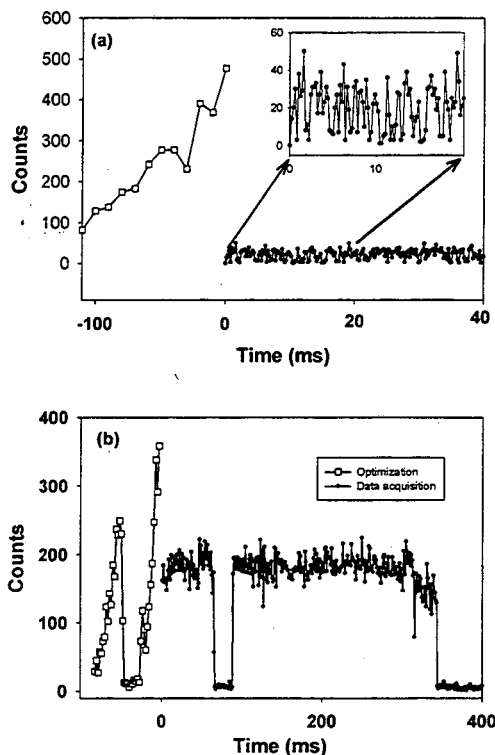
Fig.A.4. Immunity of the positioning algorithm to intrinsic noise: (a) quantum jumps to triplet states. Inset is the zoom-out showing individual jumps. 10ms integration for positioning and 0.2ms integration for data were used. (b) Long dark states during and after the completion of the positioning subroutine.
