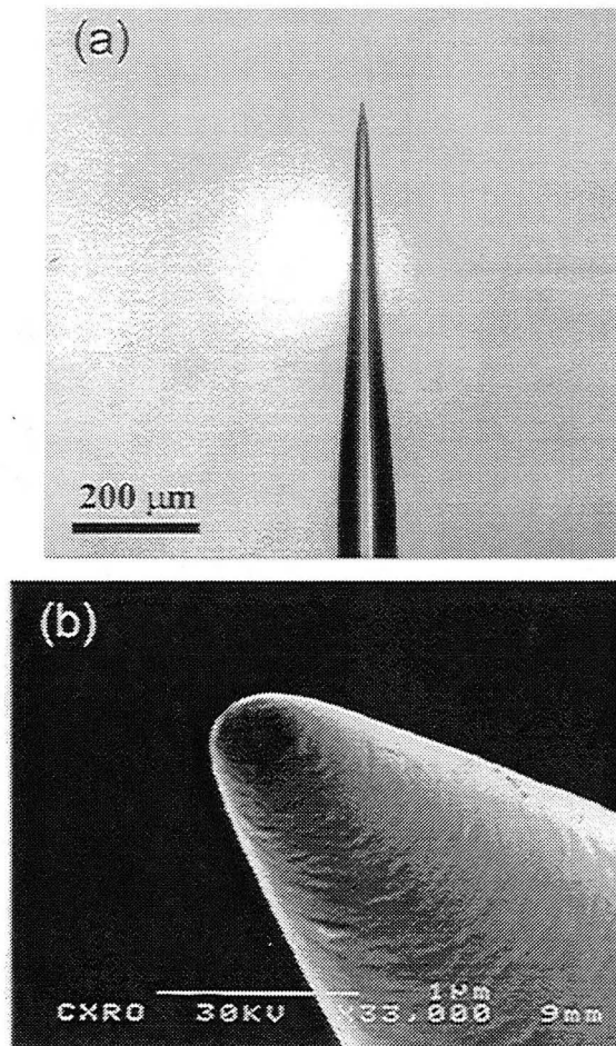
Fig.2.3 Optical and electron micrographs of tips. (a) optical micrograph of freshly pulled, uncoated fiber. (b) SEM image of aluminum coated fiber.
