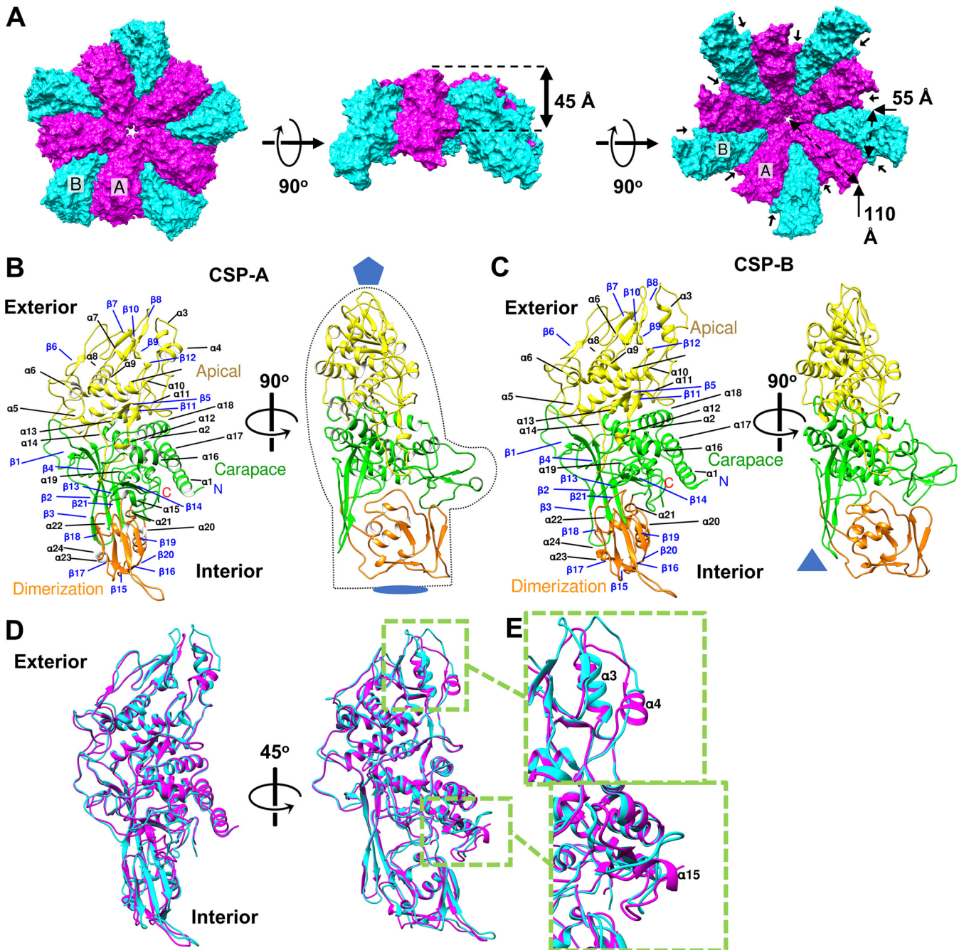
FIG 2 Characterization of the capsid shell protein. (A) Surface diagrams of decamer subunits with CSP-As (magenta) nearest the I5 vertex and surrounded by CSP-Bs (cyan) viewed from the exterior (left), side (middle), and interior (right). Approximate measurements of the conformer dimensions are overlaid in Å. Stabilizing protrusions are labeled with black pointers. (B and C) Orthogonal views of A and B conformers (CSP-A and CSP-B), respectively, with secondary structural elements labeled, symbols indicating sites of icosahedral symmetry, and mitten shape provided to enhance visualization. Colored: carapace, green; apical, yellow; dimerization domain, orange. (D) Ribbon diagram of CSP-A (magenta) and CSP-B (cyan) superimposed upon one another. (E) Close-up view of sites of structural discrepancies between conformers display on winding of \alpha 4 (top) and \alpha 15 (bottom) from CSP-A to CSP-B.
