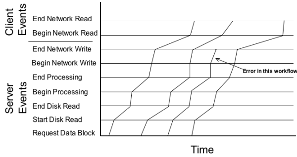
Figure 1. NetLogger Lifelines.
