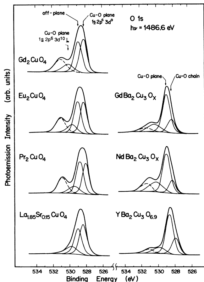
FIG. 5. O 1s core-level spectra analogous to those of Fig. 3. In all cases, two components of approximately equal intensity are found for the 2:1:4 compounds (planes and off planes as identified). For the 1:2:3 compounds, the emission from oxygen in the Cu-O planes dominates that from chains. For the single crystals, it is probable that part of the emission at \sim 531 eV is due to contamination, as discussed in the text, and the fittings to reveal the satellite structure are only qualitative.
