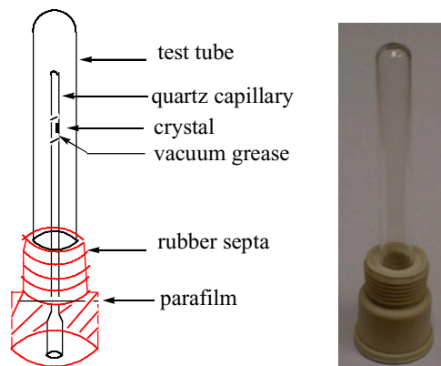
Figure 1. Test tube/capillary/septa assembly
