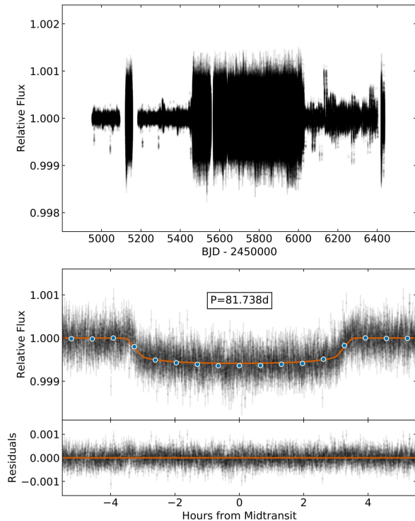
Figure 1. Transit plot of Kepler-538b. The top subplot is the pre-search data conditioning (PDC) Kepler photometry. The top panel of the bottom subplot shows the phase-folded photometry in and near the transit of Kepler-538b, with the best-fit transit model in orange and binned data in blue. The bottom panel of the bottom subplot shows the photometric residuals after subtracting the best-fit transit model.
