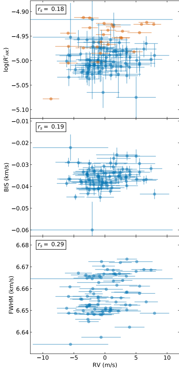
Figure 4. Scatter plots of RV vs. \log R'_{HK} , BIS, and FWHM for Kepler-538. The RVs have been mean-subtracted and plotted against the other three data types. Blue data points correspond to HARPS-N observations, orange data points to HIRES. In the top left corner of each panel is the Spearman correlation coefficient between the two data sets, an indicator of nonlinear, monotonic correlation. (The coefficients were calculated using the observation values but not their uncertainties.)
