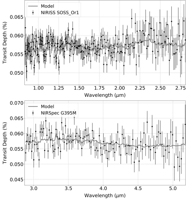
Figure 8. A simulated transmission spectrum of Kepler-538b with five transits observed with JWST . The model spectrum, with low metallicity (five times solar) and no clouds, is shown as a gray line. The black data points are the simulated instrument spectra, using NIRISS SOSS-Or1 (0.81–2.81 \mu\text{m} ) and NIRSpec G395M (2.87–5.18 \mu\text{m} ).
