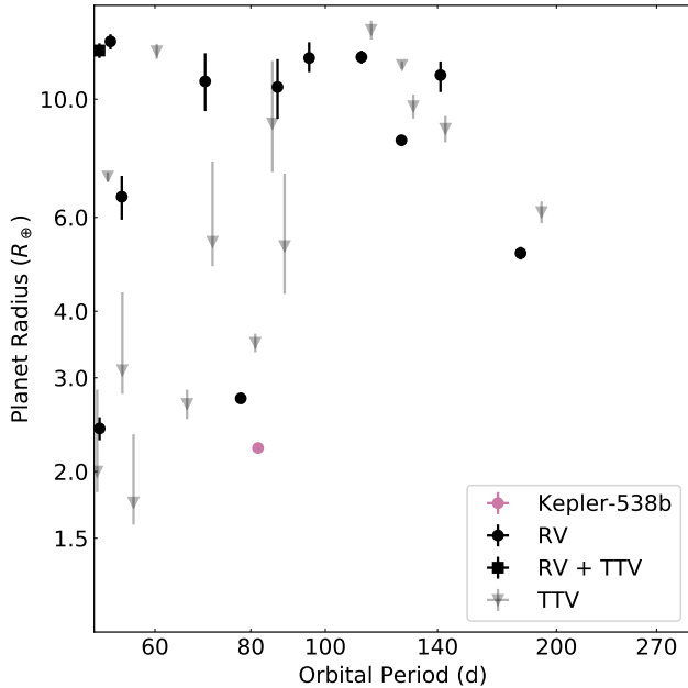
Figure 7. Orbital period versus planet radius for all transiting exoplanets with P > 50 days and RV or transit timing variation (TTV) mass measurements. Data for all planets besides Kepler-538b were retrieved from the NASA Exoplanet Archive (accessed 2019 February 16). Kepler-538b is plotted as a pink circle, all other exoplanets with RV mass measurements are plotted as black circles, one exoplanet (Kepler-117c) has a jointly derived mass from RV and TTV measurements and is plotted as a black square, and exoplanets with only TTV mass measurements are plotted as gray triangles. (Period and radius uncertainties are plotted for all planets, including Kepler-538b, but are smaller than the data points in many cases.) At long periods ( P > 50 days), Kepler-538b is the smallest transiting exoplanet with an RV mass measurement, and Kepler-20d is the only such planet with a lower mass (by 0.5M_{\oplus} ). Overall, there are very few mass measurements for planets in the long-period, small-radius regime of Kepler-538b.
