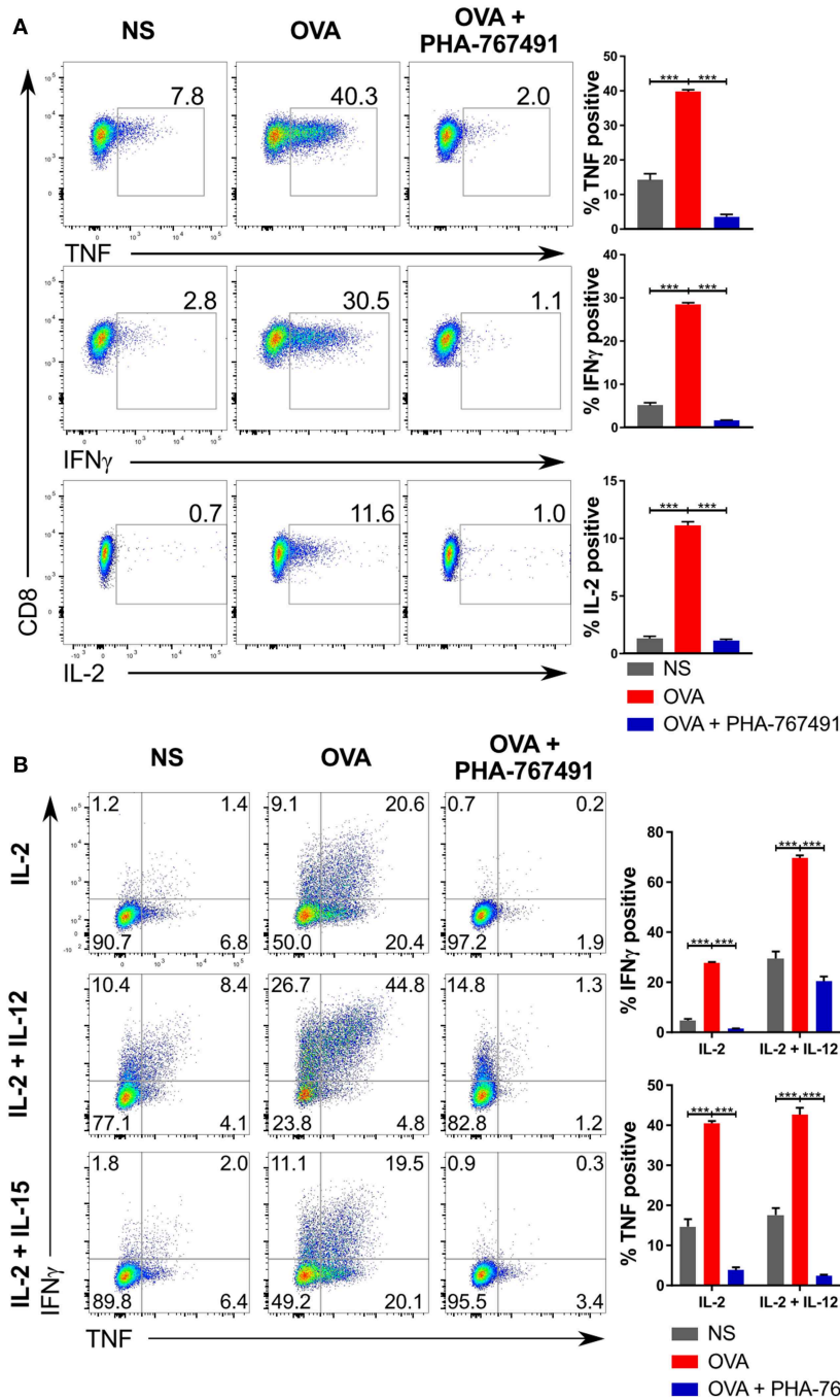
FIGURE 4 | Suppression of cytokine production by PHA-767491. (A) PHA-767491 suppresses cytokine production in OT-I CTL. APCs expressing single chain H-2K b with OVA peptide were seeded into 96 well plates 1 day prior to the experiment. CTL were pre-treated with BFA for 30 min before co-culturing with the APCs for 6 h. The percentages of the positive population of each sample are indicated for each plot. (B) PHA-767491 also suppresses cytokine production in strongly polarized OT-I CTL. For the preparation of the OT-I CTL, OT-I splenocytes were pre-treated with either 10 nM OVA peptide and 10 U/ml IL-2 only, 10 nM OVA peptide and 10 U/ml IL-2 with 10 ng/ml IL-12, or 10 nM OVA peptide and 10 U/ml IL-2 with 10 ng/ml IL-15. CTL were pre-treated with BFA and restimulated by co-culturing with APCs expressing single chain H-2K b with OVA peptide for 6 h. The percentages of each quadrant in each graph are shown. Data shown is representative of at least three independent experiments. Bar charts are represented as mean \pm SEM. Statistical significance was determined by unpaired two-sided Student's t -test (***) p < 0.001).
