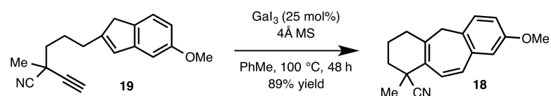
Scheme 3. Cycloisomerization of Indenylalkynes
