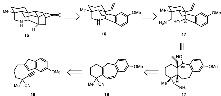
Scheme 2. Synthesis of Alkynylindene 19
