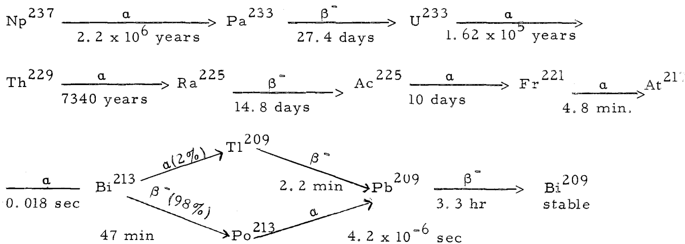
Figure 6. Decay scheme of the neptunium series. 10, 11
