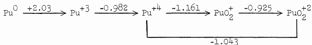
Figure 12. Formal Oxidation Potential Diagram of Plutonium in Perchloric Acid
