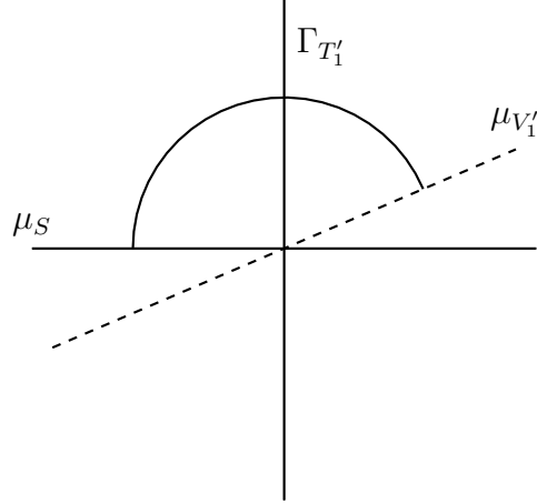
Figure 7.10: Because 0 < q_1/p_1 < 1 , we must have m = 0 .
