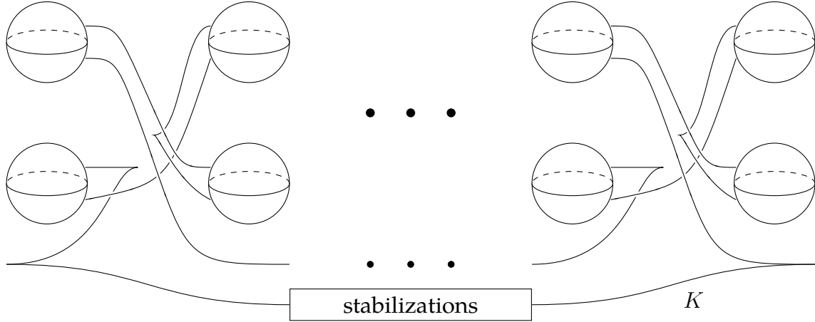
Figure 8.1: Stein handlebody diagrams for filling the tight contact structures on a circle bundle \pi: M \rightarrow \Sigma with t(S^1) = -1 . The diagram has 2g 1-handles, and the knot K has 2g - 2 - e stabilizations in the marked region.
