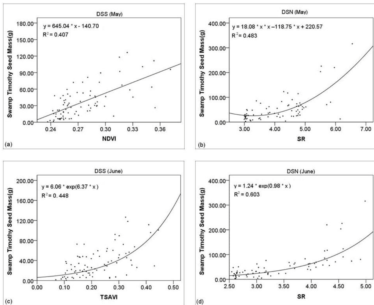
Fig. 3 Observed swamp timothy seed mass(g/m 2 ) plotted to the best correlated vegetation indices in two fields, Ducky Strike North (DSN) and Ducky Strike South (DSS) from aerial photos taken on two different dates (May 11,2006 and June 9,2006).
