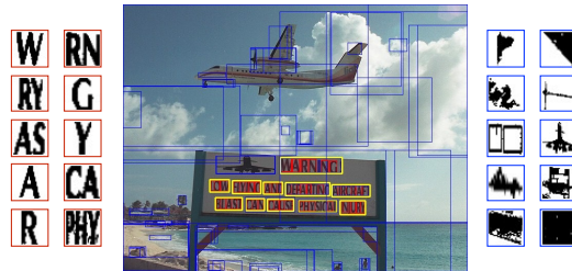
Figure 4. Mining positive (red) and negative (blue) examples from an image that was labeled at word level (yellow rectangles). Only a subset of MSERs are shown on the image for readability.
