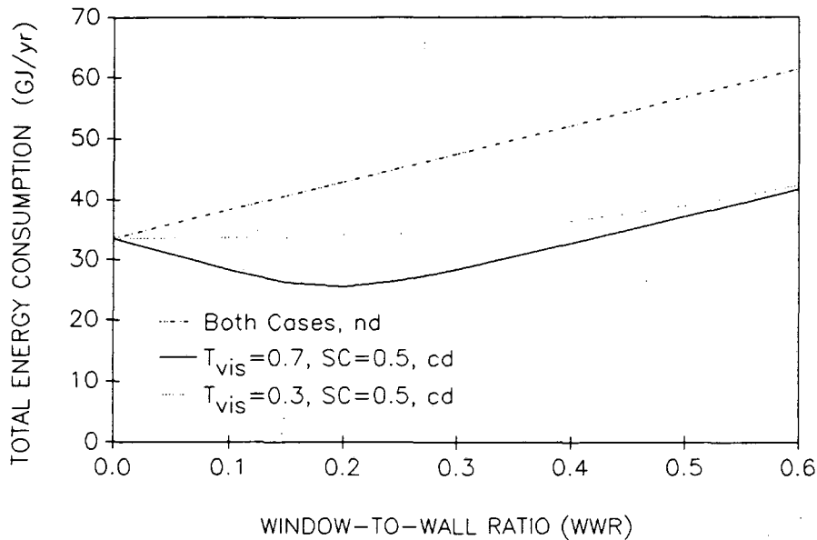
Fig. 1. Total annual energy consumption as a function of the ratio of window area to exterior wall area for the south-facing zone of a Los Angeles office building with a single-zone constant-volume system, a cooling COP of 3.0, a heating efficiency of 0.6, and a lighting power density of 18 \text{ W/m}^2 . The notation is: SC - shading coefficient, T_{vis} - visible transmittance, nd - no lighting controls, cd - lighting controls.
