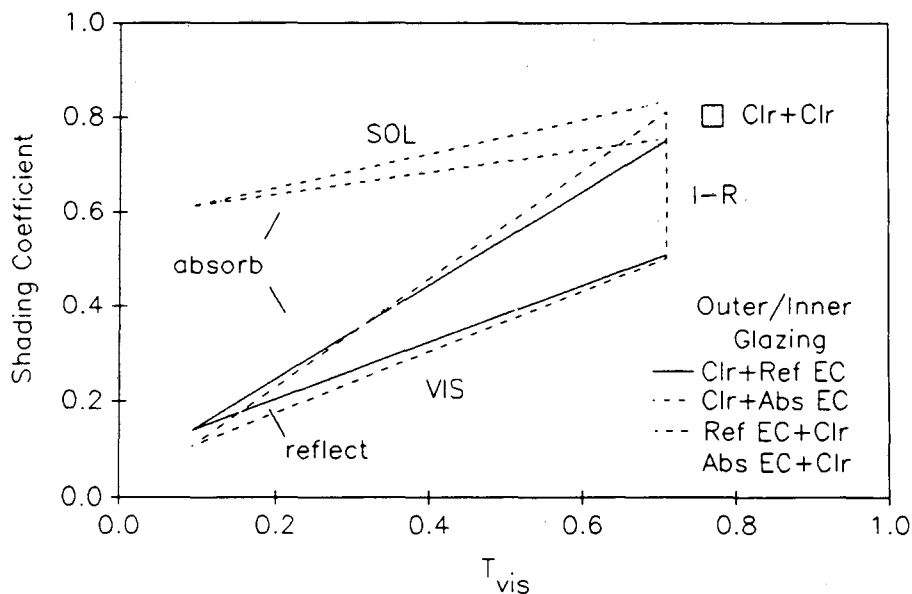
Fig. 6. Performance indices for a double-pane window with clear glass (Clr) and an electrochromic layer with the infrared properties of clear glass (EC). Results are given for reflecting (Ref) electrochromic glazings and absorbing (Abs) electrochromic glazings. For each triangle, the results for a window with: a type SOL electrochromic are represented by the top line; a type I-R are given by the vertical line; and a type VIS are represented by the lower line. The SC and T_{vis} of a window, Clr+Clr, without an electrochromic layer is included for comparison.
