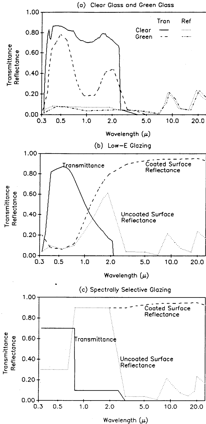
Fig. 3. Transmittance and reflectance spectra of: (a) clear glass and green glass; (b) clear glass with a low-E coating; (c) spectrally selective glazing.
