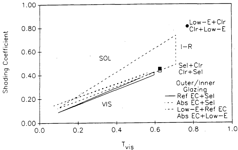
Fig. 7. Performance indices for a double-pane window with either selective glazing (Sel) or low-E glass (Low-E) and an electrochromic layer with the infrared properties of clear glass (EC). Results are given for reflecting (Ref) electrochromic glazings and absorbing (Abs) electrochromic glazings. For each triangle, the results for a window with: a type SOL electrochromic are represented by the top line; a type I-R are given by the vertical line; and a type VIS are represented by the lower line. The SC and T_{vis} of sample windows without an electrochromic layer are included for comparison.
