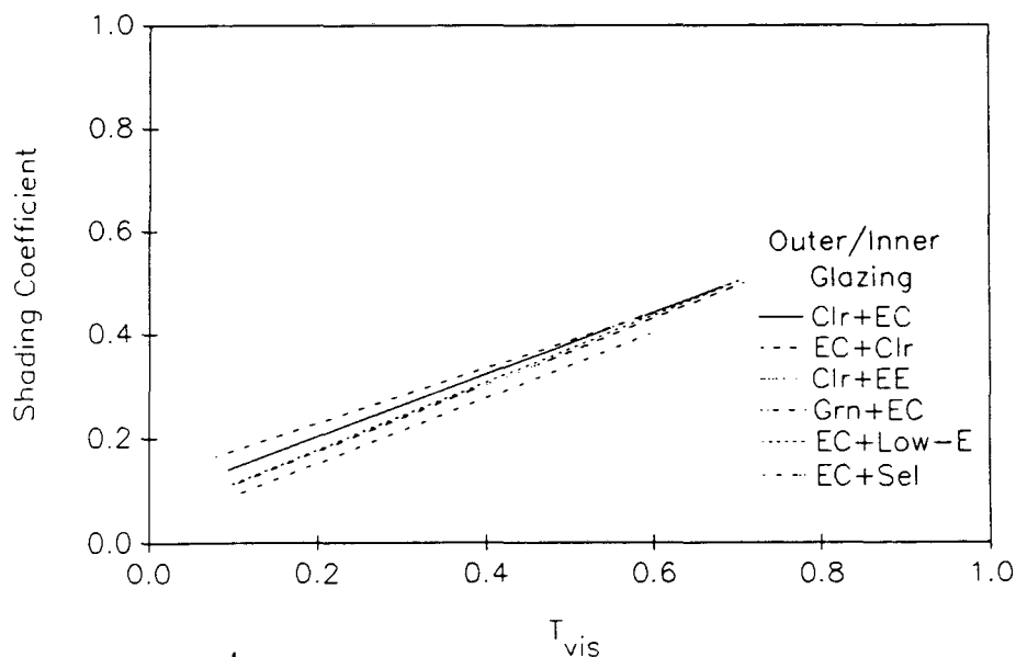
Fig. 8. Performance indices for a double-pane window with either clear glass (Clr), green glass (Grn), low-E glass (Low-E), or selective glazing (Sel) and a reflecting type VIS electrochromic layer (Ref). The electrochromic layer has the infrared properties of clear glass (EC) or low-E glass (EE).
