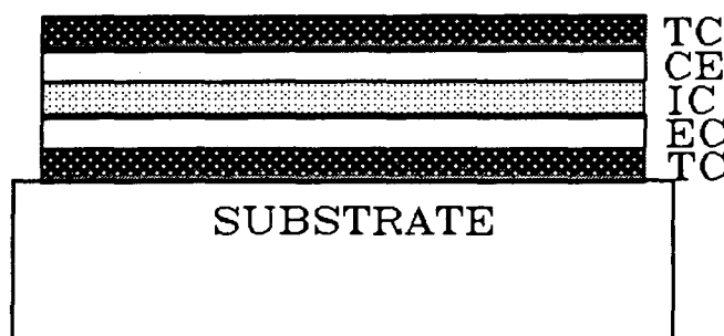
Fig. 2. Schematic of a solid-state electrochromic device: TC – transparent conductor; CE – counter-electrode; IC – ion conductor; and EC – electrochromic.
