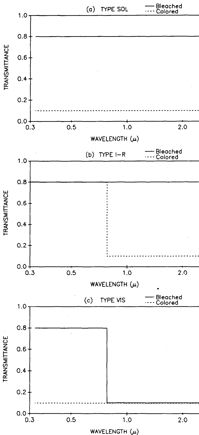
Fig. 4. Solar transmittance spectra of the three electrochromic prototype devices modeled in this study. The properties of the devices switch between the bleached (solid line) and colored (dotted line) states.
