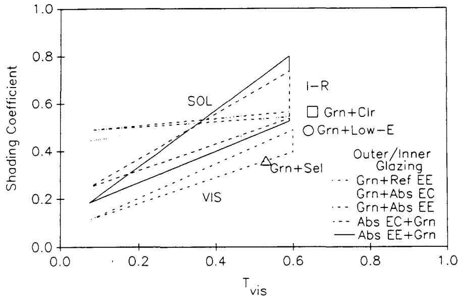
Fig. 9. Performance indices for a double-pane window with green glass (Grn) and an electrochromic layer with the infrared properties of clear glass (EC) or low-E glass (EE). Results are given for reflecting (Ref) electrochromic glazings and absorbing (Abs) electrochromic glazings. The SC and T_{vis} of windows with green glass (Grn) and clear (Clr) or low-E (Low-E) glass are included for comparison.
