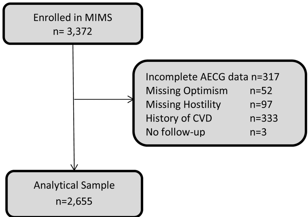
Figure 1 –. STROBE diagram
