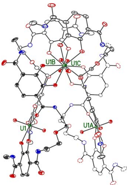
Fig. 1. Crystal structure of [\text{LUO}_2]^{2-}_4 (30% probability) without hydrogen atoms. The four ligands are presented in four different ellipsoid formats. Carbon atoms are grey, nitrogen atoms blue, oxygen atoms red, and uranium atoms green.
