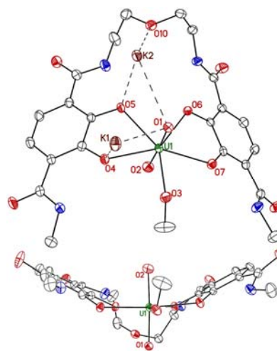
Fig. 2 Crystal structure of [\text{LUO}_2(\text{OMe})]^{2-}_3 (30% probability) without hydrogen atoms. Up: structure of [\text{K}_2\text{LUO}_2(\text{OMe})]^{3-} ; down: side view of [\text{LUO}_2(\text{OMe})]^{2-}_3 .
