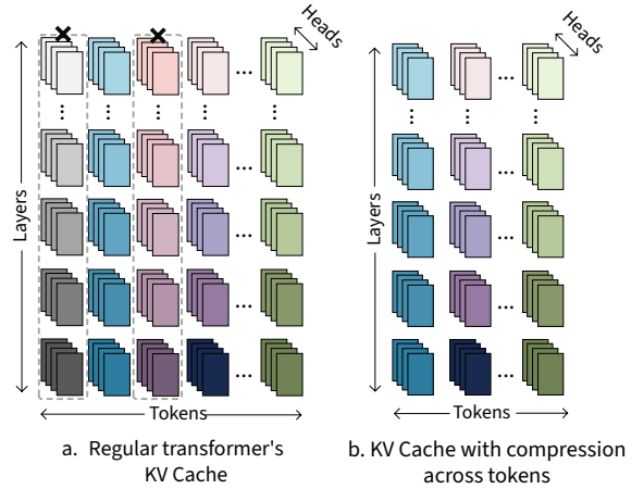
Figure 6. Illustration of KV Cache with token pruning and input compression techniques. These methods include pruning tokens or sentences or compressing the input context length using another language model, aiming to reduce computational load.
