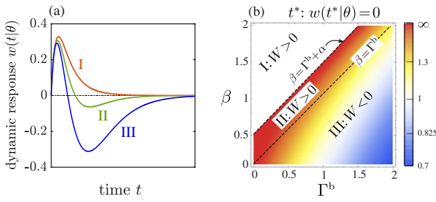
FIG. 2. (a) Three examples of time-dependent response w(t|\theta) associated with a single, isolated dopamine hit. We fix \theta = \{\Delta = 1, \alpha = 0.5, \Gamma^a = 1, \beta, \Gamma^b = 0.8\} and plot Eq. (4) for three different values of \beta showing a response that is always positive (I: \beta = 1.5 , orange), a response that can become negative (II: \beta = 0.9 , green), and one with a negative total reward (III: \beta = 0.45 , blue). (b) Density plot representing the values of the time t^* associated with the solution to the transcendental equation w(t^*|\theta) = 0 as a function of \beta and \Gamma^b for \alpha = 0.5 . The white parameter region does not admit a finite solution to t^* [ w(t|\theta) is always positive].
