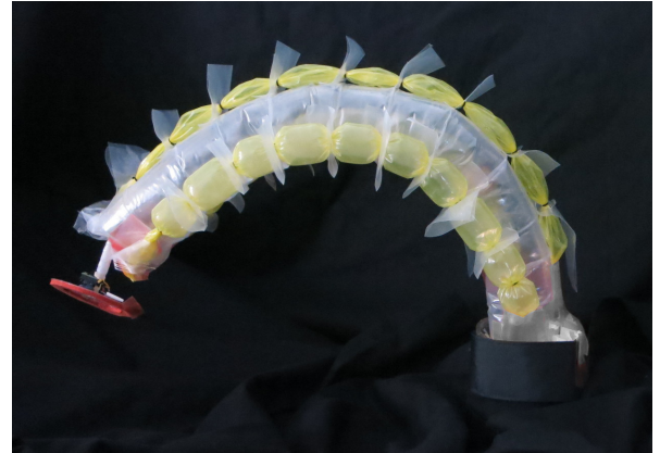
Fig. 1. Soft continuum robot with series pneumatic artificial muscles (sPAMs) attached.
