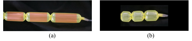
Fig. 5. (a) sPAM with o-ring spacing too large. Regions highlighted in red are where pleated PAM model predicts bulge radius larger than D_{\text{tube}} , and hence they do not contribute to contraction. (b) sPAM without inactive regions.
