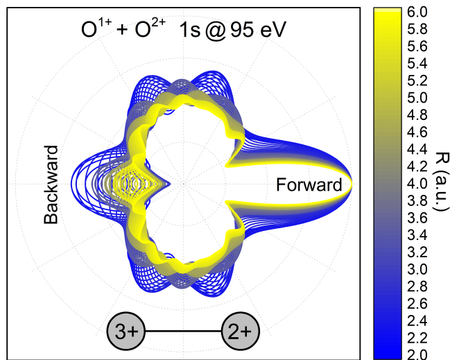
Fig. 2 Polarization-averaged MFPADs of the second 1s photoelectron, computed in the relaxed-core Hartree-Fock approximation at different internuclear separations for the \text{O}^{1+} + \text{O}^{2+} \rightarrow \text{O}^{3+} + \text{O}^{2+} channel. After the second photoionization and Auger decay, the left singly charged oxygen ion becomes triply charged. An electron energy of 95 eV was used in the calculations, as these electrons represent the high-energy part of the broad feature in Fig. 1(a). The PA-MFPADs are normalized to the forward peak. The color encodes the internuclear separation between the two oxygen ions at the instant of the photoionization.
