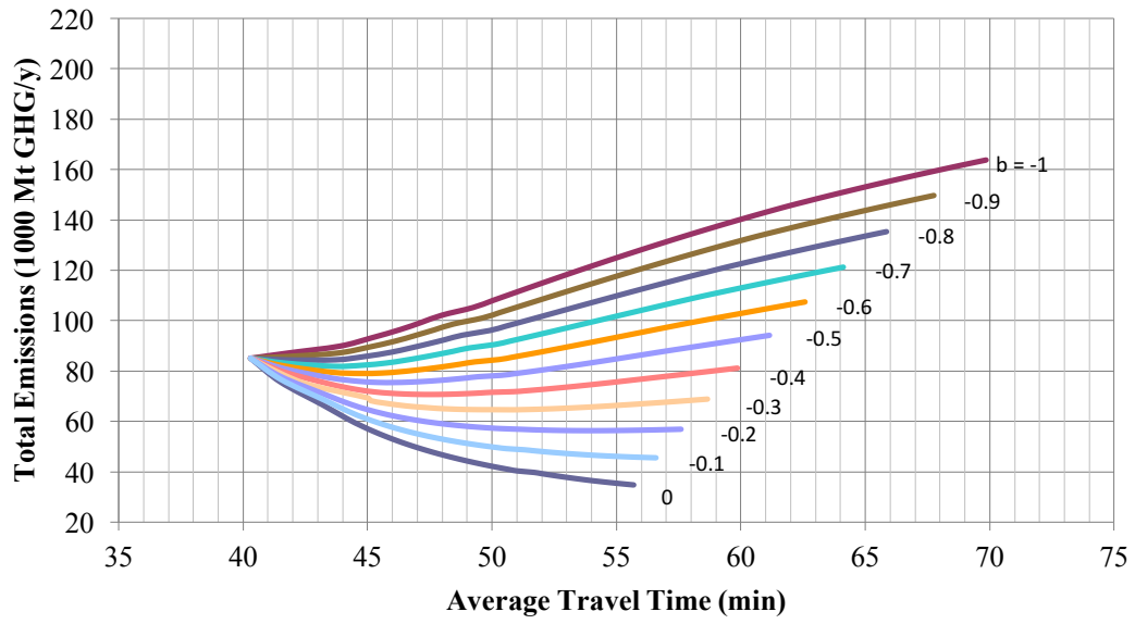
Figure 4.7 Change in total emissions with travel time as LOS is reduced for BRT (scenario 2)
