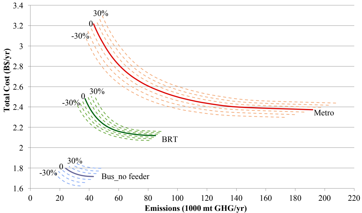
Figure 4.15 Sensitivity to changes in parameters for metro, BRT and trunk-only bus (scenario 2)
