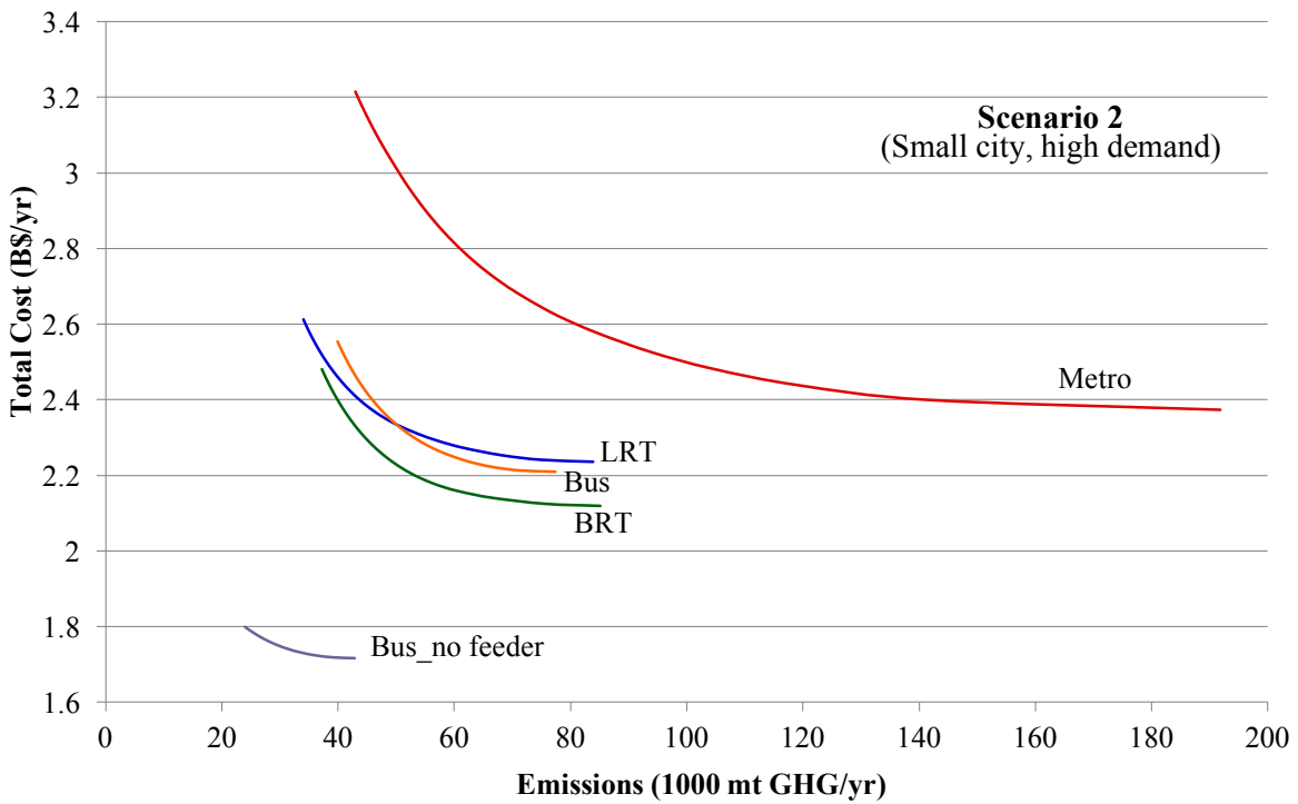
Figure 4.2 Technology-specific Pareto curves of system costs with varying transit emissions (scenario 2)
