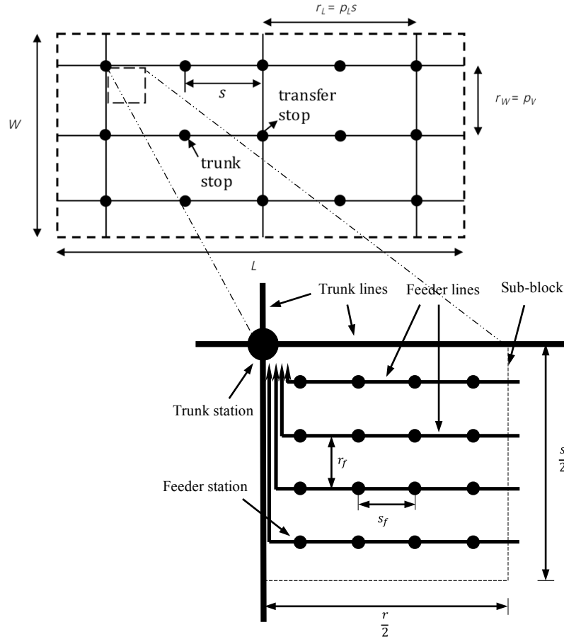
Figure 3.1 Hierarchical transit network for this study
