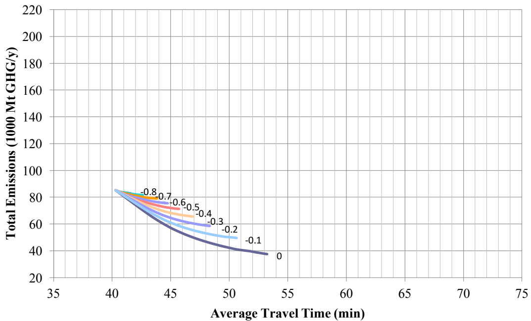
Figure 4.10 Change in total emissions as LOS is reduced for BRT under a city-wide emissions budget (scenario 2)
