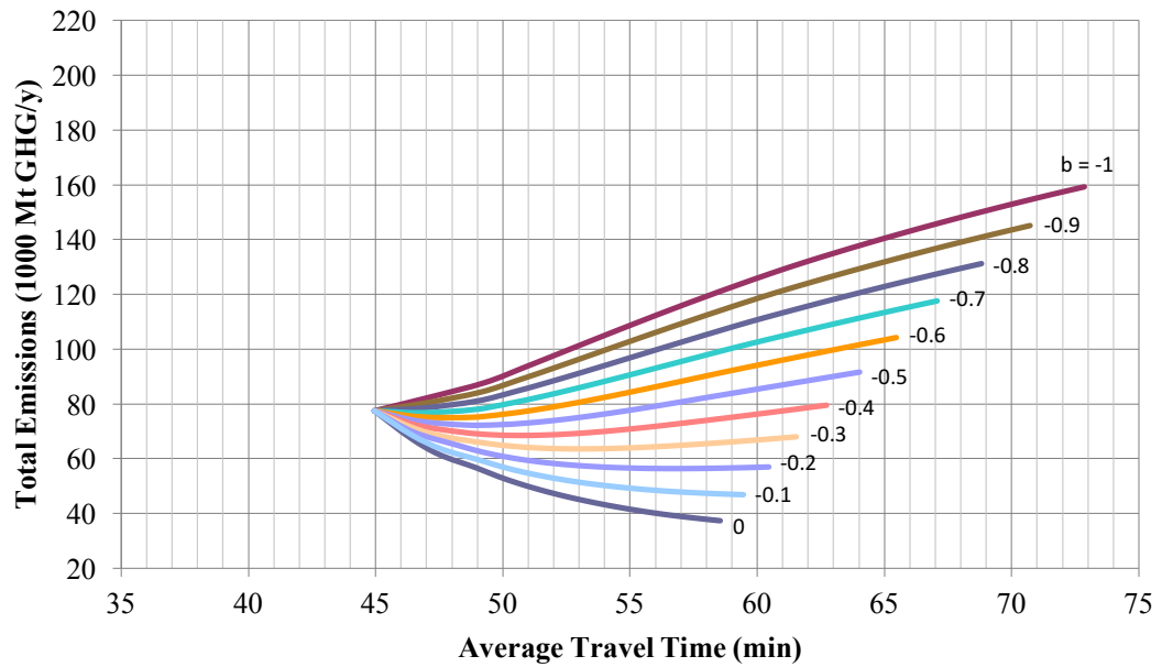
Figure 4.5 Change in total emissions with travel time as LOS is reduced for bus with no feeder access (scenario 2)
