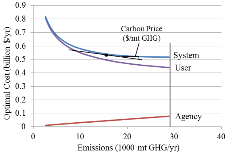
Figure 3.2 Total (system), user, and agency costs for a bus system by GHG emissions level (Griswold et al. 2013)
