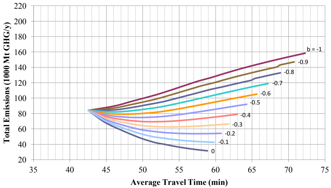
Figure 4.7 Change in total emissions with travel time as LOS is reduced for BRT (scenario 2)
