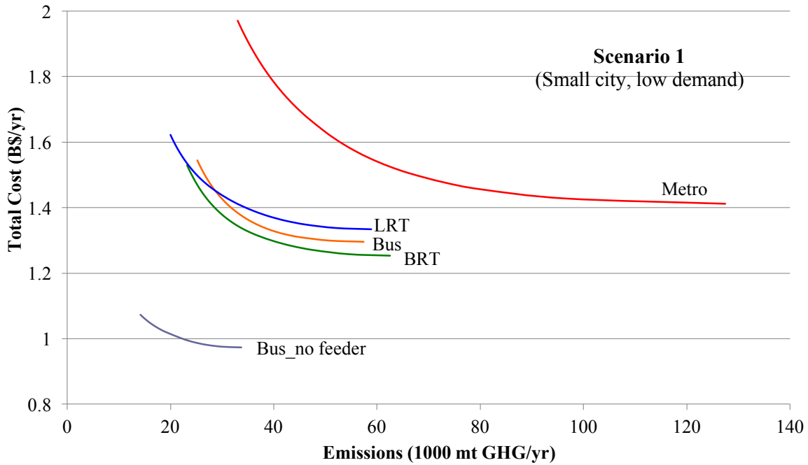
Figure 4.1 Technology-specific Pareto curves of system costs with varying transit emissions (scenario 1)
