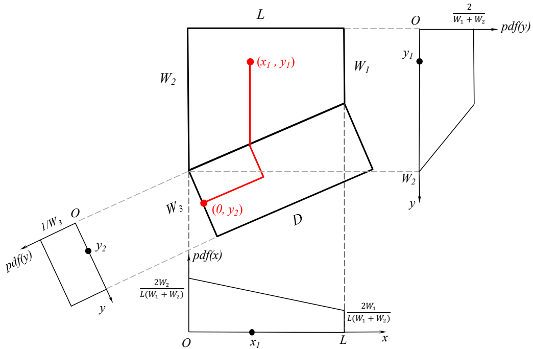
Figure 5.2 The Manhattan distance between two random dots in region S_1 and on edge W_3
