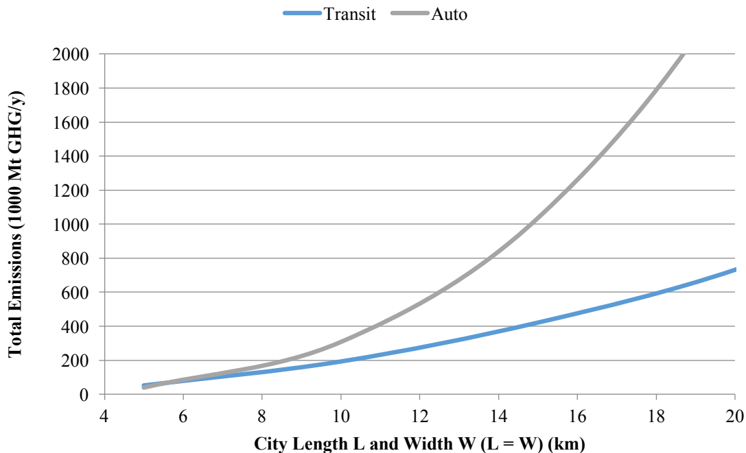
Figure 4.14 Total emissions of city with varying size
