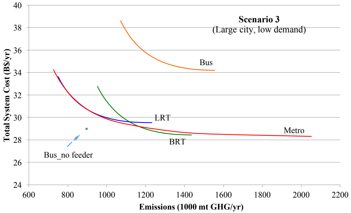
Figure 4.3 Technology-specific Pareto curves of system costs with varying transit emissions (scenario 3)
