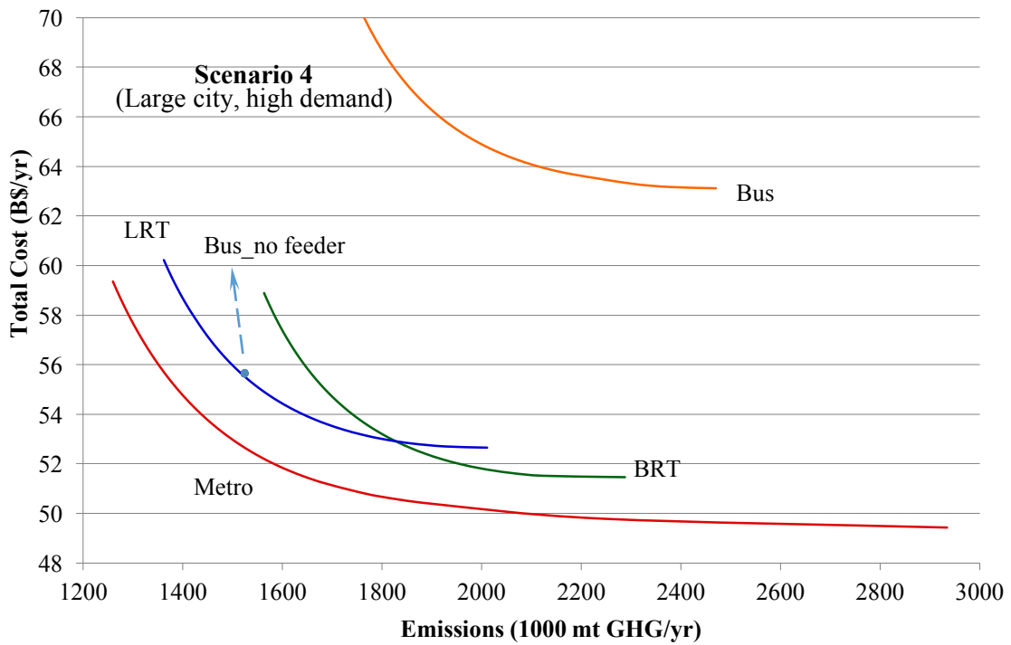
Figure 4.4 Technology-specific Pareto curves of system costs with varying transit emissions (scenario 4)
