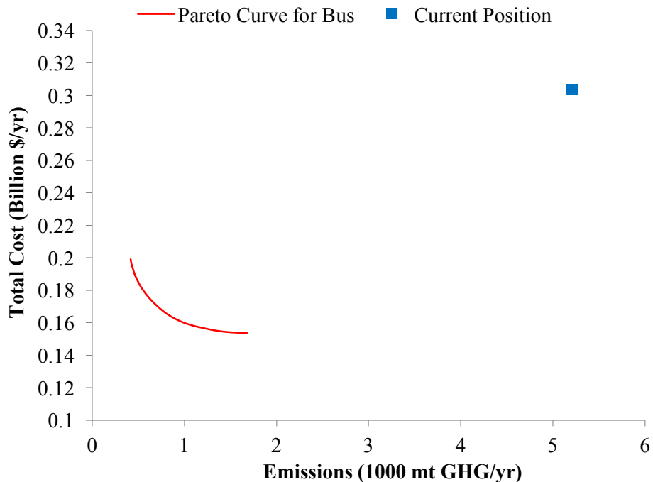
Figure 6.1 The current state of the MUNI network and the Pareto frontier
