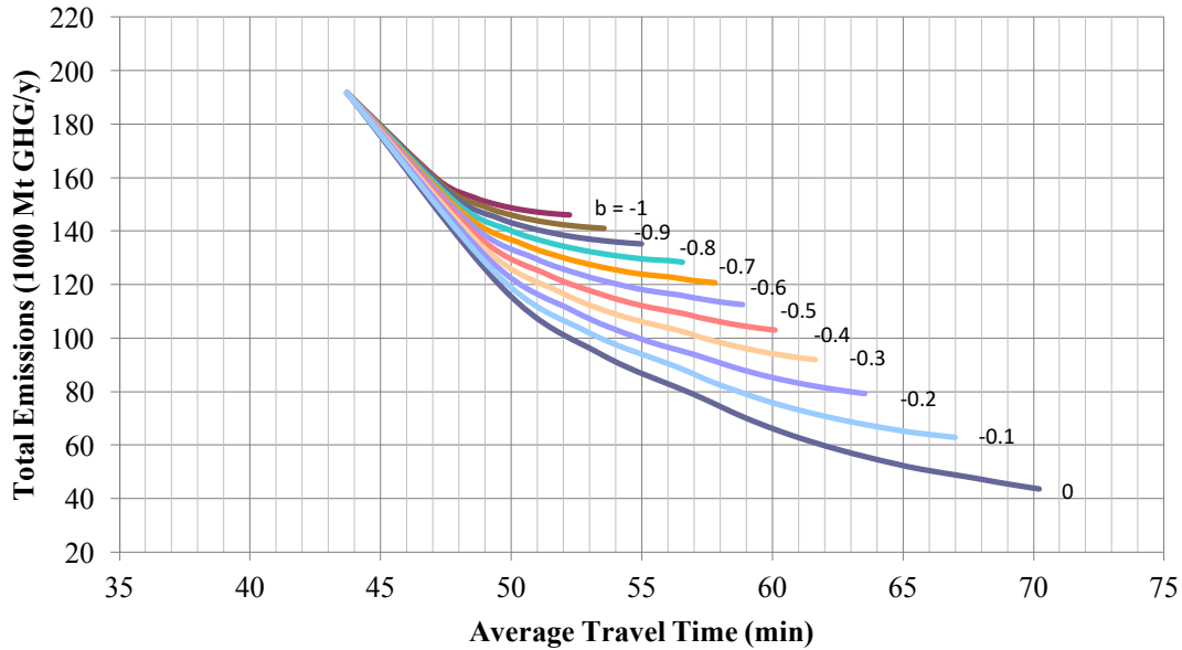
Figure 4.11 Change in total emissions as LOS is reduced for metro under a city-wide emissions budget (scenario 2)
