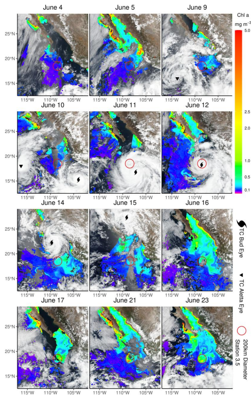
Ch 1 - Figure 2: Remotely sensed [Chl a] images ( \text{mg m}^{-3} ) prior to (June 4 th -10 th 2018), during (June 11 th -15 th ), and following (June 16 th -23 rd ) Hurricane Bud demonstrate the presence and influence of the tropical cyclone. [Chl a] values are shown on the color scale, with values above 5 \text{ mg m}^{-3} shown in red. Overlaid true-color imagery shows cloud cover, land cover, and areas with no available [Chl a] values. Eye position is shown for tropical cyclones Bud (storm symbol) and Aletta (triangle), and the red circle (200 km diameter) is centered on station 3.5. See text for dates and specific storm strength designation. Images are ca. local solar noon.
