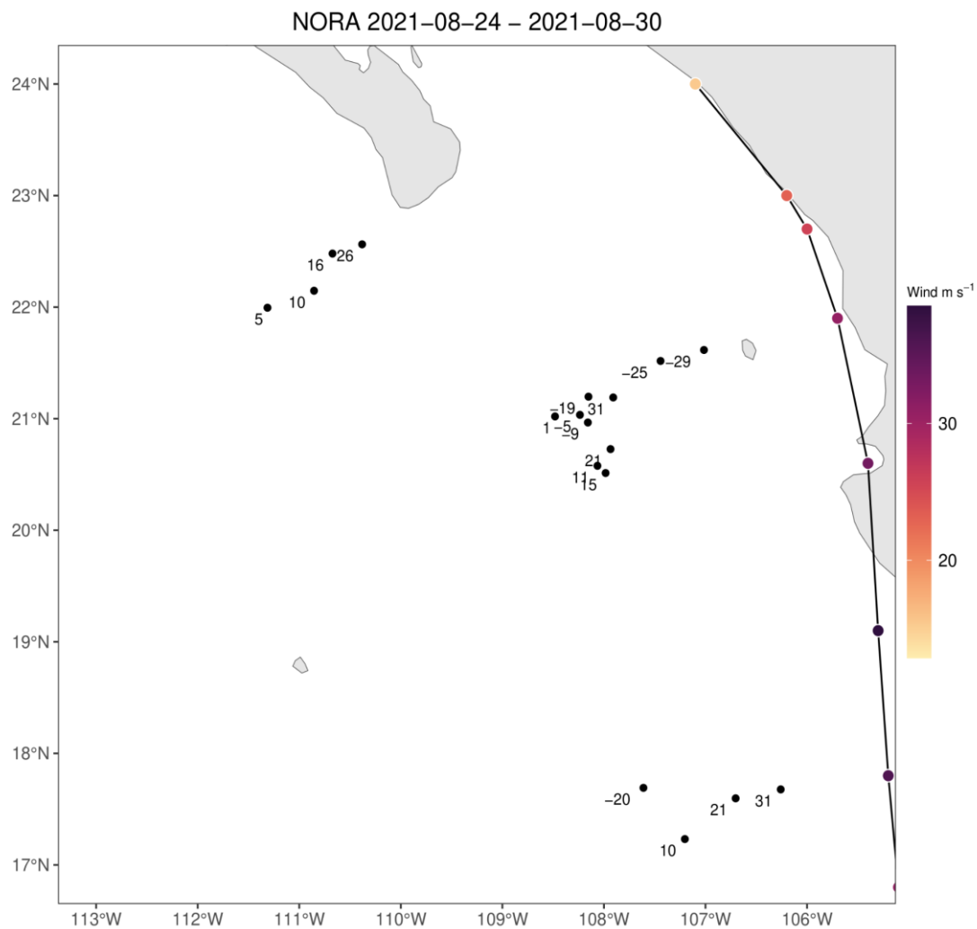
Ch 3 - Figure 6: Multiple floats and TC Nora .Dates in the title give the window of six hour eye position for Nora on the map. Three sets of dots are profiles for floats 6903094, 6903093, 5905068, from North to South, respectively. Positive and negative numbers are days after or before from closet overpass to the TC track for individual profiles. Scale is wind speed for TC at the six hour position.
