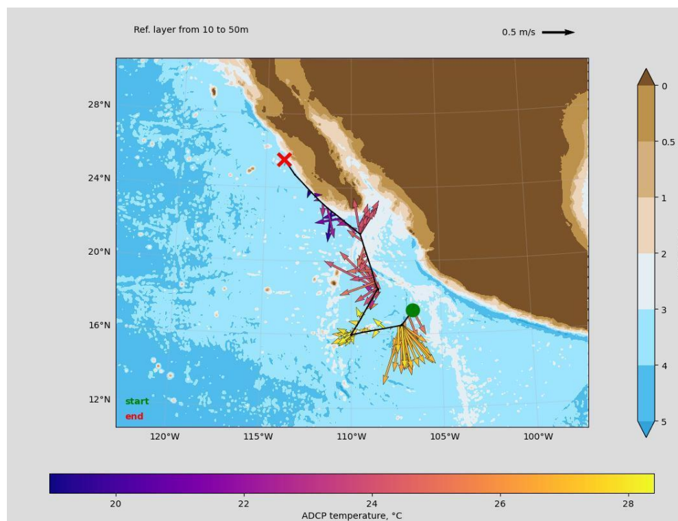
Ch 2 - Figure 1: Ocean current profiles from shipboard ADCP sensors. 2-hour averaged, depth integrated (10-50m) horizontal vector (m/s) components with colors indicating temperature using Wh300 hz bb surface ADCP. Track on map corresponds to the three panels in Figure 2.
