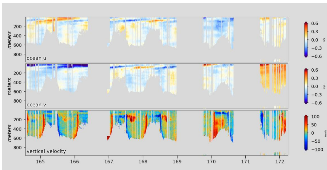
Ch 2 - Figure 2: Ocean current profiles from shipboard ADCP sensor. Corresponds to the cruise track in Figure 1. Top panel is zonal velocity, u , ( \text{m s}^{-1} ). Middle panel is meridional, v , “”. Bottom panel vertical velocity, w , ( \text{mm s}^{-1} ). Gray indicates no data, or data removed due to ship movement induced noise. Red is positive (East, North, Up). Blue is negative (West, South, Down). Left axis is depth to 1000m. Times in decimal yr-day UTC-0. Panels are velocity components from the 75 kHz near-band sensor.
