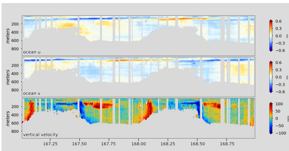
Ch 2 - Figure 17: Station 3 deep. Ocean current profiles from shipboard ADCP sensor over Station 3. Time window corresponds to vessel sampling at Station 3. Top panel zonal velocity, u , ( \text{m s}^{-1} ). Middle panel is meridional, v , “”. Bottom panel is vertical velocity, w , ( \text{mm s}^{-1} ). Gray indicates no data, or data removed due to ship movement induced noise. Red is positive (East, North, Up). Blue is negative (West, South, Down). Times in decimal yr-day (167.25 ~ 2018-06-17 06:02 UTC). Left axis is depth to 1000m. Panels are velocity components from the 75 kHz near-band sensor.
