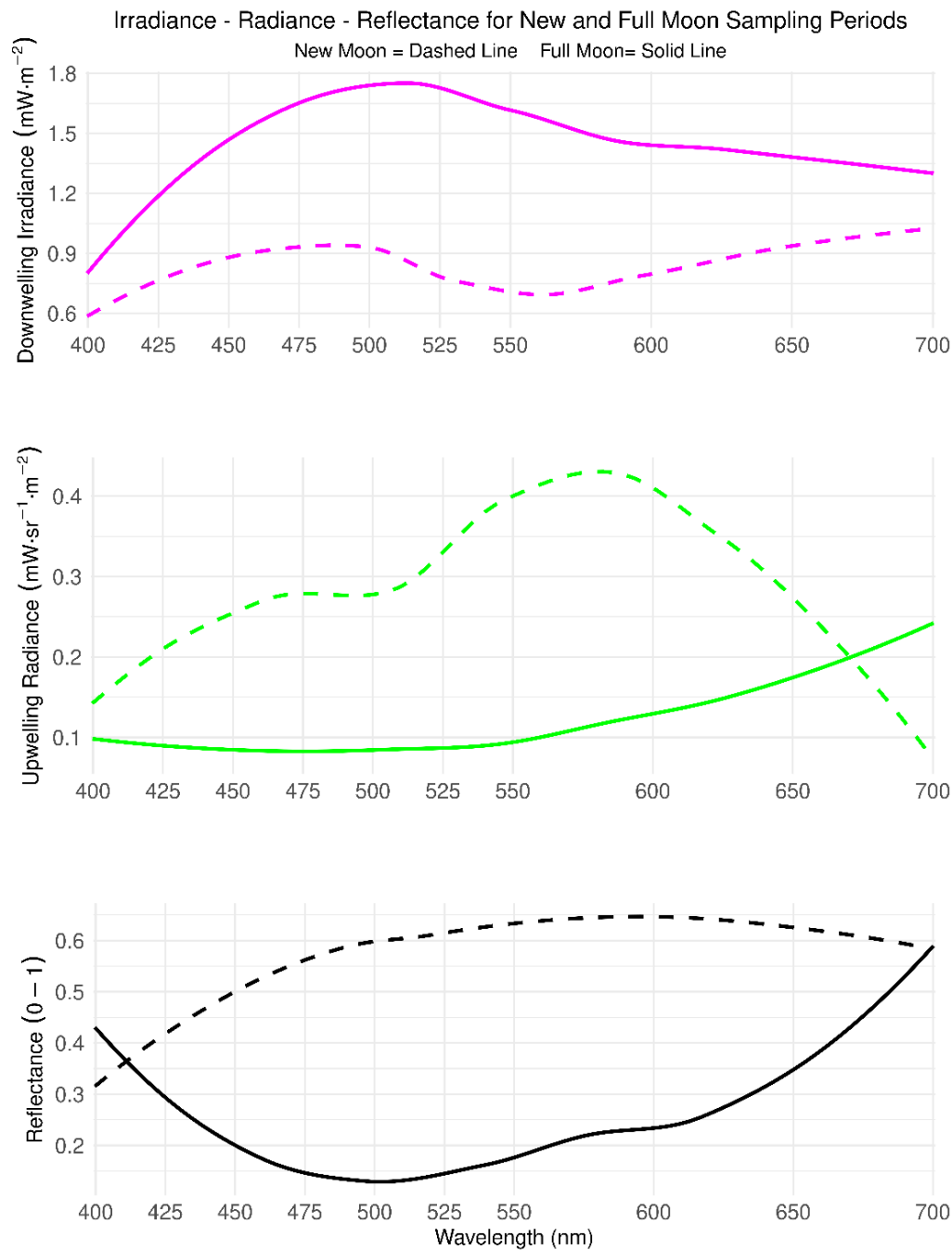
App. - Figure 3: Full moon indicated by solid lines, new moon dashed. Lines are mean for all sites per sampling night. Top panel is downwelling irradiance, incoming moonlight a meter above water (magenta). Middle panel is water leaving/upwelling radiance (green). Units differ. Bottom panel is reflectance (black), the ratio of upwelling energy to incoming energy ( \pi \cdot \text{radiance}/\text{irradiance} ). Does not take into account the
