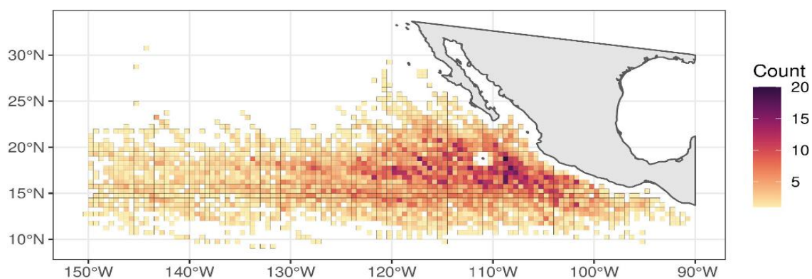
Ch 1 - Figure 5: Hurricane occurrence in the ENTP. Color scale shows hurricane eye observations per 0.5° x 0.5° cell from 1942 to 2021 in the NOAA HURDAT database. Hurricanes outside of the ETNP (~5-33°N, and 150-90°W) and within 200 km distance from land (including islands located off the Pacific coast of Mexico) were excluded.
