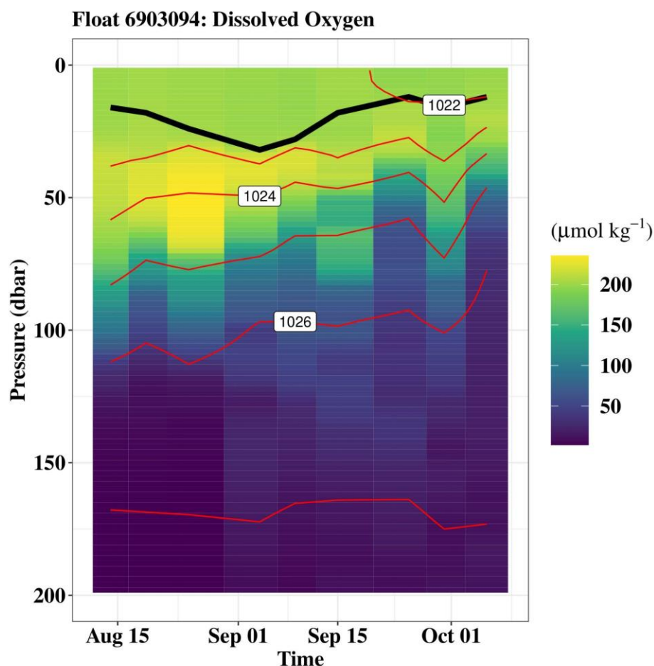
Ch 3 - Figure 12: Interpolated section of Float 6903094 for Olaf and Nora overpasses. Not the same float as preceding figures of profiles. For Olaf Passover date (09/10), was -1 and 5 days to the closet profiles. Black line is the mixed layer depth red lines are density isopycnals.
