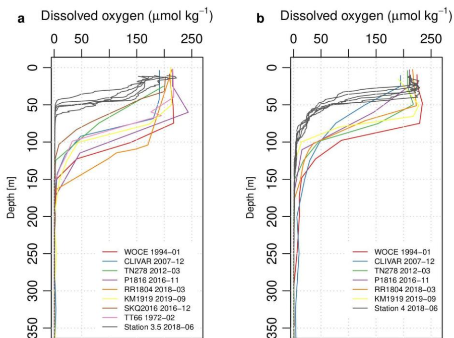
Ch 1 - Supplementary Figure 4: Dissolved oxygen profiles, CTDs from 2018 cruise with reference cruise measurements closest to (a) Station 3.5, and (b) Station 4. Reference cruises have course depth resolution. Colored lines indicate each cruise. Multiple profiles are shown for the 2018 cruise in gray. Dates listed for reference cruises indicate the start month of the cruise.
