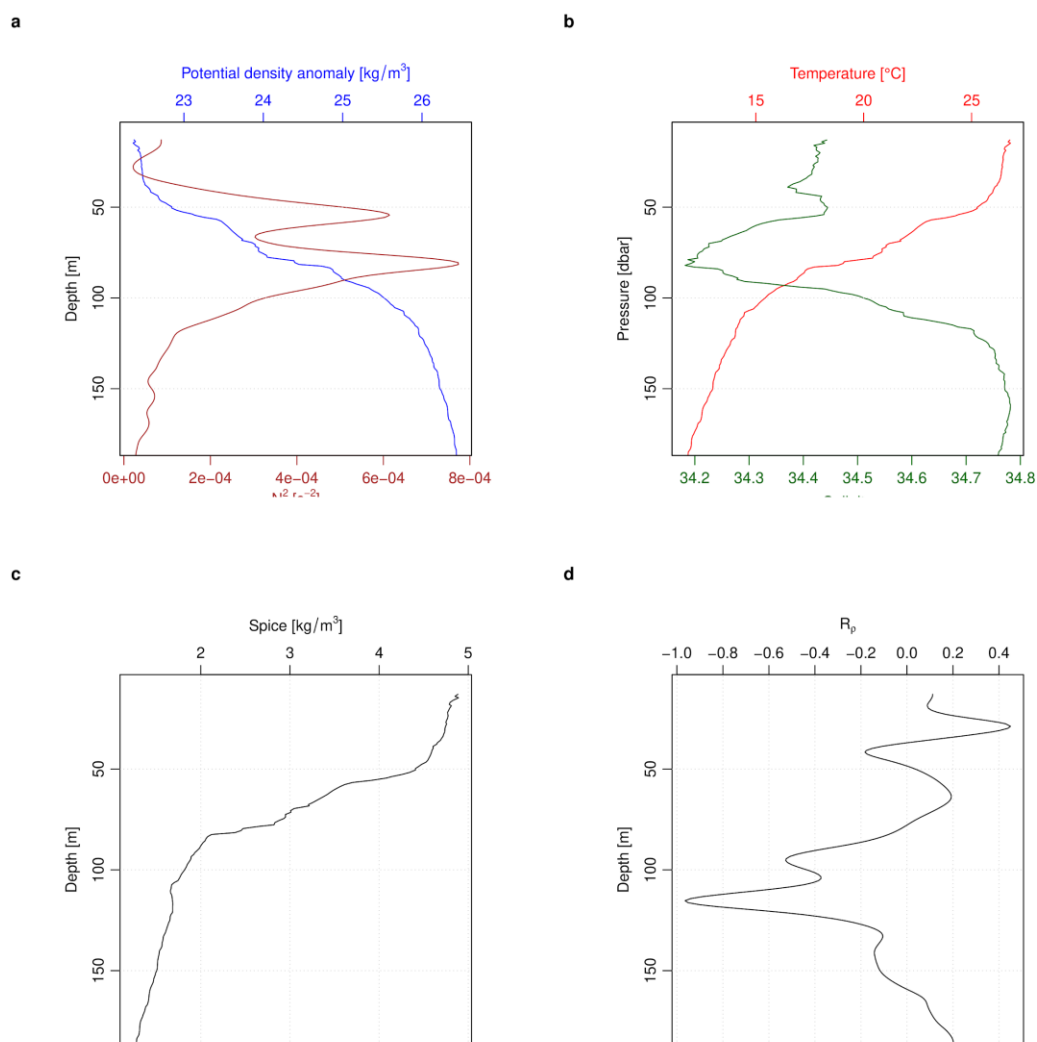
Ch 2 - Figure 21: Station 3 descriptive oceanographic CTD profiles for the sixth cast, 18 - 01:01 UTC-0. (a) potential density anomaly \Sigma\text{-}0 [ \text{kg}/\text{m}^3 ] top x-axis in blue, with the square of the buoyancy frequency in brown [ \text{N}^2[\text{s}^{-2}] ], bottom x-axis. (b) Temperature in Celsius in the red top x-axis, Salinity in PSUs in green bottom x-axis. (c) Spice, ratio of (warm + salty)/ (cold+fresh) of water mass [ \text{kg}/\text{m}^3 ]. (d) R_\rho = change in f^\circ of salinity/temperature over depth as described in methods. Diffusivity implementation.
