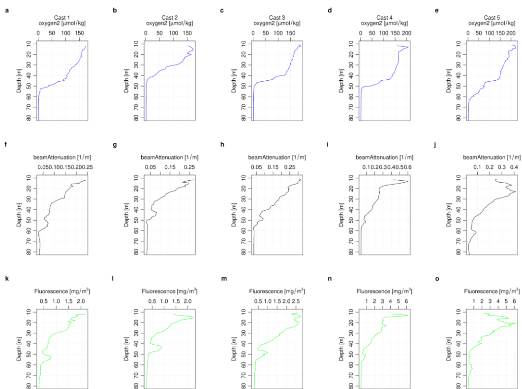
Ch 2 - Figure 9: Station 3.5 CTD profiles by depth. Each column is an individual cast plotted in sequential order corresponding to Table 1 (e.g., cast 1 {a,f,k}). (a-e) oxygen [ \mu\text{mol/kg} ], (f-j) beam attenuation [ 1/\text{m} ], (k-o) fluorescence [ \text{mg}/\text{m}^3 ]. The y-axis is increasing depth in meters.
