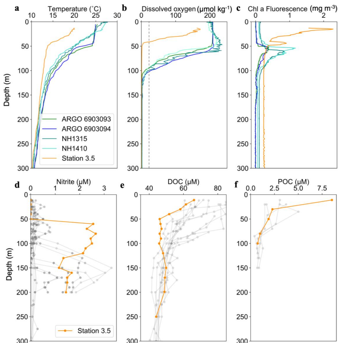
Ch 1 - Figure 4: Post-hurricane profiles from Station 3.5 show substantial differences with data from other cruises, floats, and stations in (a) temperature, (b) dissolved oxygen concentrations, (c) chlorophyll, (d) nitrite concentrations, (e) DOC, and (f) particulate organic carbon (POC) concentrations. In panels a-c, Station 3.5 data (orange) are shown in comparison to earlier cruises and recent float data (blue and green profiles) collected nearby (see text). In panels d-f, Station 3.5 data (orange) show distinct patterns in comparison to all other data collected on our cruises (gray). The dashed line in panel c indicates 20 \mu\text{M} DO.
