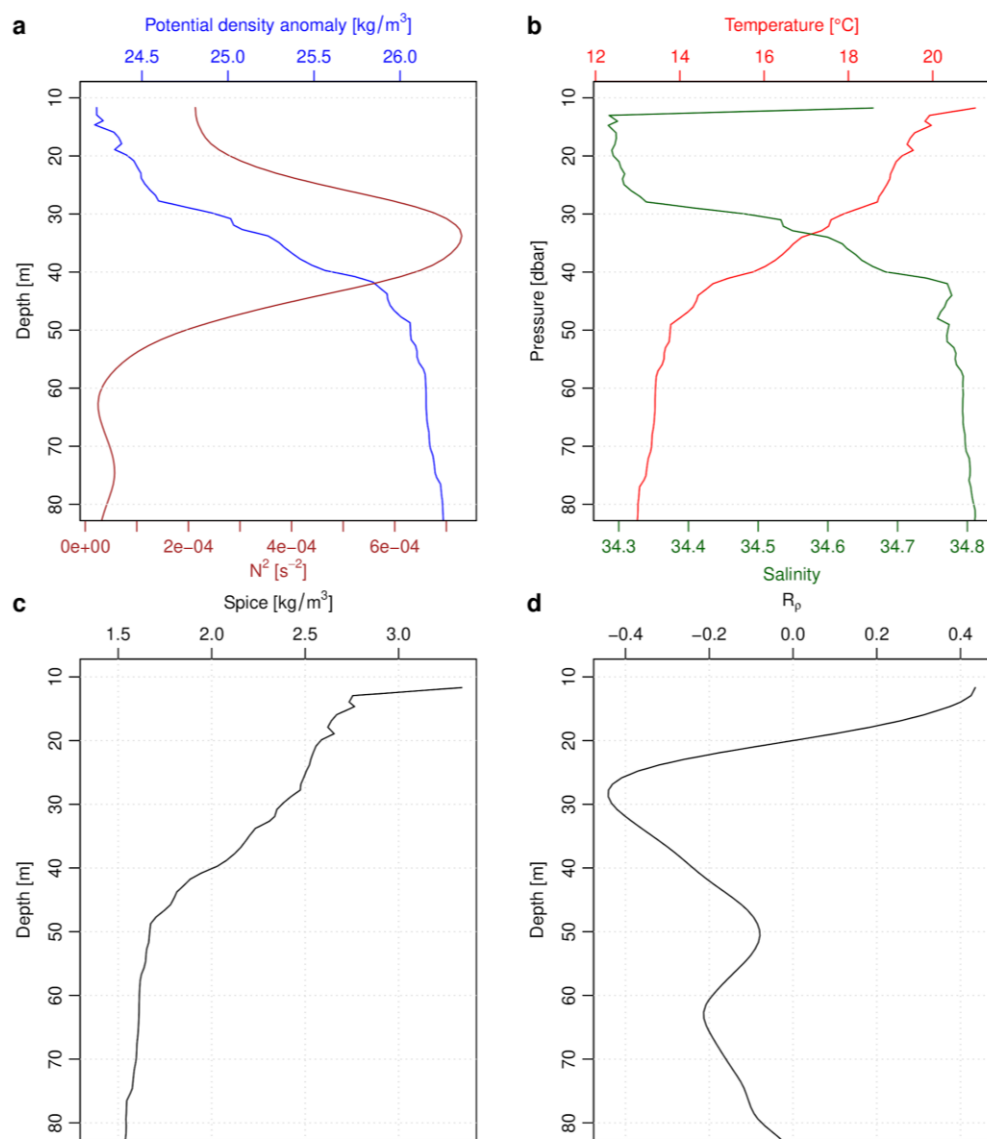
Ch 2 - Figure 8: Station 3.5 descriptive oceanographic CTD profiles for the second cast, 19 - 21:04 UTC-0. (a) potential density anomaly \Sigma\text{-}0 [ \text{kg}/\text{m}^3 ] top x-axis in blue, with the square of the buoyancy frequency in brown [ \text{N}^2[\text{s}^{-2}] ], bottom x-axis. (b) Temperature in Celsius in red top x-axis, Salinity in PSUs in green bottom x-axis. (c) Spice, ratio of (warm + salty)/ (cold+fresh) of water mass [ \text{kg}/\text{m}^3 ]. (d) R_\rho = change in f' of salinity/temperature over depth as described in methods. Diffusivity implementation.
