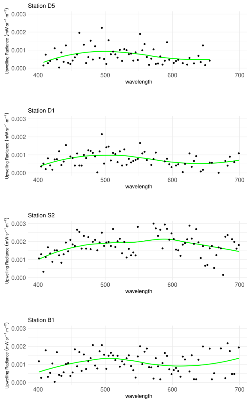
App. - Figure 4: Integrated nighttime subsurface radiometric profiles, upwelling radiance - downward facing probe, for June 2019 full moon sampling. Trends are means for integrated values (points) for 0-5m for all profiles per station. Y-axis is intensity, x axis is wavelength. From top panel:: Station D5, D1, S2, B1 (see Figure 1).
