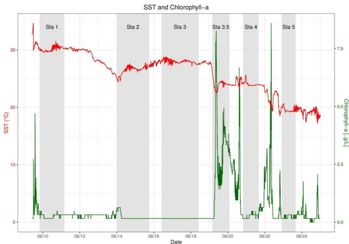
Ch 1 - Supplementary Figure 1: Continuous flowthrough data of Sea Surface Temperature (SST; red line) and chlorophyll- a concentration (in \mu\text{g/L} ; green line) from the 2018 R/V Oceanus cruise. Chlorophyll increases coincide with decreases in SST near stations 2, 3.5, and 4 in wake of Hurricane Bud. Gray bars denote periods on station when water profile measurements and biogeochemical casts were collected (see Figures 1 & 3). Date/times are local (MDT/UTC-6). Data are available on the R2R repository 4 .
