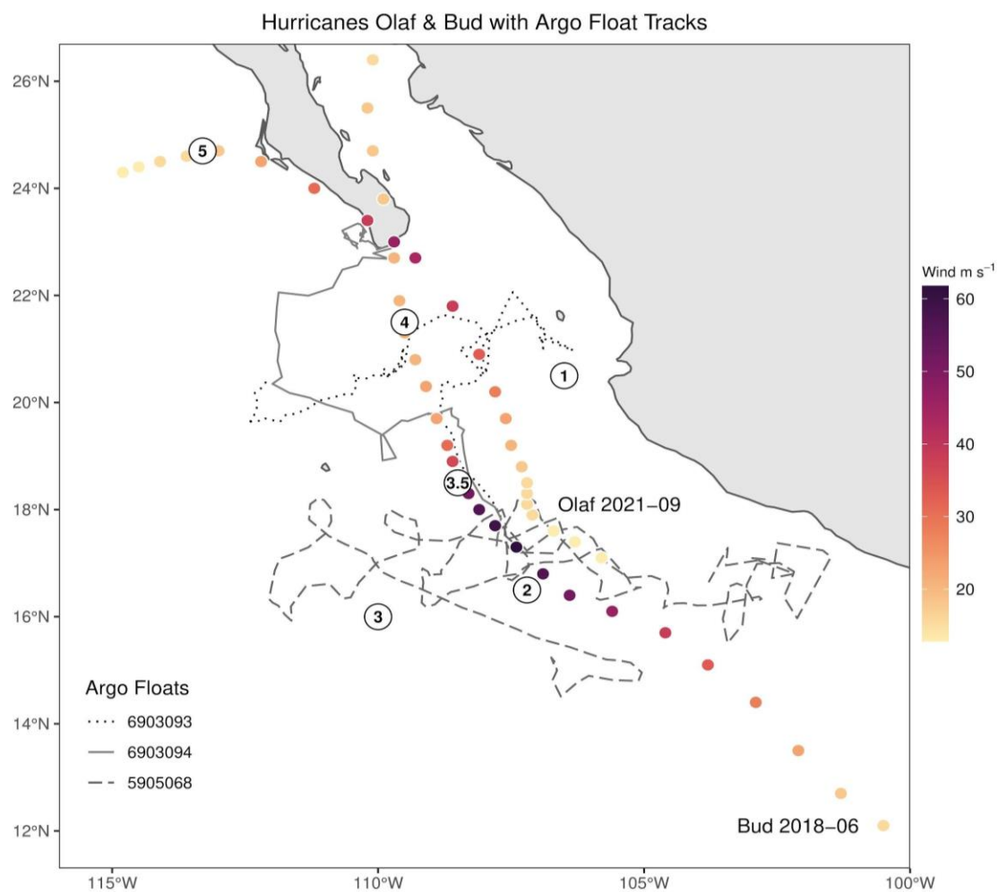
Ch 3 - Figure 2: Spatial overlay of Hurricanes Bud (Ch1 & 2), with cruise sampling stations (numbered circles), as well as Hurricane Olaf. Three different dashed lines are tracks of associated BGC-Argo floats with identifier numbers. Floats 6903093 and 6903094 were used for reference data for Station 3.5 (Ch 1 Fig. 4a). Color-shaded dots show maximum sustained wind speeds every six hours along Hurricane Olaf's track.
