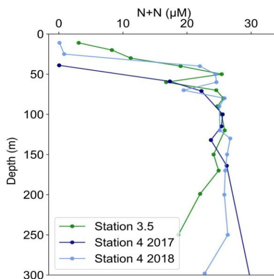
Ch 1 - Supplementary Figure 3: Water column profiles of combined nitrate + nitrite concentrations at Station 3.5 (green; 2018 only) and Station 4 (blue; 2017 and 2018). For Station 4, 2017 data are shown in dark blue, and 2018 data collected following the hurricane are shown in light blue.
