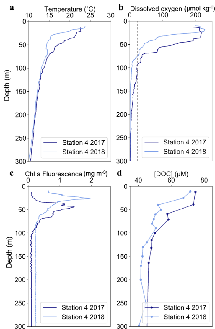
Ch 1 - Figure 3: Water column profiles at Station 4 demonstrate hurricane-driven shifts in (a) temperature, (b) dissolved oxygen, (c) chlorophyll, and (d) dissolved organic carbon (DOC) concentrations between 2017 (dark blue profiles) and 2018 (light blue profiles). The dashed line in panel b indicates 20 \mu\text{M} DO.
