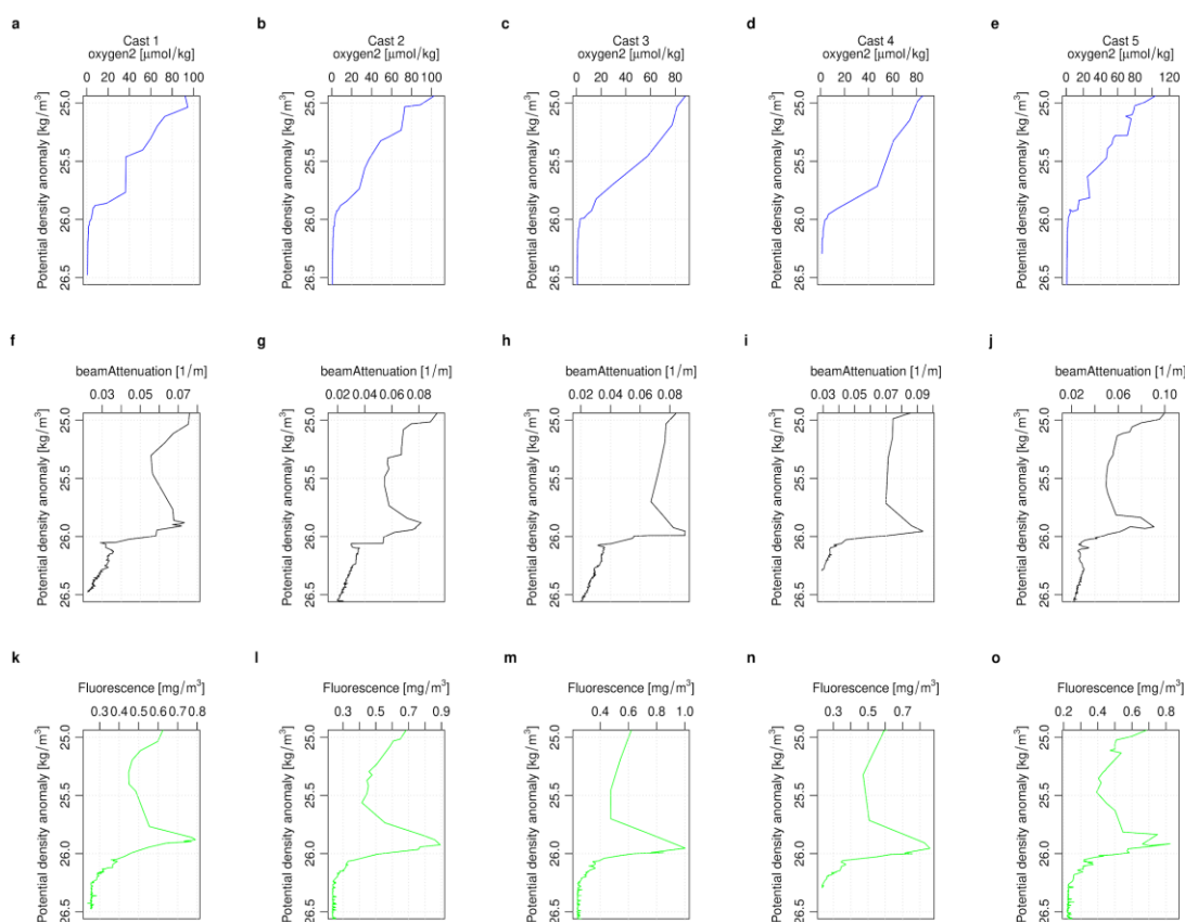
Ch 2 - Figure 10: Station 3.5 CTD profiles by isopycnal surfaces. Each column is a unique cast plotted in sequential order corresponding to Table 1 (e.g., cast 1 {a,f,k}). (a-e) oxygen [ \mu\text{mol/kg} ], (f-j) beam attenuation [ 1/\text{m} ], (k-o) fluorescence [ \text{mg}/\text{m}^3 ]. y-axis being Sigma-0 , potential density anomaly [ \text{kg}/\text{m}^3 ], as opposed to depth.
