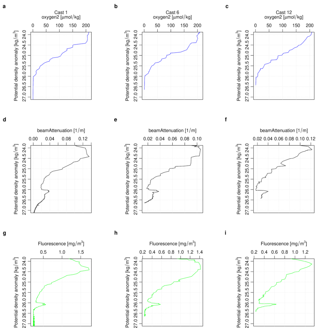
Ch 2 - Figure 20: Station 3 CTD profiles by isopycnal surfaces. Each column is a unique cast plotted in sequential order corresponding to Table 2. Casts were chosen to be ~ 24 hours apart. (e.g., cast 1 {a,d,g}). (a-c) oxygen [μmol/kg], (d-f) beam attenuation [1/m], (g-i) fluorescence [mg/m 3 ]. y-axis being Sigma-0 , potential density anomaly [kg/m 3 ], as opposed to depth.
