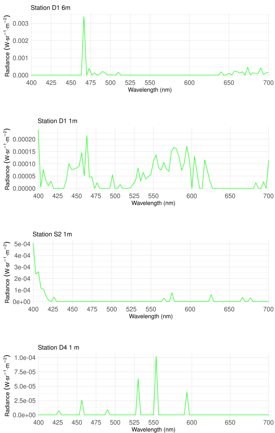
App. - Figure 5: Single nighttime subsurface radiometric profiles, upwelling radiance - downward facing probe, for June 2019 full moon sampling. Y-axis is intensity, x axis is wavelength. Panels are specific depths at three stations. From top panel: Station D1 6m, Station D1 1m, Station S2 1m, Station D4 1m.
