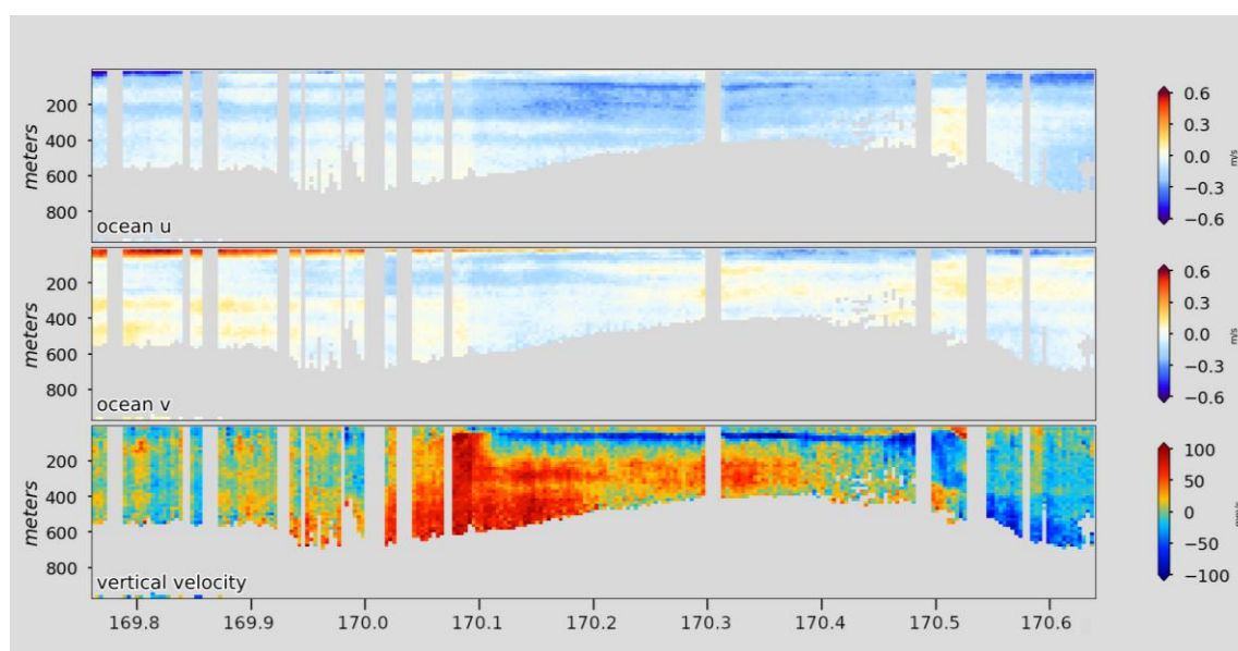
Ch 2 - Figure 4: Station 3.5 deep. Ocean current profiles from shipboard ADCP sensor over station 3.5. Time window corresponds to vessel sampling at Station 3.5. Top panel is zonal velocity, u , ( \text{m s}^{-1} ). Middle panel is meridional, v , “”. Bottom panel is vertical velocity, w , ( \text{mm s}^{-1} ). Gray indicates no data, or data removed due to ship movement induced noise. Red is positive (East, North, Up). Blue is negative (West, South, Down). Times in decimal yr-day (169.80 ~ 2018-06-19 19:13 UTC-0). Left axis is depth to 1000m. Panels are velocity components from the 75 kHz near-band sensor.
