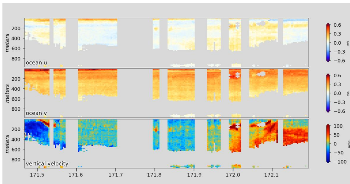
Ch 2 - Figure 12: Station 4 deep. Ocean current profiles from shipboard ADCP sensor over Station 4. Time window corresponds to vessel sampling at Station 4. Top panel zonal velocity, u , ( \text{m s}^{-1} ). Middle panel is meridional, v , “”. Bottom panel is vertical velocity, w , ( \text{mm s}^{-1} ). Gray indicates no data, or data removed due to ship movement induced noise. Red is positive (East, North, Up). Blue is negative (West, South, Down). Times in decimal yr-day (171.5 ~ 2018-06-21 11:59 UTC-0). Left axis is depth to 1000m. Panels are velocity components from the 75 kHz near-band sensor.
