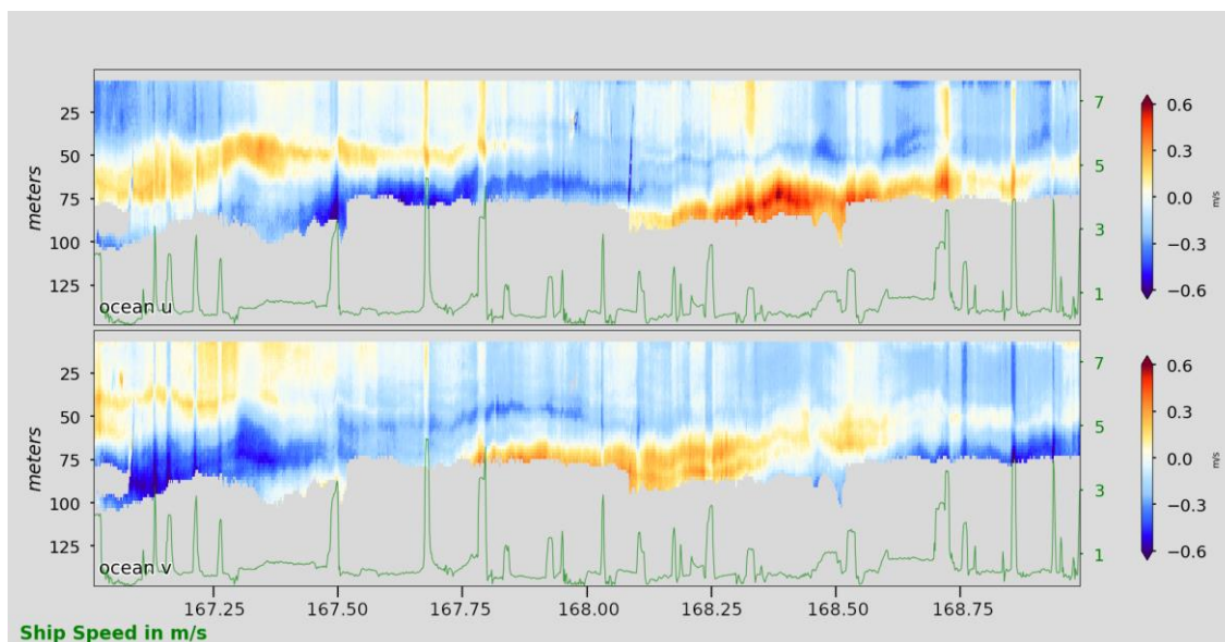
Ch 2 - Figure 16: Station 3 surface ADCP. Ocean current profiles from shipboard ADCP surface sensor over station 3. Time window corresponds to vessel sampling at Station 3. Top panel is zonal velocity, u , ( \text{m s}^{-1} ). Bottom panel is meridional, v , “”. Red is positive (East, North). Blue is negative (West, South). Times in decimal yr-day (167.25 ~ 2018-06-17 06:02 UTC-0). Green overlay/right axis is ship velocity ( \text{m s}^{-1} ). Left axis is depth to 150m. Panels are velocity components from the 300 kHz sensor.
