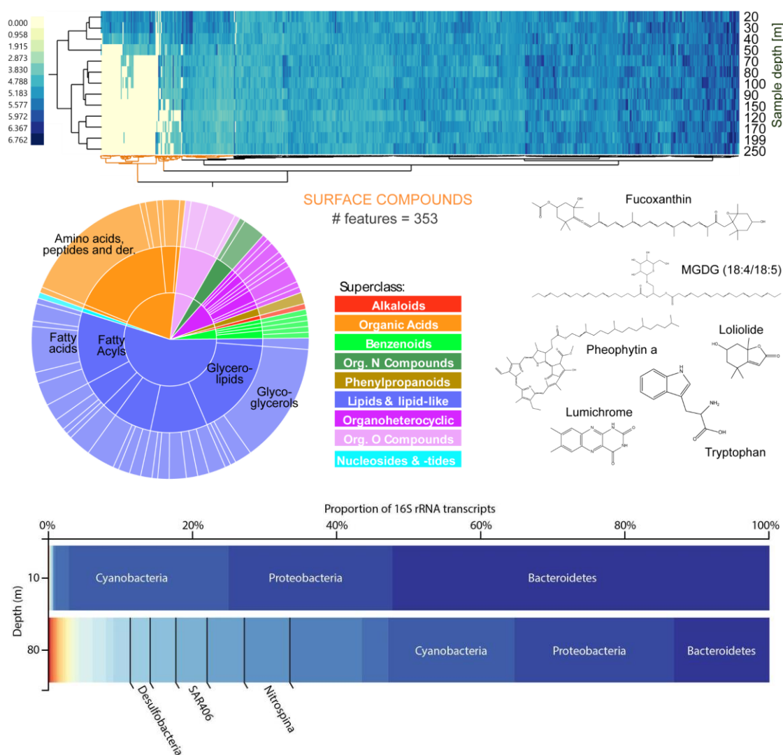
Ch 1 - Figure 6: Organic matter and microbial communities show unique compositions and variations at Station 3.5. The heatmap displays the relative abundance (color scale at left) of molecular features at different sampling depths (right axis). Two way hierarchical clustering of abundant molecular features is shown at the bottom of the heatmap, with clusters of features unique to or enriched in surface samples highlighted in orange (n=353). ‘Sunburst’ plot at left displays the chemical composition of the surface-enriched or -unique features at the Superclass, Class, and Subclass (progressing from innermost to outermost circle). Chemical structures of key surface-enriched or -unique features are shown at right. 16S rRNA data show active microbial groups at 10 m and 80 m depth at Station 3.5, with key microbial phyla indicated.
