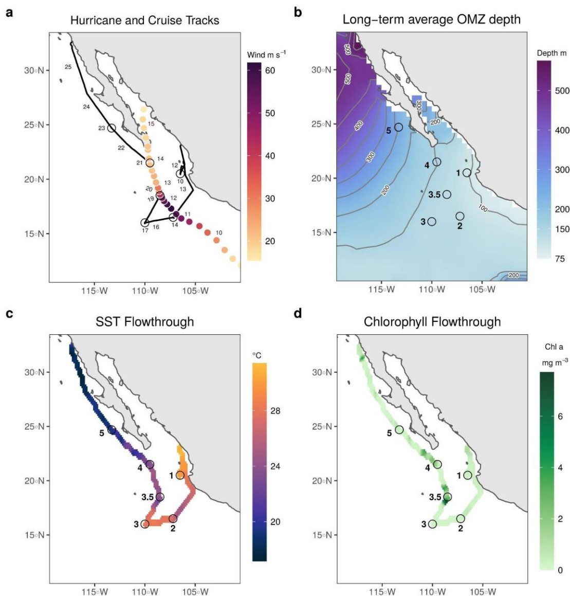
Ch 1 - Figure 1: Maps of (a) hurricane and cruise tracks, (b) long-term average OMZ depth, and shipboard flowthrough (c) SST and (d) chlorophyll in the ETNP. In panel (a), color-shaded dots show maximum sustained wind speeds 22 every six hours along Hurricane Bud's track, with the daily hurricane eye position during June 2018 labeled by purple numbers. The black line with dates in June 2018 (black numbers ranging from June 10-25) shows the cruise track. Panel (b) displays the long-term average depth of the OMZ (defined by 20 \mu M DO) based on the World Ocean Atlas climatology 23 . OMZ depth is indicated by 50 m contours and shading. Ship-board flowthrough (c) SST and (d) chlorophyll-a concentrations are shown by color shading. In panels b, c, and d, black circles with numbers indicate sampling stations.
