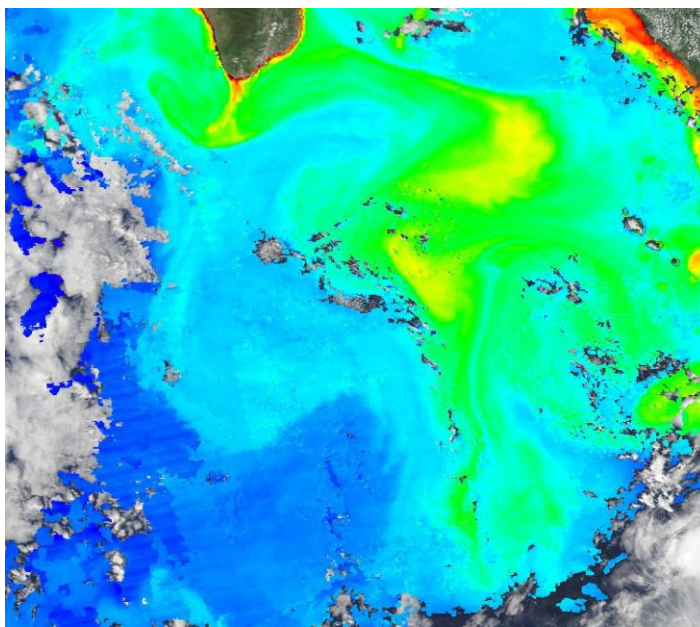
Ch 3 - Figure 4: Chl-a map on 2023-09-12. Olaf overpass. Multiple sensors for composite image (see Ch-1 Fig 2, and methods Ch-1) image from https://worldview.earthdata.nasa.gov
