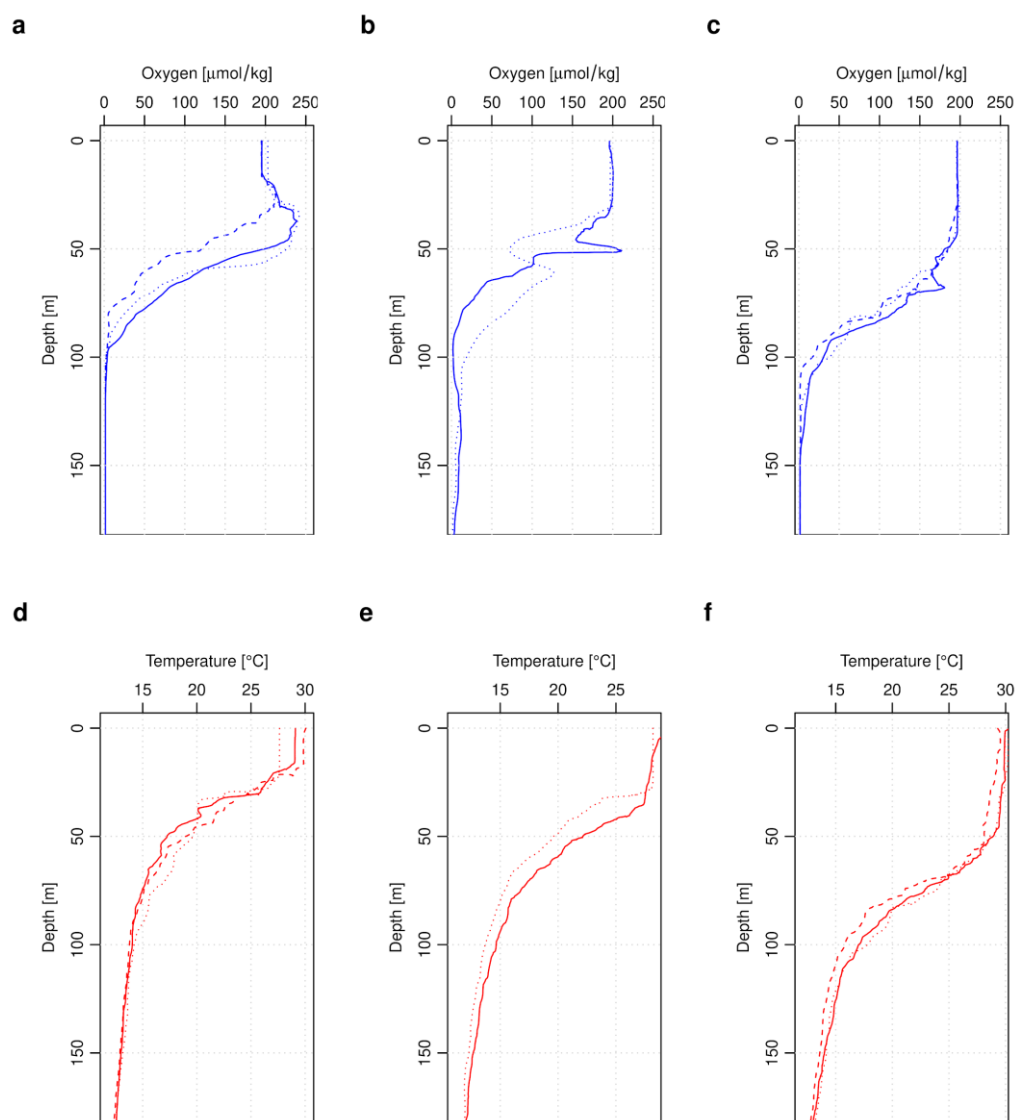
Ch 3 - Figure 7: Profiles of oxygen [ \mu\text{mol/kg} ] (a:c), and temperature in Celsius (d:f) for float 6903093 under Olaf. Three columns (a,d; b,e; c,f), are profile groupings: prior, immediately following, and post disturbance, following sequential order corresponding time relative to TC overpass. Lines in each panel are dashed, dotted, solid in sequential order, within groupings. Days relative are: -20, -16, -10, 0, 4, 10, 20, 24.
