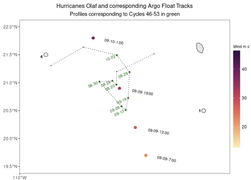
Ch 3 - Figure 3: Float 6903093 track under Olaf. Dates for before, during and after profiles used in following figures. Float track and dates in green. Six hour position of Hurricane Olaf with corresponding winds speeds, date and times in black. UTC-0. color-shaded dots show maximum sustained wind speeds every six hours along Hurricane Olaf's track.
