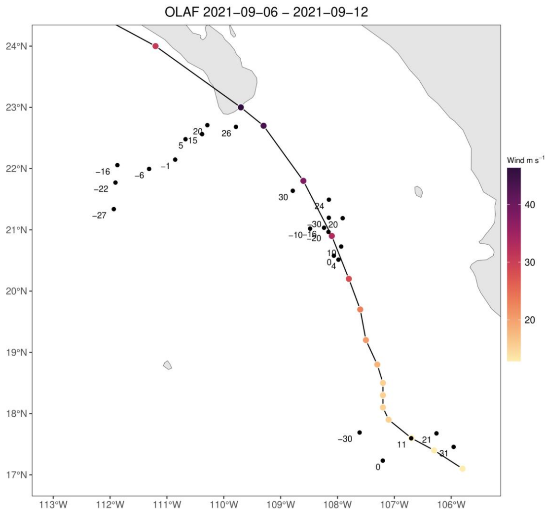
Ch 3 - Figure 5: Multiple floats and TC Olaf. Dates in the title give the window of six hour eye position for Olaf on the map. Three sets of dots are profiles for floats 6903094, 6903093, 5905068, from North to South, respectively. Positive and negative numbers are days after or before from closet overpass to the TC track for individual profiles. Scale is wind speed for TC at the six hour position.
