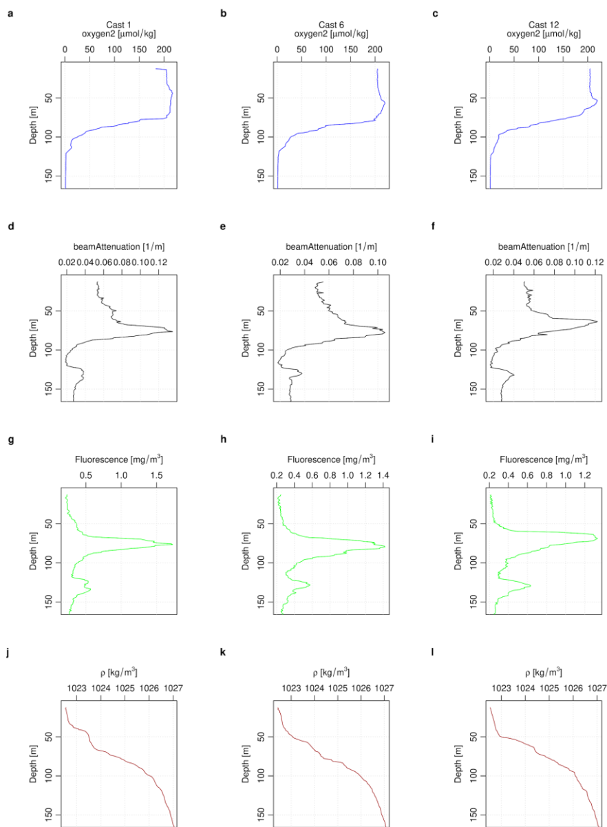
Ch 2 - Figure 19: Station 3. CTD profiles by depth. Each column is an individual cast plotted in sequential order corresponding to Table 2, casts were chosen to be ~ 24 hours apart. (e.g., cast 1 {a,d,g,j}). (a-c) oxygen [ \mu\text{mol}/\text{kg} ], (d-f) beam attenuation [ 1/\text{m} ], (g-i) fluorescence [ \text{mg}/\text{m}^3 ], and (j-l) density as Sigma-theta [ \text{kg}/\text{m}^3 ]. The y-axis is increasing depth in meters.
