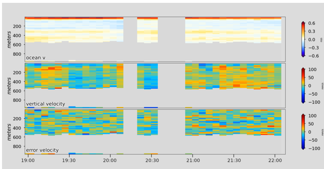
Ch 2 - Figure 22: ADCP station 3.5 deep, casts 1 & 2. Ocean current profiles from shipboard ADCP sensor over station 3.5. Time window corresponds to CTD casts 1 and 2 (Table 1). Top panel is meridional velocity, v , ( \text{m s}^{-1} ). Middle panel is vertical velocity, w , ( \text{mm s}^{-1} ). Bottom panel is error velocity in the vertical velocity panel. Gray indicates no data, or data removed due to ship movement induced noise. Red is positive (North, Up). Blue is negative (South, Down). Times in UTC-0 for 06-19. Left axis is depth to 1000m. Panels are velocity components from the 75 kHz near-band sensor.
