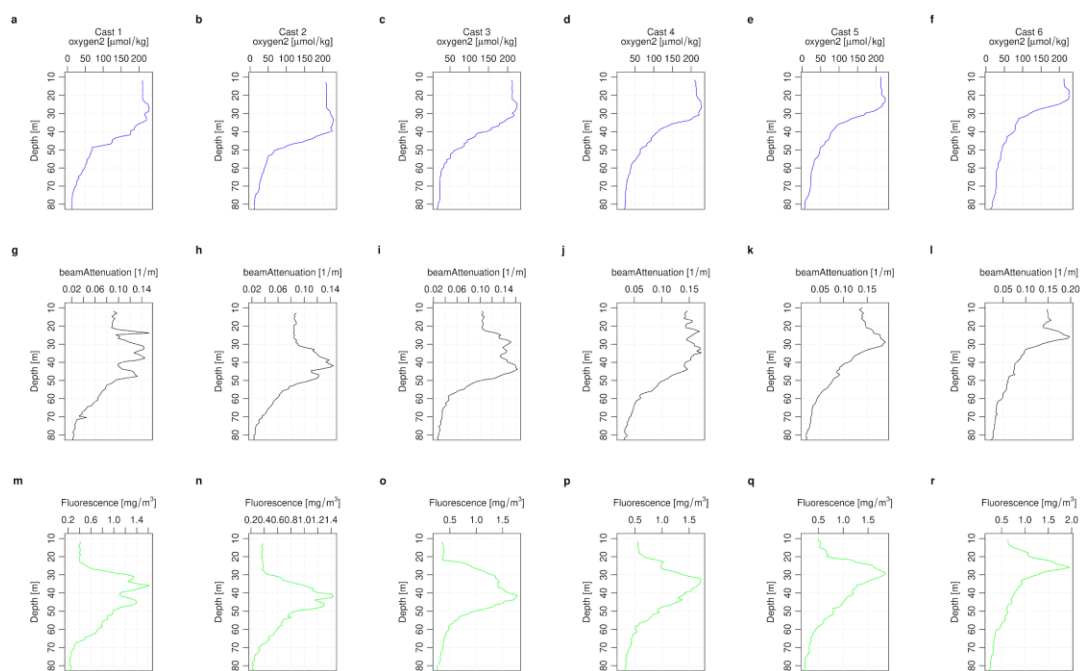
Ch 2 - Figure 14: Station 4 CTD profiles by depth. Each column is an individual cast plotted in sequential order corresponding to Table 2 (e.g., cast 1 {a,g,m}). (a-f) oxygen [ \mu\text{mol/kg} ], (g-l) beam attenuation [ 1/\text{m} ], (m-r) fluorescence [ \text{mg}/\text{m}^3 ]. The y-axis is increasing depth in meters.
