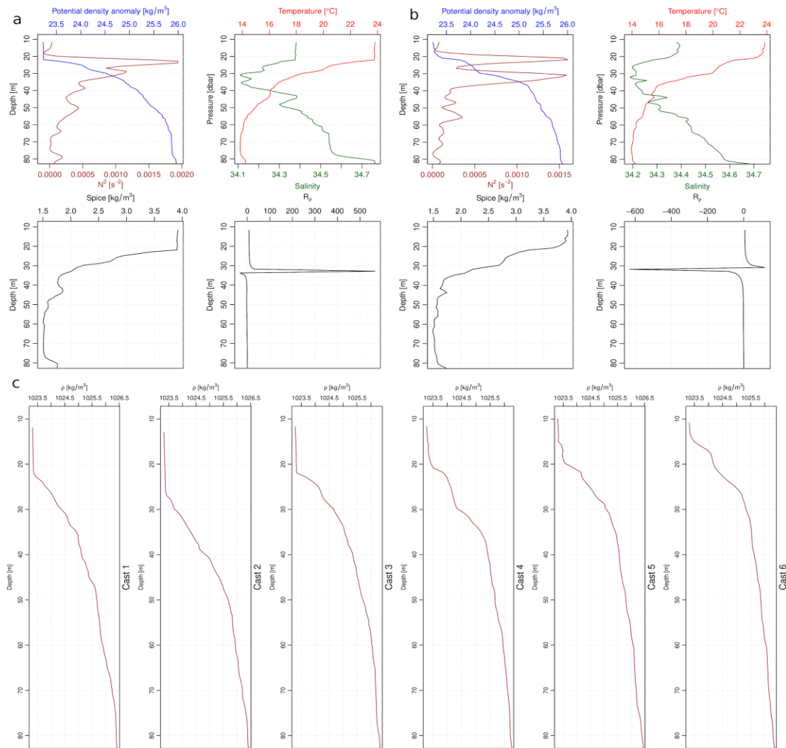
Ch 2 - Figure 15: Station 4 oceanographic plots, (a) four subplots for cast 3, clockwise from top left: {1} potential density anomaly Sigma-0 [ kg/m 3 ] top x-axis in blue, with the square of the buoyancy frequency in brown [N 2 [s -2 ]] , bottom x-axis. {2} Temperature in Celsius in red top x-axis, Salinity in PSU in green bottom x-axis. {3} Spice, ratio of (warm + salty)/ (cold+fresh) of water mass [kg/m 3 ]. {4} Rrho = change in f' of salinity/temperature over depth as described in methods. Salt finger implementation. (b) same sub plots for cast 4. (c) is casts: 1-6 of density as Sigma-theta [kg/m 3 ].
