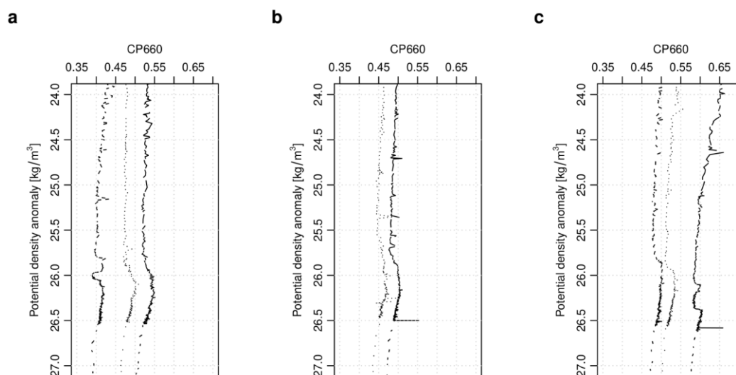
Ch 3 - Figure 10: Density profiles of cp660 , beam attenuation at 660 nm [ \text{m}^{-1} ] (a:c) for float 6903093 under Olaf. Three columns are profile groupings: prior, immediately following, and post disturbance, following sequential order corresponding time relative to TC overpass. Lines in each panel are dashed, dotted, solid in sequential order, within groupings. Days relative are: -20, -16, -10, 0, 4, 10, 20, 24. y-axis being Sigma-0 , potential density anomaly [ \text{kg}/\text{m}^3 ], as opposed to depth.
