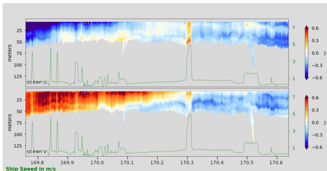
Ch 2 - Figure 3: Station 3.5 surface ADCP. Ocean current profiles from shipboard ADCP surface sensor over station 3.5. Time window corresponds to vessel sampling at Station 3.5. Top panel is zonal velocity, u , ( \text{m s}^{-1} ). Bottom panel is meridional, v , “”. Red is positive (East, North). Blue is negative (West, South). Times in decimal yr-day (169.80 ~ 2018-06-19 19:13 UTC-0). Green overlay/right axis is ship velocity ( \text{m s}^{-1} ). Left axis is depth to 150m. Panels are velocity components from the 300 kHz sensor.
