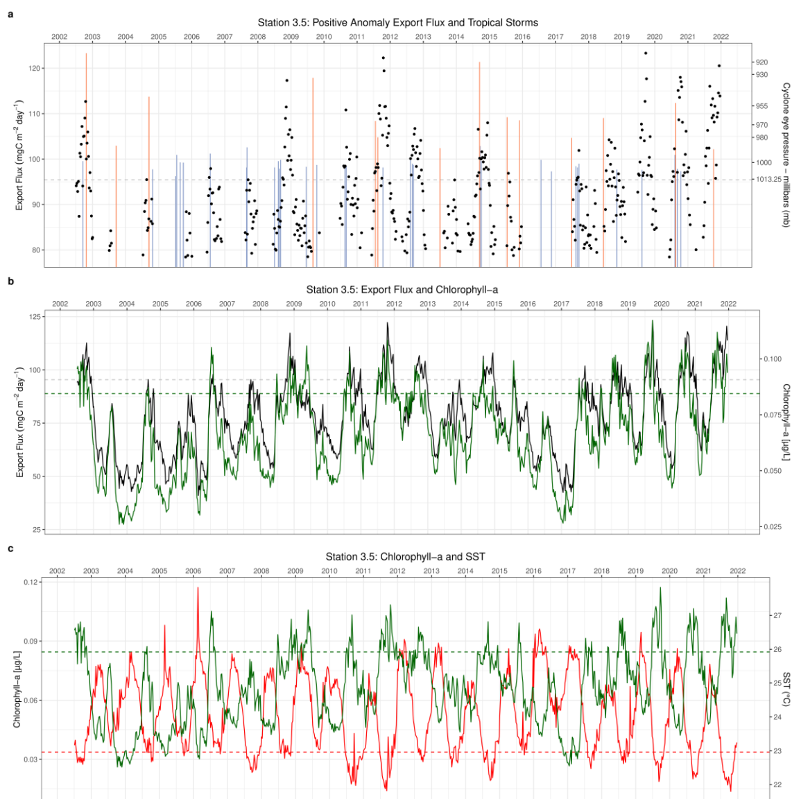
Ch 1 - Supplementary Figure 5: 8-day resolution: Non-lagged export flux (proportion of modeled VGPM). Derived from 8-day remotely sensed Chl-a & SST input variables. Values are mean computed for the 200km box around Station 3.5 ( \text{m}^{-2} \text{day}^{-1} ) for each variable (a) Export flux left axis ( \text{mg C} ). Positive anomalies only (above or equal to mean). Colored vertical lines are individual tropical disturbances that pass within the export 200 km flux box around Station 3.5. Orange = Hurricane strength, Blue = less than ". Height of each line is the median eye pressure per individual storm, which corresponds to the inverted right axis. Gray dashed horizontal line is 1 SD ( \sigma ) above mean export flux for time series, and corresponds to 1013.25 mb, standard atmospheric pressure at sea level for reference. (b) MODIS derived Chl-a [ \mu\text{g/L} ] in green/right axis, and export flux in black/left axis. Dashed horizontal lines are 1 SD ( \sigma ) above mean for time series (EF = gray, Chl-a = green). (c) MODIS derived Chl-a [ \mu\text{g/L} ] in green/left axis, and sea surface temperature ( ^{\circ}\text{C} ) in red/right axis. Dashed lines are 1 SD ( \sigma ) above/below mean for time series (Chl-a = green, SST = red).
