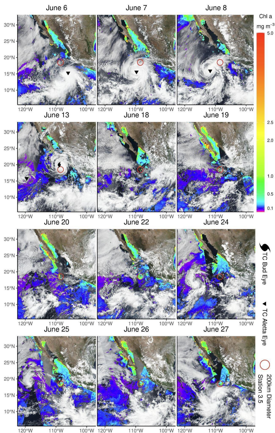
Ch 1 - Supplementary Figure 2: Select daily remotely sensed [Chl a] composites ( \text{mg m}^{-3} ) from June 6-27th 2018, with true-color cloud imagery overlaid, demonstrate the presence and influence of Hurricane Bud. [Chl a] values above 5 \text{ mg m}^{-3} are shown as red, while RGB imagery is shown for areas with no available [Chl a] values. The red circle (100 km radius) in all images is centered on Station 3.5. Eye position is shown for tropical cyclones Bud, and Aletta. See text for dates and specific storm strength designation. Images are ca. local solar noon. Larger area, and alternate days from Figure 2 main text.
