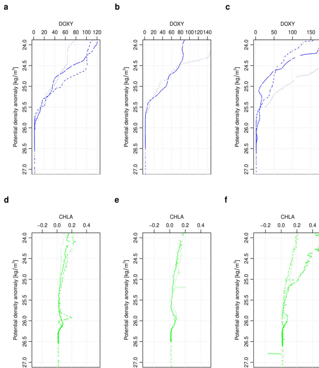
Ch 3 - Figure 9: Density profiles of oxygen [ \mu\text{mol/kg} ] (a:c), and Chl-a [ \mu\text{g L}^{-1} ] (d:f) for float 6903093 under Olaf. Three columns (a,d; b,e; c,f), are profile groupings: prior, immediately following, and post disturbance, following sequential order corresponding time relative to TC overpass. Lines in each panel are dashed, dotted, solid in sequential order, within groupings. Days relative are: -20, -16, -10, 0, 4, 10, 20, 24. y-axis being Sigma-0, potential density anomaly [ \text{kg/m}^3 ], as opposed to depth.
