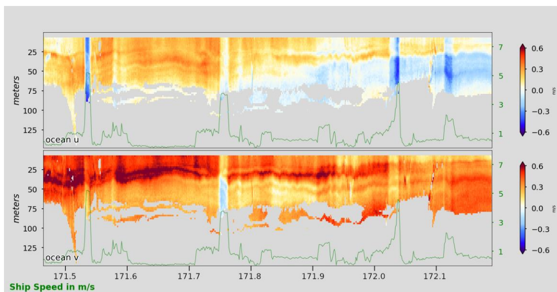
Ch 2 - Figure 11: Station 4 surface ADCP. Ocean current profiles from shipboard ADCP surface sensor over station 4. Time window corresponds to vessel sampling at Station 4. Top panel is zonal velocity, u , ( \text{m s}^{-1} ). Bottom panel is meridional, v , “”. Red is positive (East, North). Blue is negative (West, South). Times in decimal yr-day (171.5 ~ 2018-06-21 11:59 UTC-0). Green overlay/right axis is ship velocity ( \text{m s}^{-1} ). Left axis is depth to 150m. Panels are velocity components from the 300 kHz sensor.
