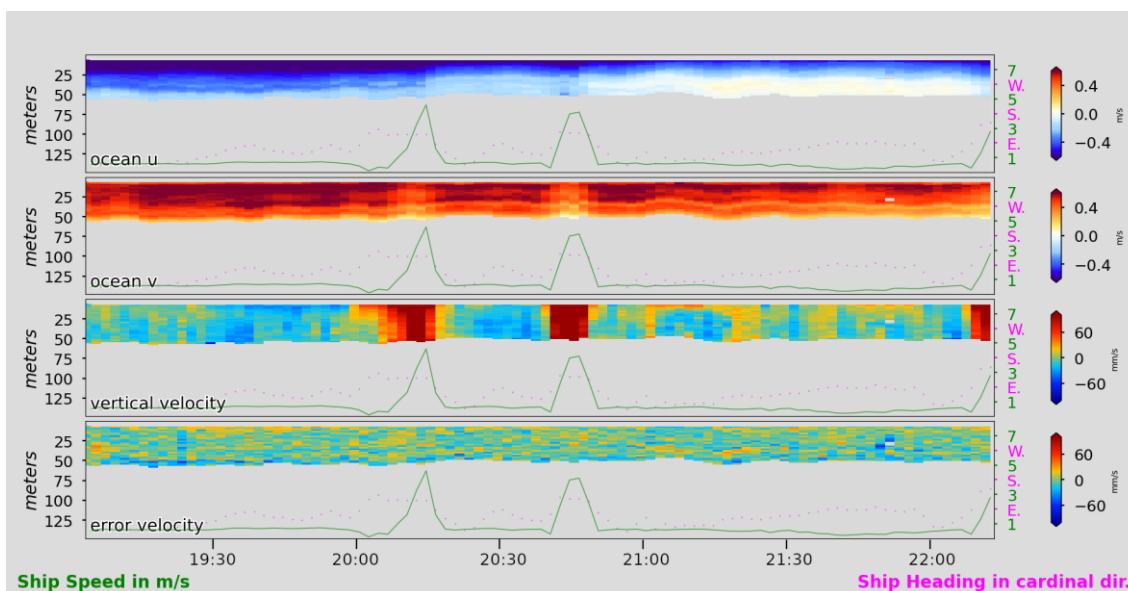
Ch 2 - Figure 23: ADCP station 3.5 shallow, casts 1 & 2. Ocean current profiles from shipboard ADCP surface sensor over station 3.5. Time window corresponds to CTD casts 1 and 2 (Table 1). First panel is zonal velocity, u , ( \text{m s}^{-1} ). Second panel is meridional, v , ( \text{m s}^{-1} ). Third panel is vertical velocity, w , ( \text{mm s}^{-1} ) a depth in meters. Gray indicates no data, or data removed due to ship movement induced noise. Bottom panel is error velocity in the vertical velocity panel. Gray indicates no data, or data removed due to ship movement induced noise. Red is positive (East, North, Up). Blue is negative (West, South, Down). Times in UTC-0 for 06-19. Green overlay/right axis is ship velocity. Pink dots/right axis is ship heading in cardinal direction. Left axis is depth to 1000m. Panels are velocity components from the 300 kHz sensor.
