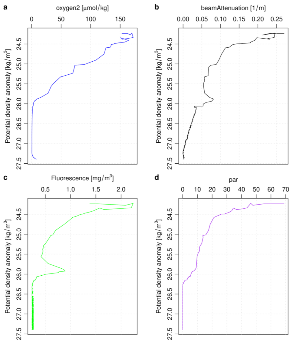
Ch 2 - Figure 7: Station 3.5 CTD profiles for the second cast, 19 - 21:04 UTC-0, by isopycnal surfaces. (a) oxygen [ \mu\text{mol/kg} ], (b) beam attenuation [ 1/\text{m} ], (c) fluorescence [ \text{mg}/\text{m}^3 ], and (d) percentage of available photosynthetically active radiation in purple [%]. y-axis being Sigma-0, potential density anomaly [ \text{kg}/\text{m}^3 ], as opposed to depth.
