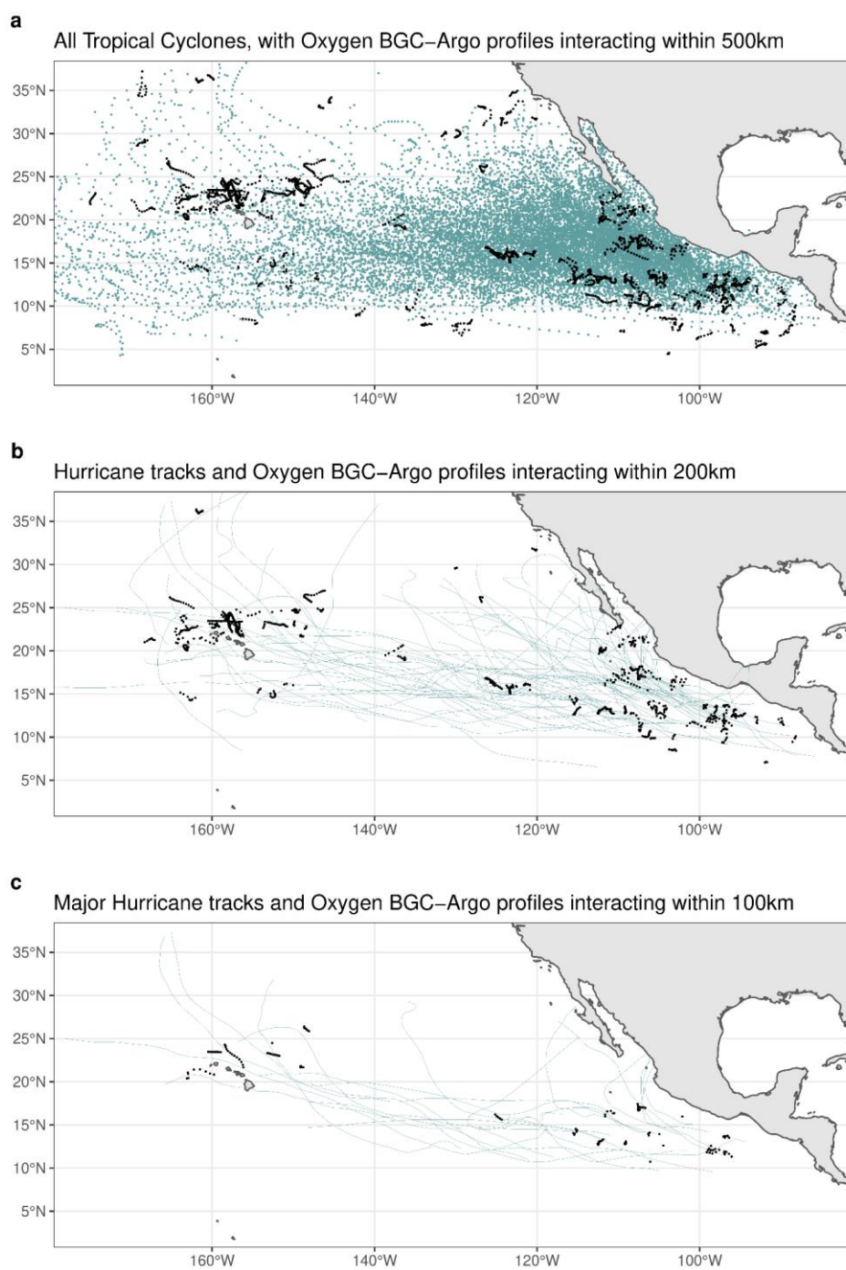
Ch 3 - Figure 1: Map of overlays of tropical cyclones and BGC–Argo profiles with oxygen sensors. Within the time and space selection window, see methods, Table 1. (a) All six hour positions for TC’s in the database, blue dots, with profiles of a float that fell within 500 kms, black dots. (b) Hurricane tracks, blue lines, and associated profiles falling within 200km, black dots. (c) Major hurricane tracks, blue lines, and associated profiles falling within 100km, black dots. Time window is from 30 days prior to or 45 days after TC overpass.
