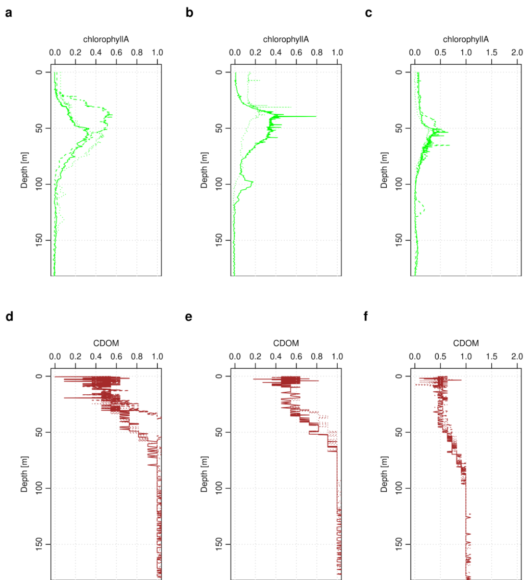
Ch 3 - Figure 8: Profiles of Chl-a [ \mu\text{g L}^{-1} ] (a:c), and CDOM (d:f) for float 6903093 under Olaf. Three columns (a,d; b,e; c,f), are profile groupings: prior, immediately following, and post disturbance, following sequential order corresponding time relative to TC overpass. Lines in each panel are dashed, dotted, solid in sequential order, within groupings. Days relative are: -20, -16, -10, 0, 4, 10, 20, 24.
