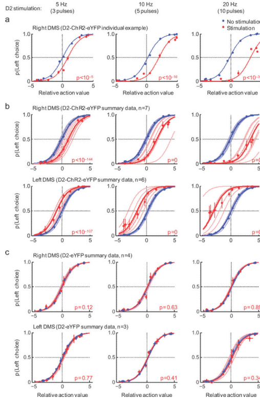
Figure 5. Dorsal striatal D2R-expressing neuron activation mimics a decrease in relative action value for contralateral choice
