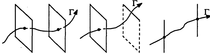
Figure 3.10: Example chain separators
