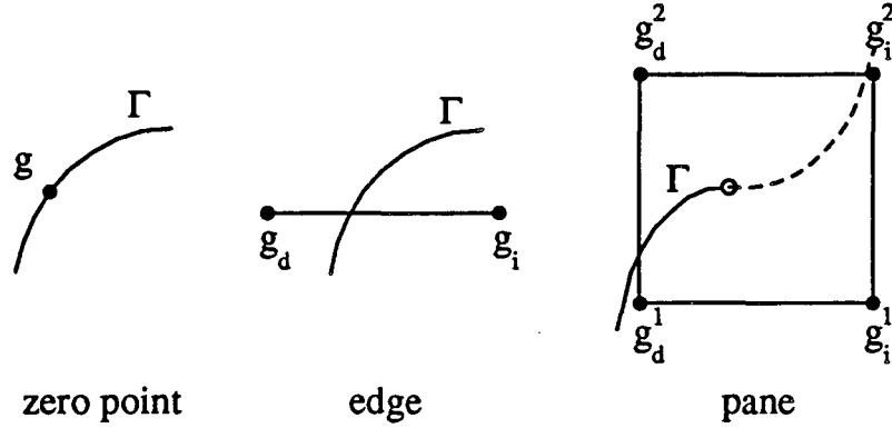
Figure 3.6: Interaction between a curve and a grid
