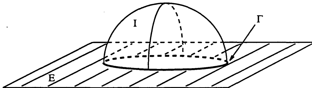
Figure 3.3: \Phi^{-1}(0) = E \cup I
