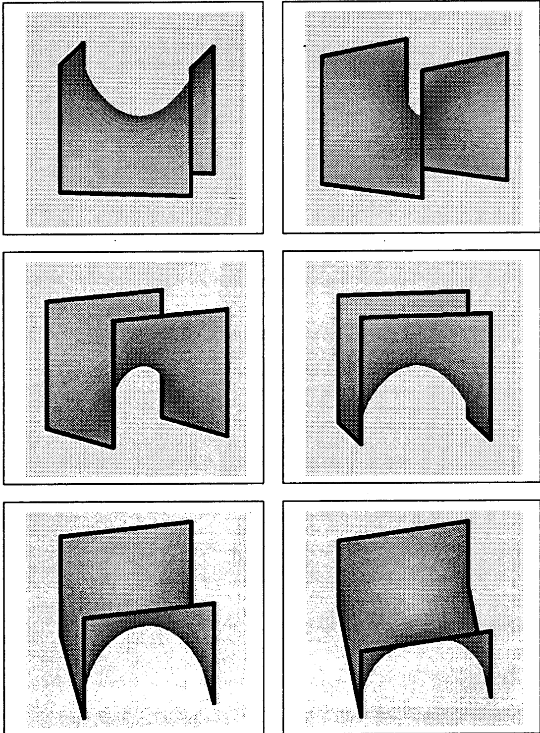
Figure 4.10: Square Sherck Surface
