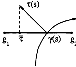
Figure 3.18: Edge dependency diagram
