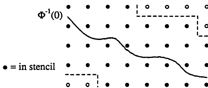
Figure 3.24: A 2-dimensional stencil diagram
