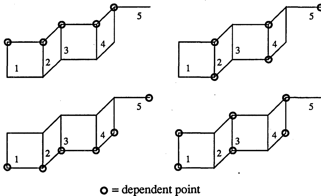
Figure 3.11: Four consistent labellings
