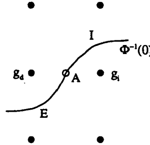
Figure 3.5: Grid points around the boundary
