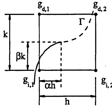
Figure 3.8: Dependency calculation of a pane
