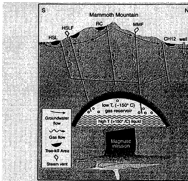
Figure 3.7. Theoretical model of Mammoth Mountain structure, posited gas reservoir, and geothermal system to explain the variety of CO 2 manifestations observed. HSL = Horseshoe Lake, HSLF = HSL fumarole, RC = Red Creek, MMF = Mammoth Mountain fumarole, and CH12 = chair 12 of the Mammoth Mountain ski resort (Sorey et al., 1999).
