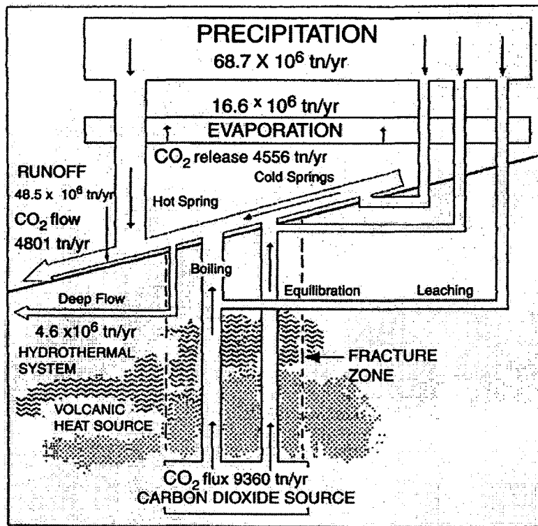
Figure 3.6b. Passive geothermal release of CO 2 at Furnas volcano, Sao Miguel, Azores, including precipitation, evaporation, and groundwater flow rates and CO 2 flux from springs and in runoff (Cruz et al., 1997). (tn = tonne).
