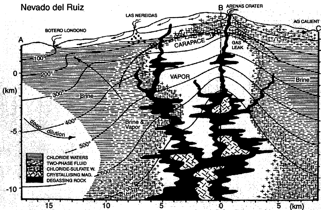
Figure 3.6a. Tentative cross section through Nevado del Ruiz, Colombia volcanic structure showing active volcanic releases of CO 2 . Heavy dashed line indicates likely position of chemically sealed carapace (from Giggenbach et al., 1990).
