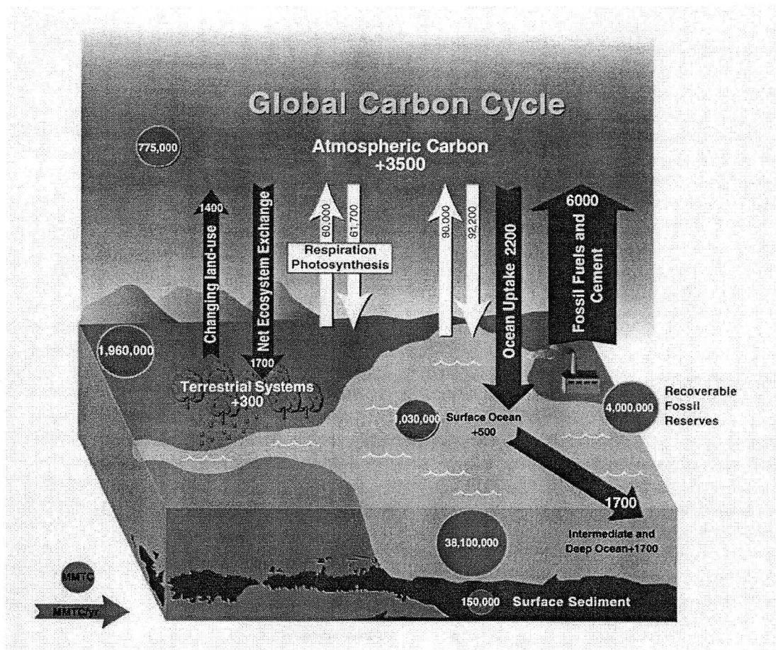
Figure 2.1. Global biogeochemical carbon cycle. Includes human influence from fossil fuel combustion and changing land-use patterns. Black arrows indicate net fluxes and white arrows indicate gross fluxes. Annual net additions are shown as + numbers, and pool sizes (circles) are shown in gray. All quantities are in Million Metric Tonnes Carbon, MMTC, and all fluxes are in MMTC/yr (modified from US DOE, 1999).
