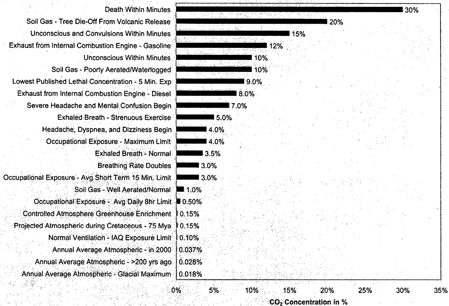
Figure 2.6. Comparison of ambient concentrations of CO 2 and risks of exposure. Data Tables with references attached as Appendix 4.
