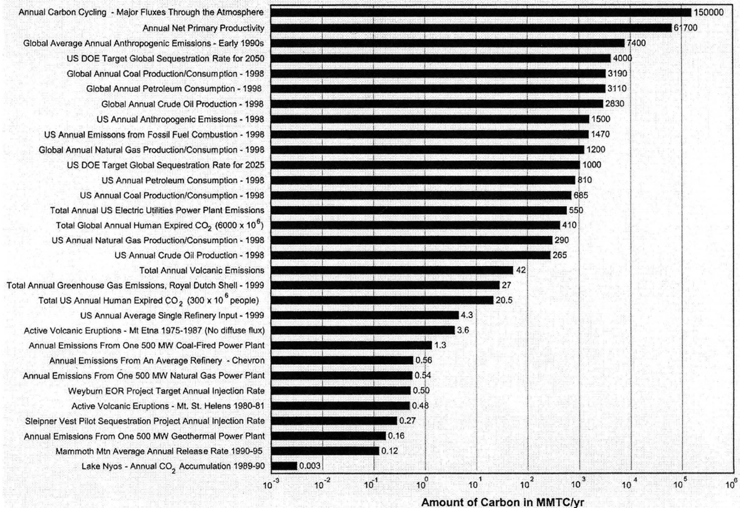
Figure 2.2b. Comparison of carbon fluxes and target sequestration rates. Data tables, references, and conversions are included as Appendices 2 and 3. Estimates are order of magnitude only and may include small conversion discrepancies due to independent rounding.
