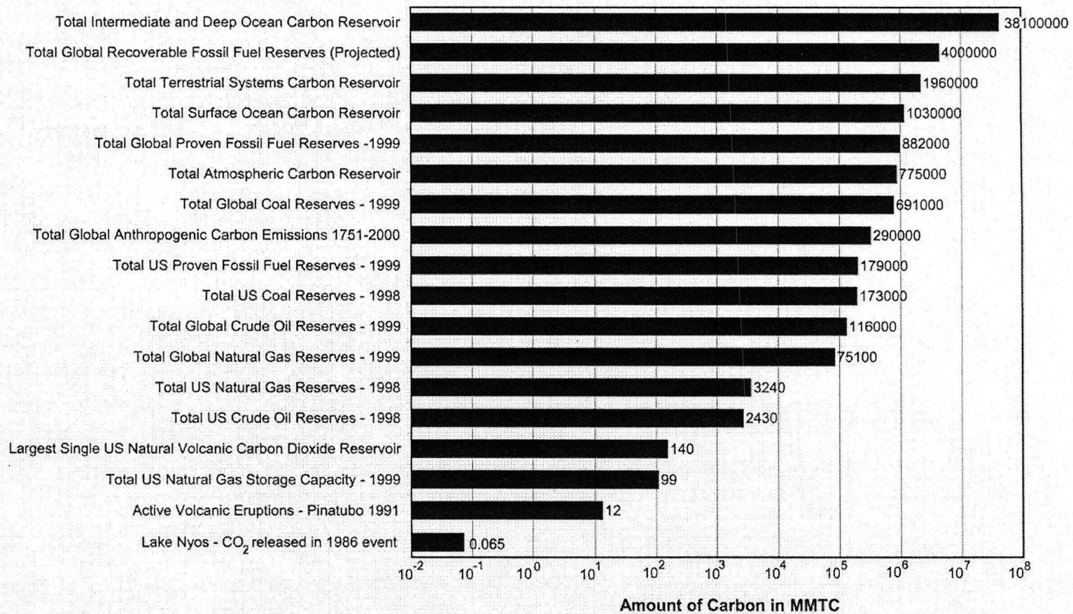
Figure 2.2a. Comparison of carbon reservoirs and one-time events. Data tables, references, and conversions are attached as Appendices 1 and 3. Estimates are order of magnitude only and may include small conversion discrepancies due to independent rounding.
