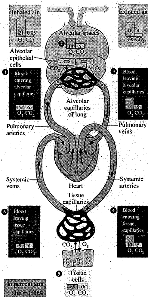
Figure 2.5. Gas exchange and variation in respiratory gas concentration along the coupled respiratory and circulatory systems (modified from Campbell et al., 1999).
