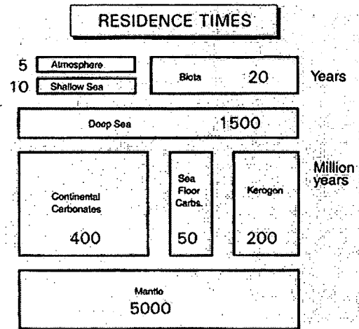
c) Residence time for carbon reservoirs (Walker, 1993).
