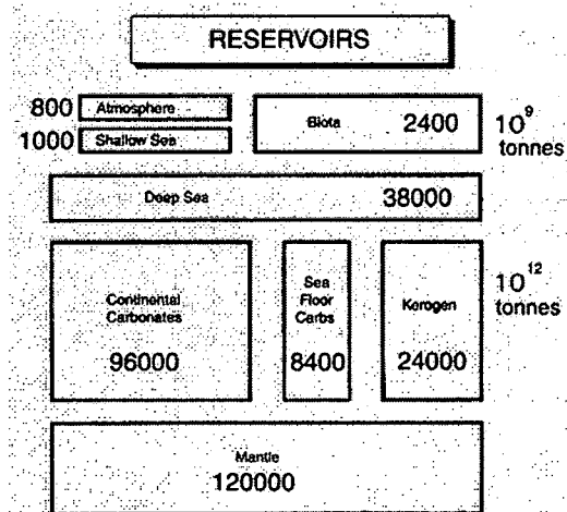
b.) Carbon reservoirs in metric tonnes of carbon (Walker, 1993).
