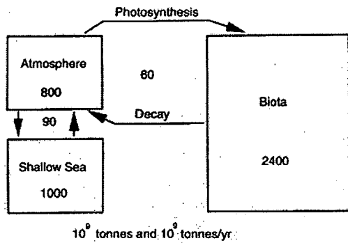
d) Fluxes among surface reservoirs of carbon (Walker, 1993).
