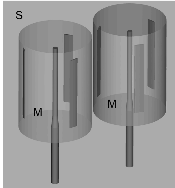
Figure 2.1: Computational domain for the two-VAWT case: Zoom on the rotating subdomains. The two cylindrical subdomains (labeled "M") spin with the rotors, while the remaining subdomain (labeled "S") is stationary.
