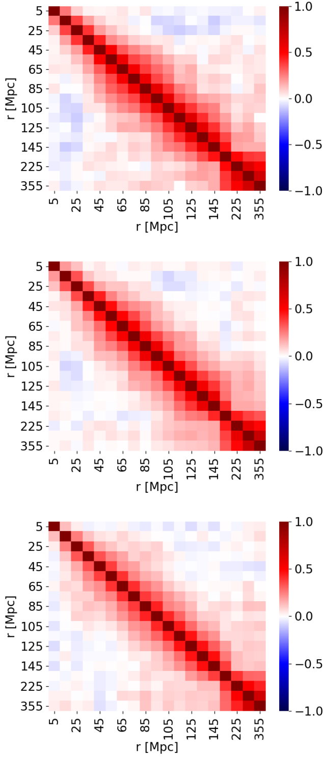
FIG. 9: The pairwise correlation matrix, for the DR4 ILC map across the 19 spatial cluster separation bins for the L43 galaxy tracer sample, derived from [top] the covariance across 560 noise sims, [center] the bootstrap and [lower] jack-knife resampling.
