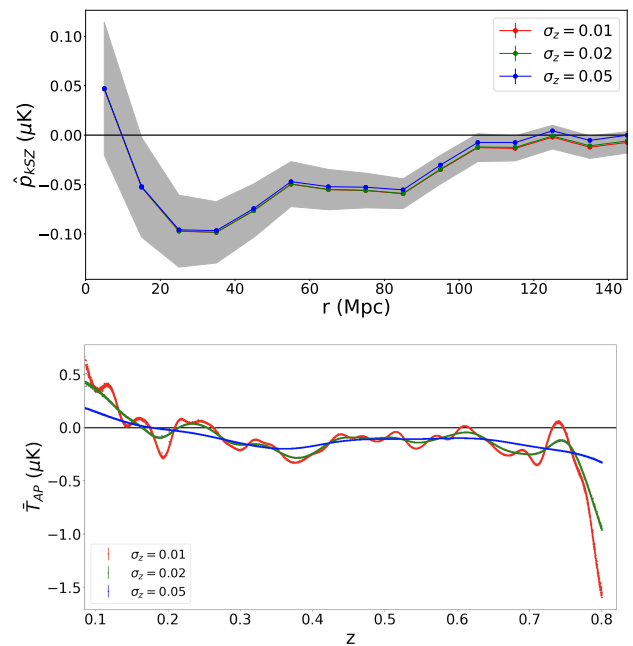
FIG. 5: Comparison of the impact of the redshift smoothing factor in the aperture photometry estimation for the DR4 ILC map and the DR15 L43 sample. [Upper] The uncertainties introduced in \hat{p}_{\text{kSZ}} when varying \sigma_z=0.01, 0.02, 0.05 are compared with 1\sigma uncertainties from noise simulations (assuming \sigma_z = 0.01 ). [Lower] The individual \bar{T}_{\text{AP}} realizations for each case.
