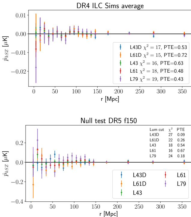
FIG. 1: Two null tests conducted on the pipeline for each galaxy tracer luminosity sample: [Upper] The mean and standard deviation of the pairwise estimator derived from the average sample covariance for the DR4 ILC 560 noise simulations. [Lower] A null test applied on the DR5 f150 map. Aperture photometries are taken from our science dataset for all luminosity bins, however the temperature decrement values are randomly shuffled which removes the pairwise signal. Error bars show one sigma uncertainty inferred with bootstrapping temperature decrements. The \chi^2 and the probabilities to exceed it are also given for each test.
