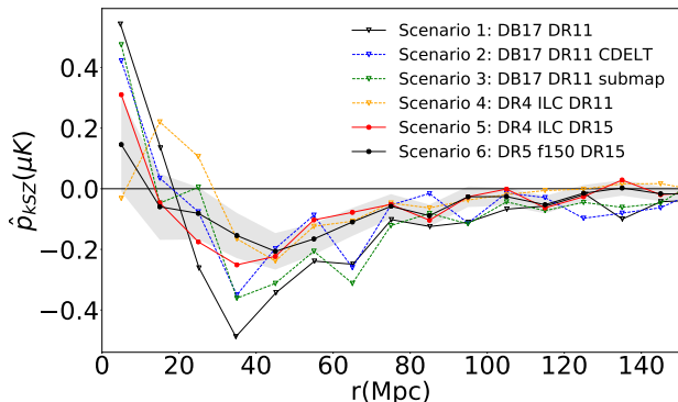
FIG. 6: Comparison of the impact of step-by-step changes in the aperture photometry assumptions in pairwise momentum estimation, \hat{p} obtained from those used in DB17 to this work. The stepwise changes in analysis and data are given in Table 3 for samples with a L > 7.9 \times 10^{11} L_{\odot} luminosity cut. The gray shaded region shows the 1\sigma bootstrap-derived uncertainties for the DR5 f150 analysis.
