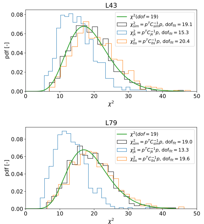
FIG. 8: Comparison of the distribution of \chi^2 values obtained from 560 simulation realizations evaluated on covariances inferred using: sims [Black], jackknife (‘jk’) [Blue] and bootstrap (‘bs’) [Orange] resampling of a single sim for the DR4 ILC [Upper] L43 and [Lower] L79 samples versus the theoretical prediction for \chi^2 for 19 degrees of freedom (equal to the number of spatial separation bins).
