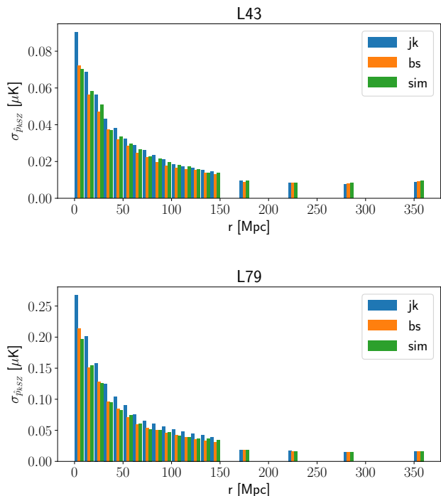
FIG. 7: Comparison of the standard deviation of 560 DR4 ILC noise simulations (‘sim’) [green] to the uncertainties obtained from the jackknife (‘jk’) [blue] and bootstrap (‘bs’) [orange] resampling of a single noise simulation for [Upper] L43 and [Lower] L79 galaxy tracer samples.
