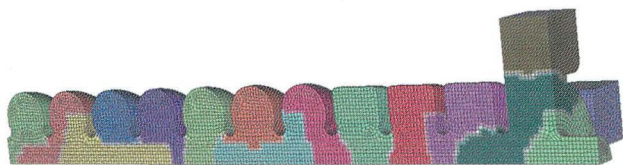
Tau3P simulation of the Next Linear Collider (NLC) Rounded Damped Detuned Structure (RDDS) output end, modeled on NERSC's T3E.
