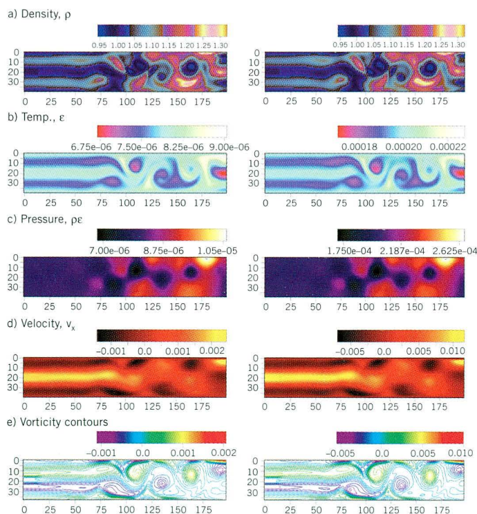
Evolution of 2D jet flow at Mach number 0.5 between constant temperature walls using the 9-bit energy-dependent lattice: a long-time comparison of the scaling integrity of the flows for Reynolds number = 20,000. Left column: timestep = 300 K, temperature = 8.0 (-6), v_0 = 2.0 (-3). Right column: timestep = 60 K, temperature = 2.0 (-4), v_0 = 1.0 (-2).
