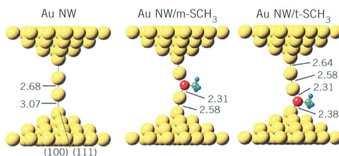
Equilibrium structures of a bare gold nanowire (AuNW, left) and of wires chemically modified by adsorption of a \text{SCH}_3 molecule, with the molecule adsorbed in the middle of the wire (m- \text{SCH}_3 ) or at the vicinity of the tip (t- \text{SCH}_3 ). Yellow spheres correspond to Au atoms, and in the chemically modified wires S, C, and H atoms are depicted by red, green, and blue spheres, respectively. Marked distances are in units of Å.
