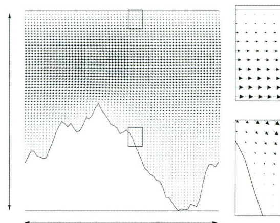
Example of the geometry and velocity field in a 2D fracture with one planar and one self-affine surface of roughness exponent H = 0.8 . The enlargements show the difference in the velocity decay near smooth and rough boundaries.
