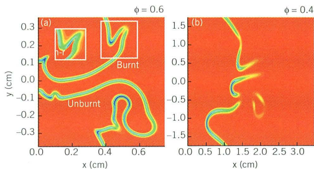
Isocontour plots of H 2 consumption rate for fuel-air equivalence ratios (a) 0.6 and (b) 0.4. The inset denoted h-r in (a) corresponds to heat release rate.
