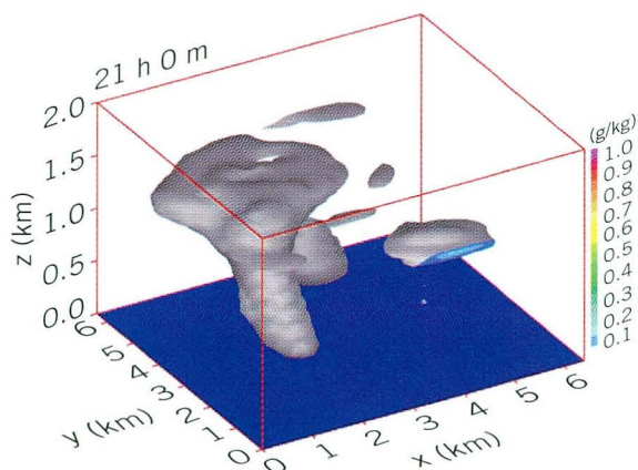
Isosurface of cloud water depicting the outer boundary of a trade cumulus cloud in simulations for studying the effects of aerosol pollution on clouds and hence global climate. The colored contours denote the liquid water content where the cloud intersects the edge of the model domain.
