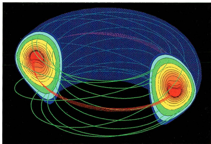
Numerical simulation of the nonlinear MHD evolution of shot 86144 in the DIII-D Tokamak at General Atomics, San Diego. Deformed pressure surfaces and magnetic field line trajectories are shown. The simulation used a realistic value of the plasma resistivity and was performed with the NIMROD code on the NERSC T3E.
