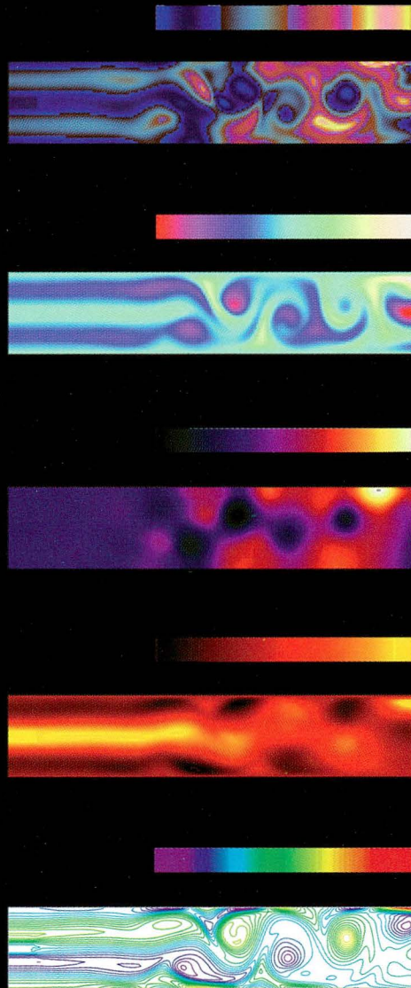
Snapshots of two-dimensional jet flow in a tokamak divertor simulation, showing density, temperature, pressure, velocity, and vorticity contours. See page 64 for details.
