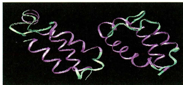
A comparison between the NMR structure of a four helix bundle DNA binding protein, 1pou (right), and the outcome from our global optimization algorithm (left). Purple indicates helical regions, while green indicates residues that are coil.
