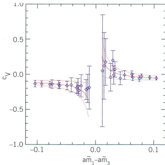
A fit of the form c_V = c_V^{(0)} + c_V^{(1)}/(\tilde{m}_1 - \tilde{m}_3) to extract the improvement constant for the vector current. The pole term is an artifact of lattice discretization, and resolved in our calculation.
