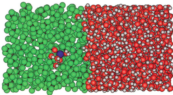
Transport of \text{Cs}^+ ion across a \text{CCl}_4/\text{H}_2\text{O} interface.
