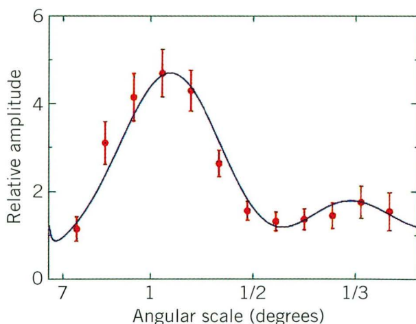
The strength of the CMB fluctuations on different angular scales as measured by BOOMERANG: points with error bars are the data, while the curve corresponds to the best-fitting cosmological model.
