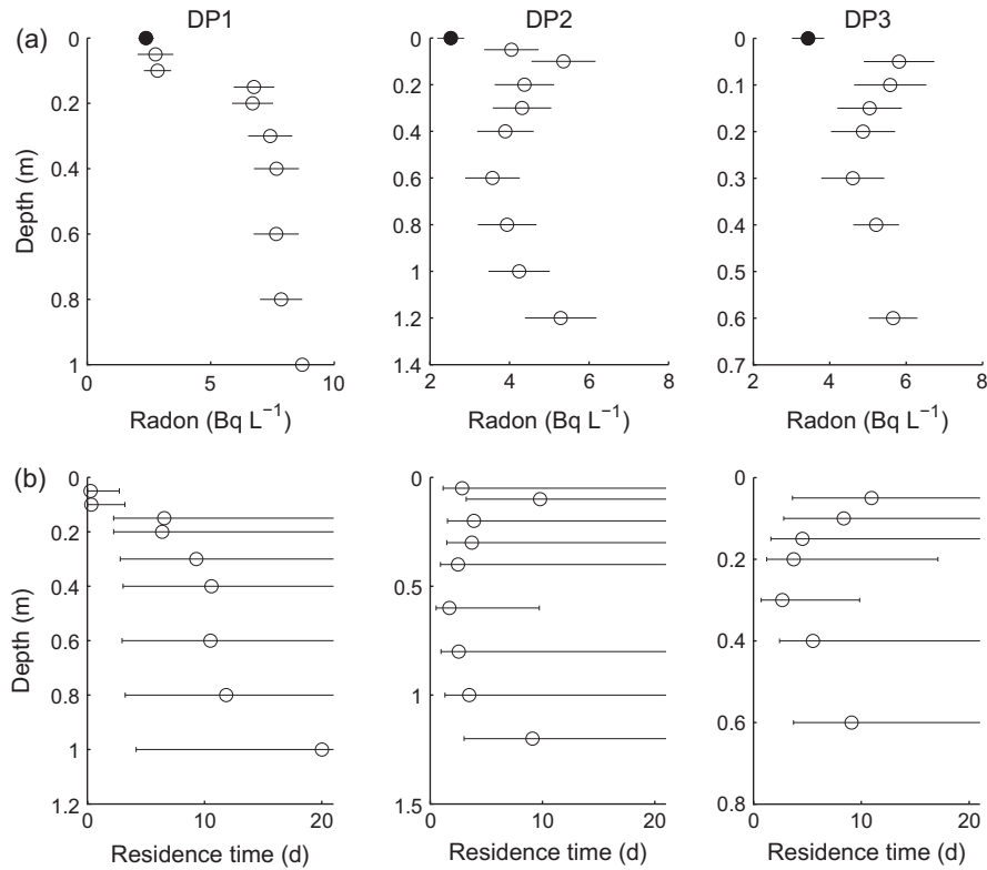
Fig. 4. (a) Streambed radon profiles. Dark circles are surface water samples, open circles are subsurface water samples. Error bars are 2\sigma based on laboratory measurement uncertainty. (b) Median hyporheic residence time and 90% confidence interval based on Monte Carlo analysis.
