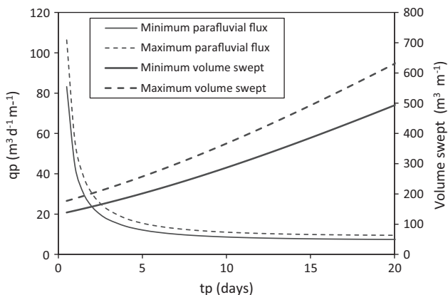
Fig. 7. Parafluvial fluxes and corresponding volume of alluvium flushed into each metre length of stream ( \text{m}^3 \text{m}^{-1} ) required to maintain radon activity in the stream at 2.4 \text{ Bq L}^{-1} as a function of parafluvial residence time. The minimum volume flushed assumes the hyporheic zone is 3 m deep with a mean residence time of 0.001 days. The maximum volume flushed assumes hyporheic radon flux is negligible.
