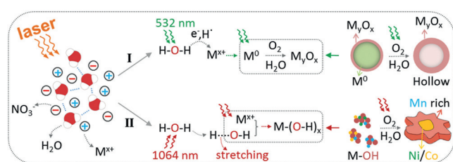
Scheme 1. Summary of the two possible reaction pathways for tailoring distinct complex nanostructures by irradiating aqueous 3d metal nitrates solutions with laser light, where M stands for Ni, Co, and Mn.
