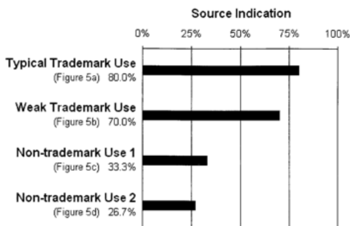
Figure 6. Results of Study 3
