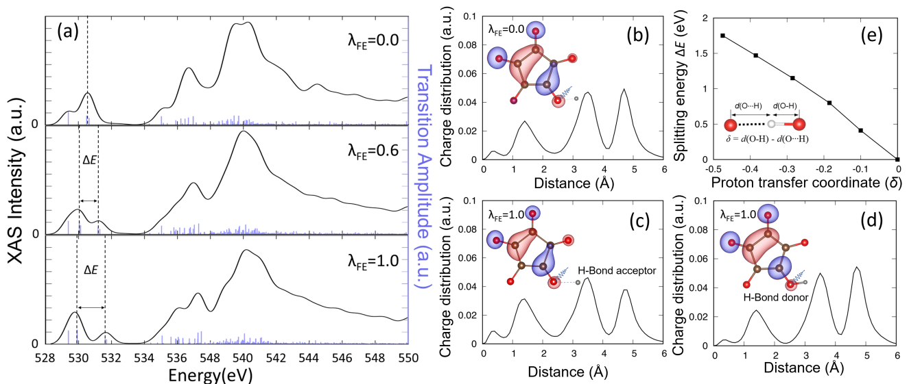
Figure 3. (a) The calculated XAS spectra (black) and XAS transition amplitude plots (purple) for CA crystal with different magnitudes of FE distortions of \lambda_{FE} = 0, 0.6, \text{ and } 1 . The dashed lines denote the peak positions when excited oxygen atoms are in different H-bonding environment. Note that the peak at around 529.4 eV belongs to the isolated Oxygen atom, whose peak position keeps the same with FE develop. (b), (c) and (d) Charge distribution of the excited oxygen atoms ( hinge direction) where the excited oxygens are oxygen atom in the paraelectric phase, H-bond acceptor pair oxygen atom in the FE phase, and H-bond donor pair oxygen atom in the FE phase, respectively. The zero point are located at the excited oxygen atom. The inserted figures in (b), (c) and (d) are selected excited molecular orbitals, where the white dot indicates the excited oxygen atoms. (e) The relation between splitting energy \Delta E and proton transfer coordinate \delta . The inserted figure is the schematic of the definition of proton transfer coordinate.
