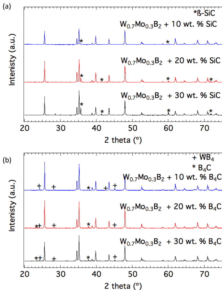
FIG. S2.5. PXRD data for: W_{0.70}Mo_{0.30}B_2 with 10, 20, and 30 wt. % (a) SiC addition and (b) B_4C . The growth of the secondary \beta -SiC phase (JCPDS 03-065-0360) is denoted by an asterisk (*) in (a). All patterns show (+) WB_4 (JCPDS 00-019-1373) and (*) B_4C (JCPDS 00-035-0798) in (b).
