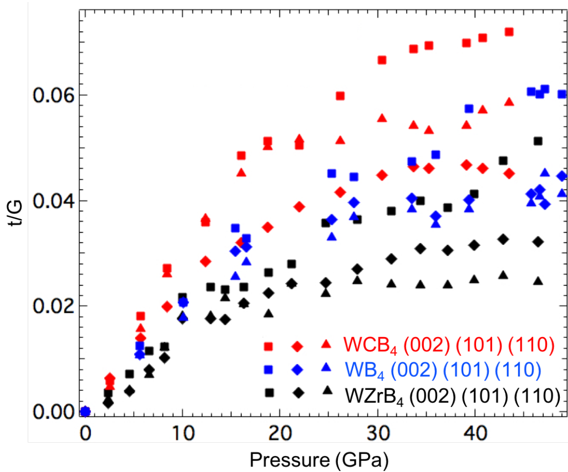
FIG. 4.10. The ratio of differential stress to shear modulus ( t/G ) for pure WB_4 (blue) compared to WB_4 with 8 at.% Zr (black) and 4 at.% C (red) addition.
