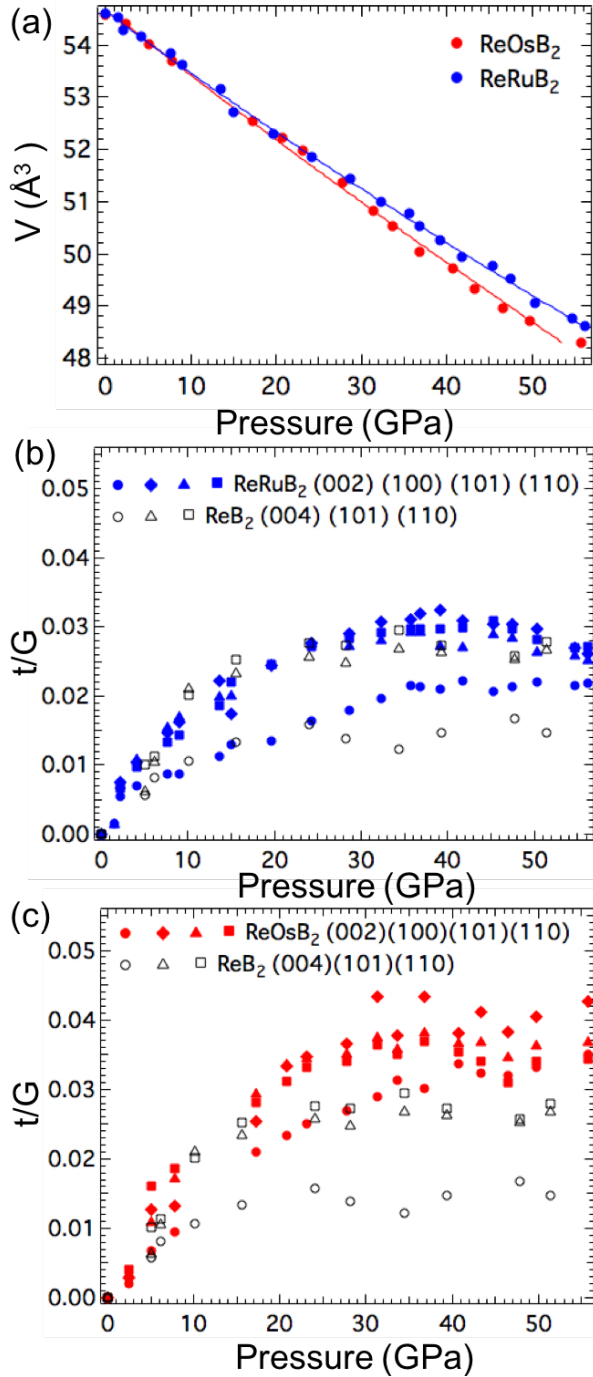
FIG. 3.4. Evolution of volume (a) of ReOsB 2 (red) and ReRuB 2 (blue) obtained at the magic angle \varphi=54.7^\circ upon pressure. The best fit lines to the Birch-Murnaghan equation-of-state on the volume are indicated by solid lines. Linear relationship between c/a ratio and pressure indicates no phase transition. Differential strain ( t/G ) as a function of pressure of ReRuB 2 (b) and ReOsB 2 (c), comparing with ReB 2 (open symbols).
