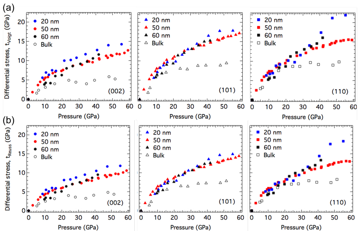
FIG. 7.6. Comparison of the differential stress ( t ) under (a) iso-strain ( t_{\text{voigt}} ) and (b) iso-stress ( t_{\text{reuss}} ) conditions as a function of pressure for 20 nm-, 50nm-, 60nm- and bulk- \text{ReB}_2 in the (002), (101) and (110) lattice planes. [Ref 22]
