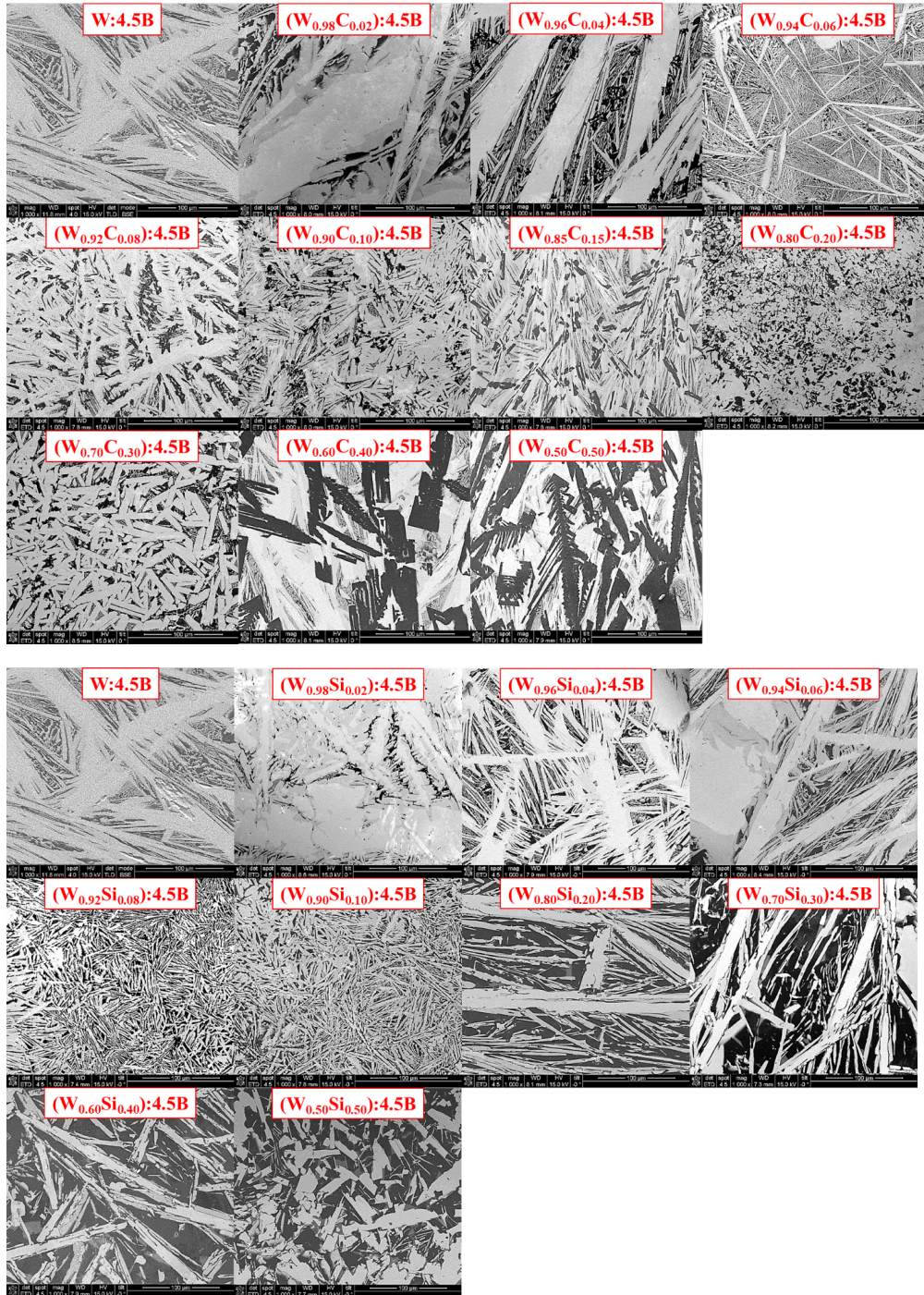
FIG. S4.2. SEM images for alloys of WB 4 with a nominal composition of (top) (W 1-x C x ) : 4.5B and (bottom) (W 1-x Si x ) : 4.5B showing a change in surface morphology associated with the effects of carbon and silicon and secondary phase formation. All SEM images were taken at 1000x magnification; the scale bars are 100 μm.
