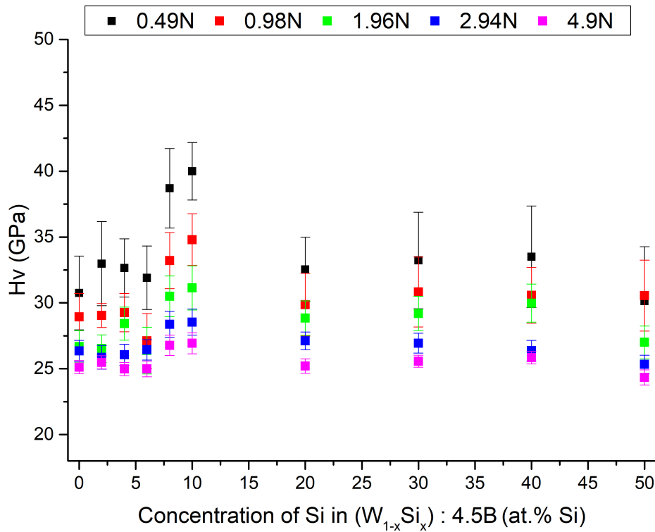
FIG. S4.5. Vickers micro-indentation hardness of alloys with a nominal composition of (top) (W_{1-x}C_x) : 4.5B and (bottom) (W_{1-x}Si_x) : 4.5B alloys at low (0.49 N) to high (4.9 N) loading.
