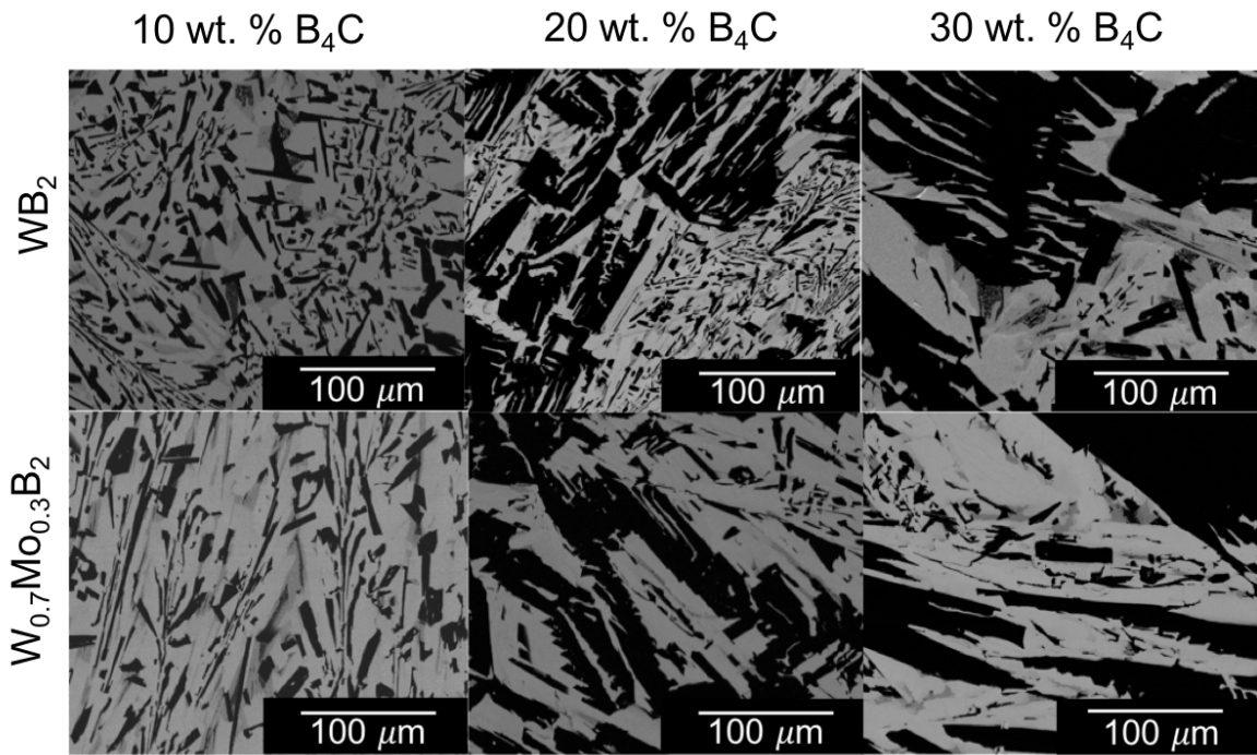
FIG. 2.9. SEM images of (top) WB 2 and (bottom) W 0.70 Mo 0.30 B 2 with 10, 20, and 30 wt. % B 4 C additions. Light gray regions represent areas of WB 2 and W 0.70 Mo 0.30 B 2 , while black regions represent B 4 C grains. A higher content of additional WB 4 impurity (shown as gray areas surrounding WB 2 and B 4 C) occurs in the WB 2 system, where more W is available for tetraboride formation.
