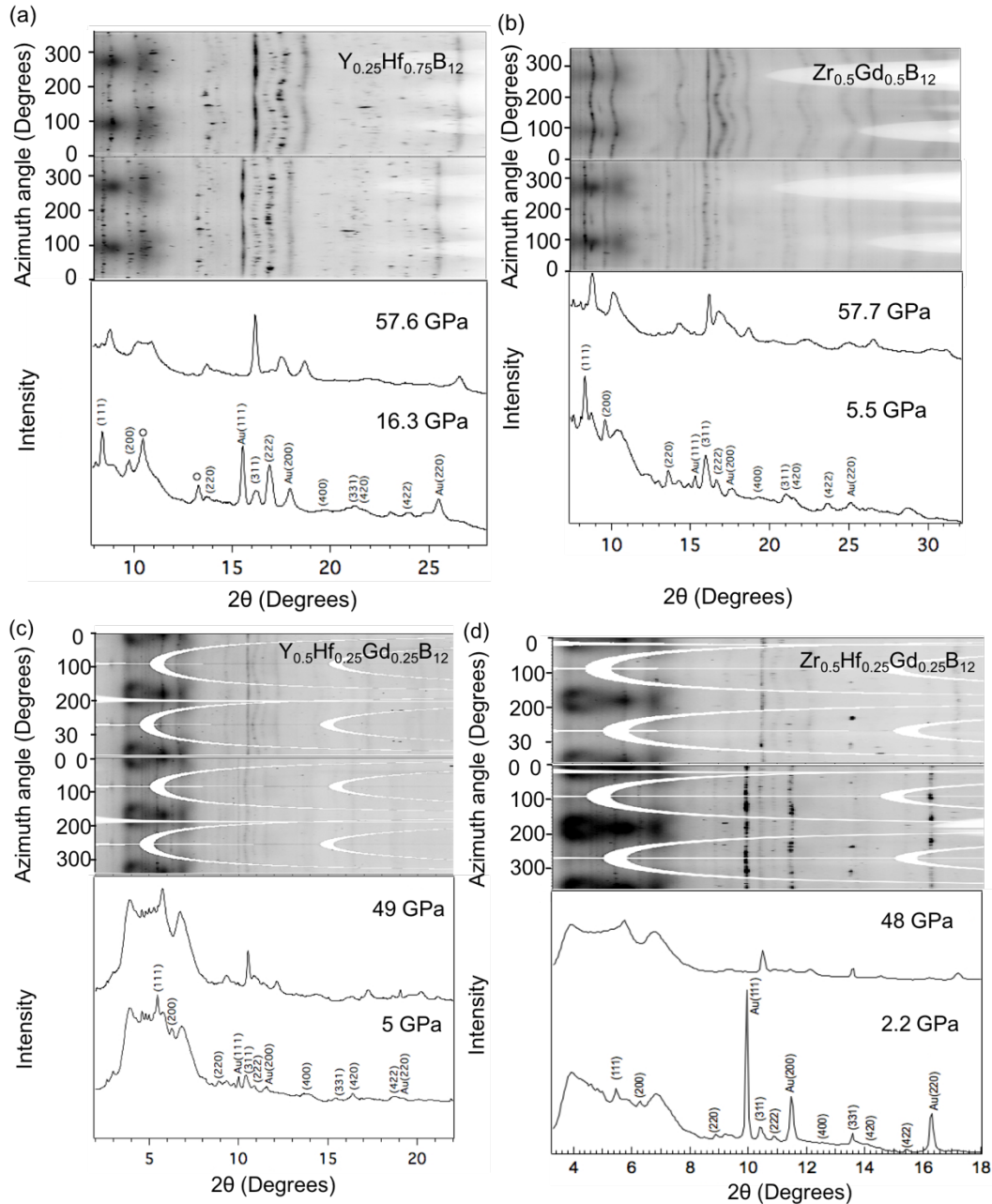
FIG. S5.1: Cake patterns (top) and full integrated 1-D diffraction (bottom) at low and high pressure for (a) Y_{0.25}Hf_{0.75}B_{12} , (b) Zr_{0.5}Gd_{0.5}B_{12} , (c) Y_{0.5}Hf_{0.25}Gd_{0.25}B_{12} , and (d) Zr_{0.5}Hf_{0.25}Gd_{0.25}B_{12} . The white arcs in the cake pattern in (c) and (d) are due to the grid lines in the Pilatus detector. Significant broadening is observed in the 1-D integrations at high-pressure due to strain anisotropy in the uniaxially compressed material.
