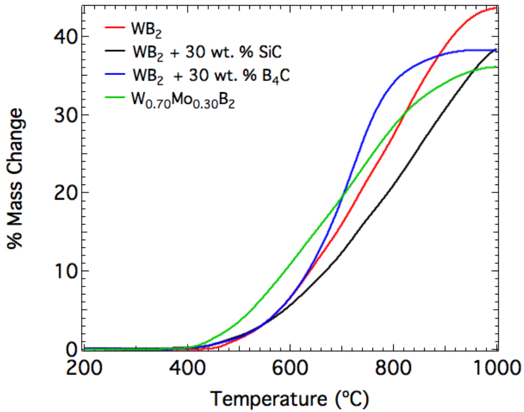
FIG. 2.11. Thermogravimetric analysis of unsubstituted WB_2 and the three hardest compositions studied in this work.
