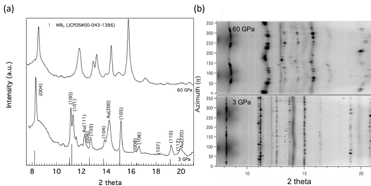
FIG. 2.4. Representative synchrotron (a) 1-D X ray diffraction patterns and (b) 2-D cake pattern of W_{0.70}Mo_{0.30}B_2 for low and high pressure. Cake patterns were obtained by integration over a 5^\circ slice centered at the magic angle ( \varphi=54.7^\circ ).
