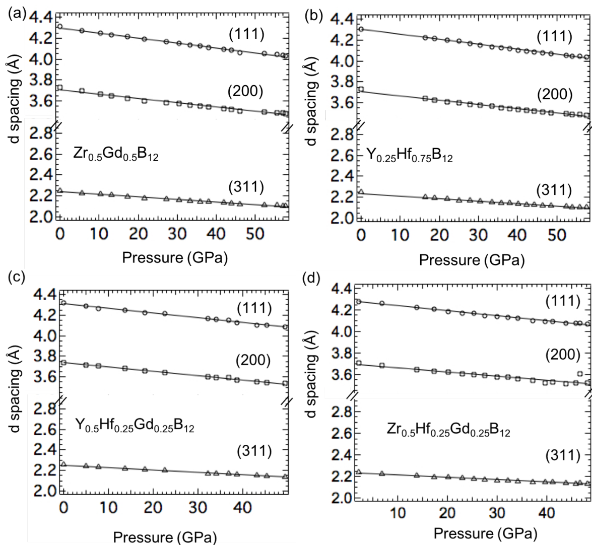
FIG. S5.3: Measured d-spacing vs. pressure for the (111), (200), (311) lattice planes in (a) Zr_{0.5}Gd_{0.5}B_{12} , (b) Y_{0.25}Hf_{0.75}B_{12} , (c) Y_{0.5}Hf_{0.25}Gd_{0.25}B_{12} , and (d) Zr_{0.5}Hf_{0.25}Gd_{0.25}B_{12} .
