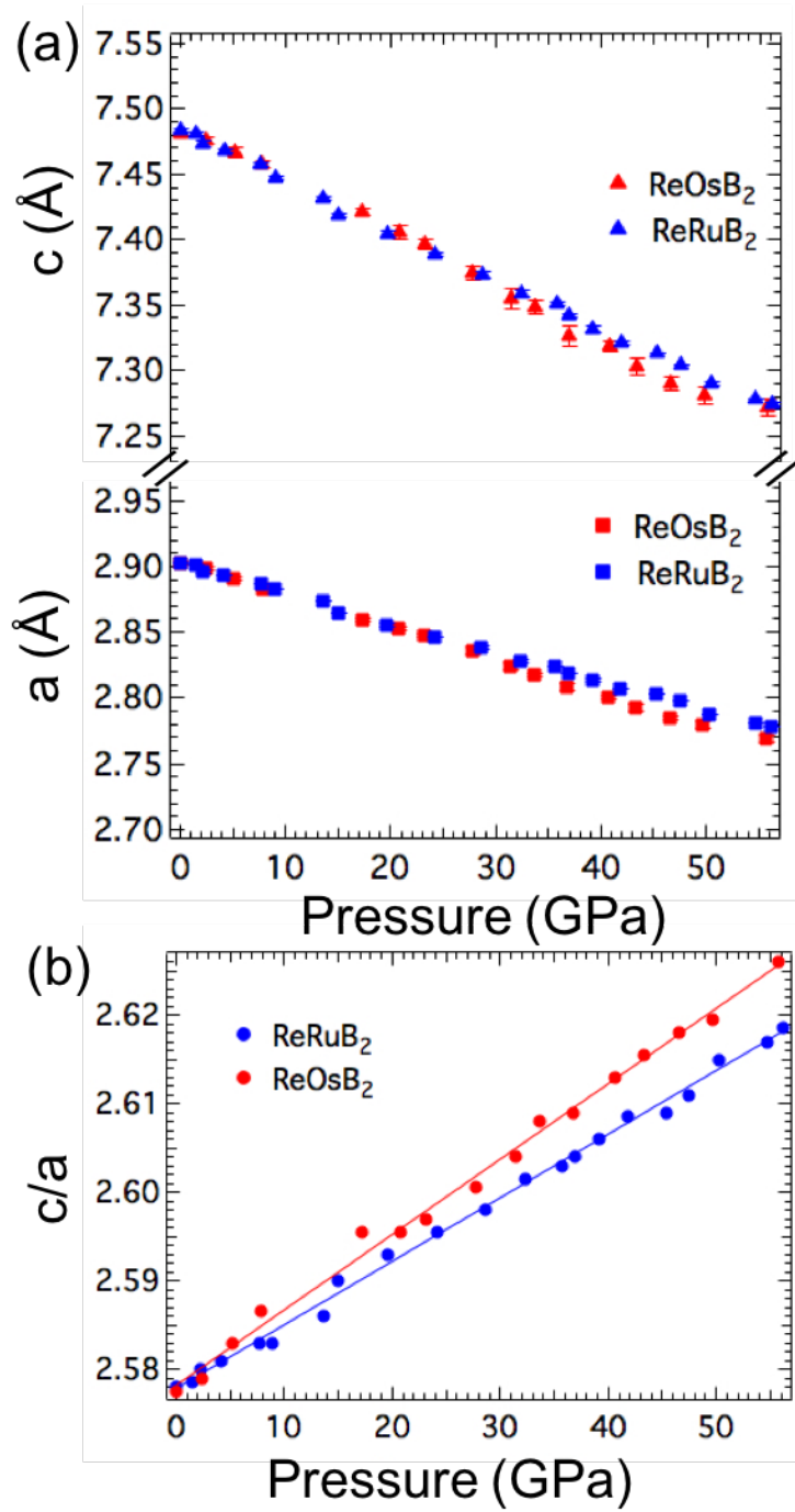
FIG. S3.4. Evolution of lattice constants (a) and c/a ratio (b) of ReOsB 2 (red) and ReRuB 2 (blue) obtained at the magic angle \varphi=54.7^\circ upon pressure. The error bar is shown on the graph.
