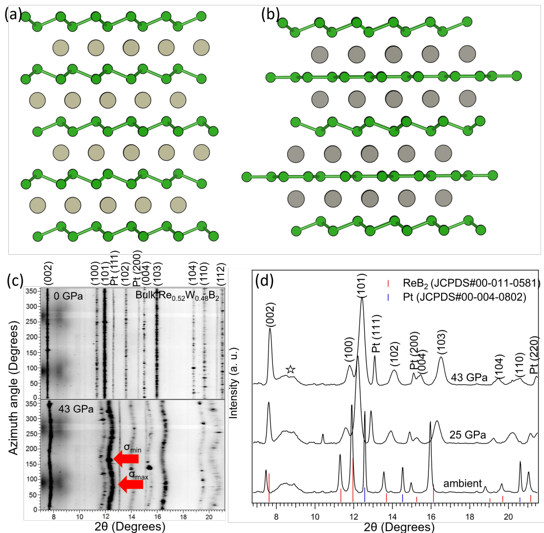
FIG. 6.1. A comparison of the structures of \text{ReB}_2 (a) and \text{WB}_2 (b). Boron and metal atoms are shown in green and gray, respectively. Representative synchrotron 2-D azimuthally unrolled patterns (c), and 1-D X-ray diffraction patterns (d) with increasing pressure for bulk \text{Re}_{0.52}\text{W}_{0.48}\text{B}_2 . The data in part (d) were obtained by integration over an 5^\circ slice center at the magic angle of \varphi = 54.7^\circ . Indexing for relevant peaks is included on the image (note that the stick pattern is for \text{ReB}_2 , not \text{Re}_{0.52}\text{W}_{0.48}\text{B}_2 ). Diffraction from the boron/epoxy gasket is indicated with an open star. All diffraction peaks other than those from the gasket shift to higher angle with increase pressure.
