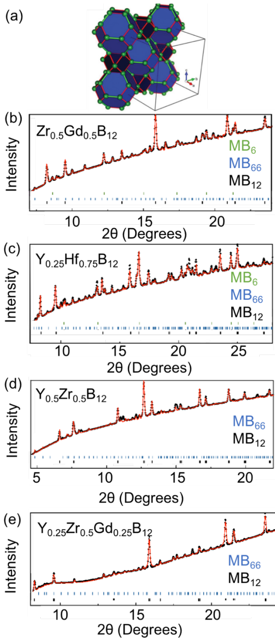
FIG. 5.1. A polyhedral view of crystal structure of (a) metal dodecaborides. Rietveld refinement of X-ray diffraction patterns to the orthorhombic structure for (b) Zr_{0.5}Gd_{0.5}B_{12} , (c) Y_{0.25}Hf_{0.75}B_{12} , (d) Y_{0.5}Zr_{0.5}B_{12} , and (e) Y_{0.25}Zr_{0.5}Gd_{0.25}B_{12} . The refinements include the parent MB_{12} phase, as well as any impurities present ( MB_2 , MB_6 , MB_{66} , M = \text{metal} ). The phases present in each sample are listed in the order of stick patterns shown at the bottom of each graph. Part (a) was reproduced with permission. 9 Copyright 2019, Advanced Functional Materials.
