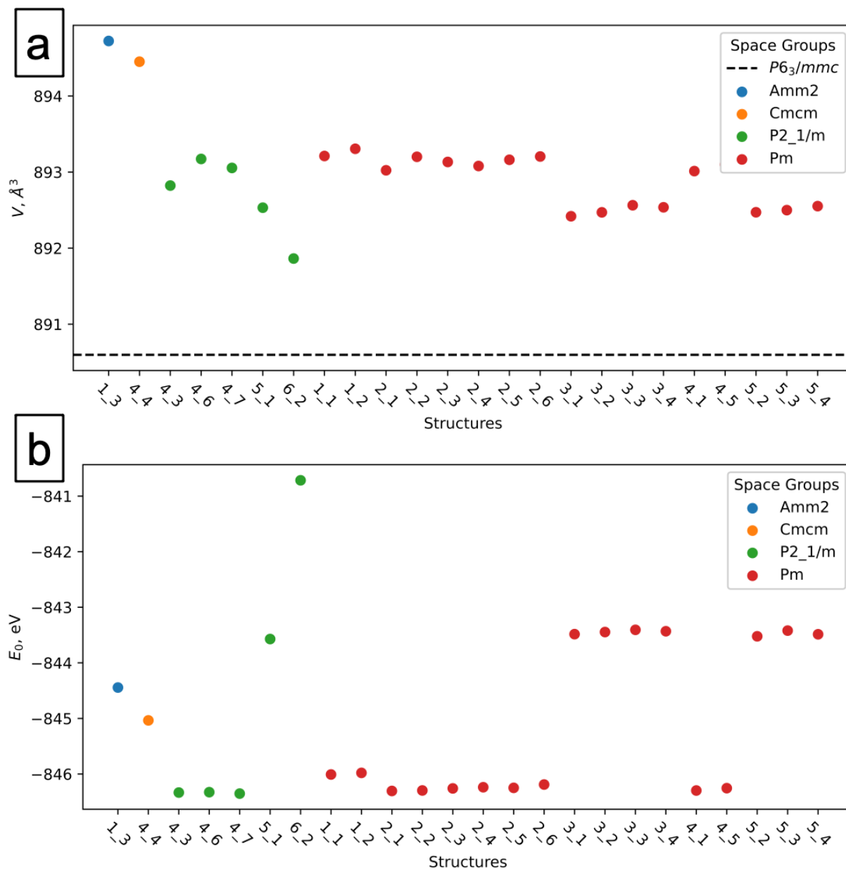
FIG. S4.11. Ensemble of 3 \times 2 \times 1 -supercell \text{WB}_{4.2} realizations. (a) Volumes of various realizations.
