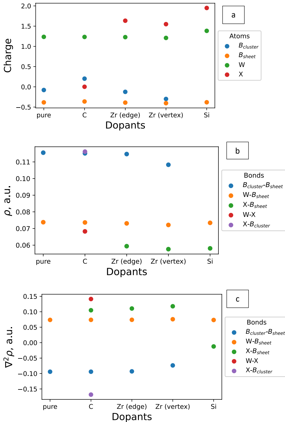
FIG. 4.12. QTAIM analysis of BCPs for model structures. (a) Average Bader atomic charges in model structures. (b) Average electron density at BCPs, connecting “layers” of the material. Average Laplacian at BCPs, connecting “layers” of the material.
