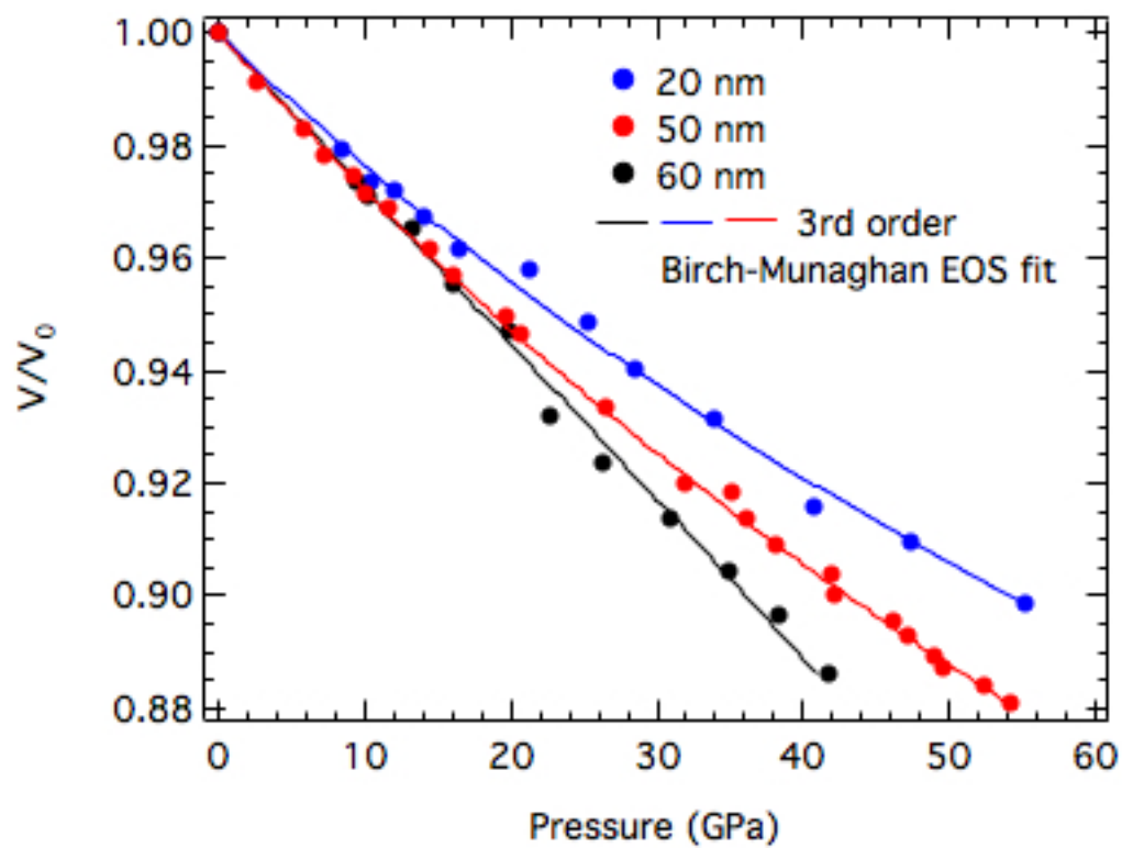
FIG. 7.5: Hydrostatic compression curves of 20 nm-, 50 nm- and 60 nm-ReB 2 obtained at the magic angle ( \varphi = 54.7^\circ ). The solid line is fit to the third-order Birch-Murnaghan equation-of-state.
