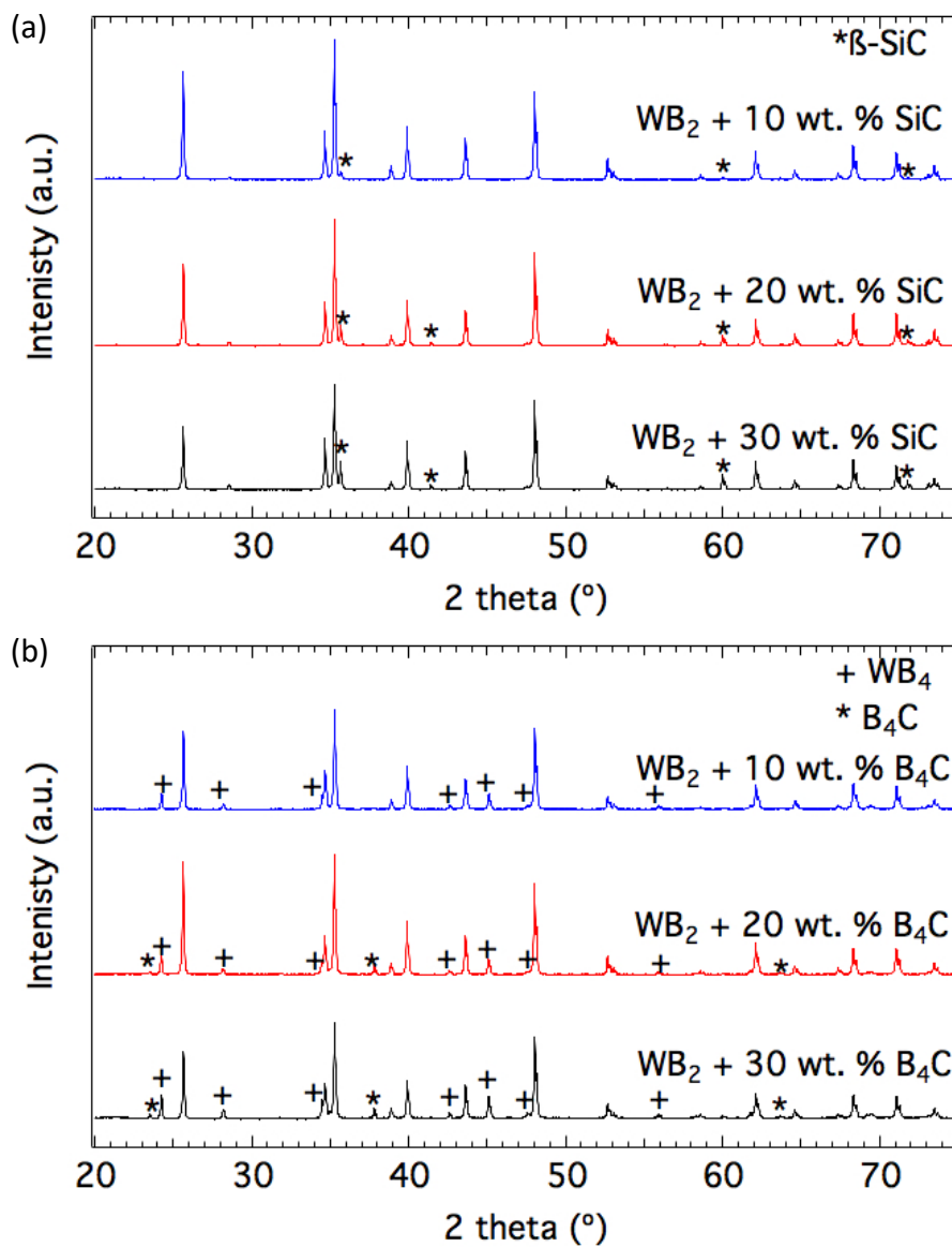
FIG. 2.10. PXR D data of: WB_2 with 10, 20, and 30 wt. % (a) SiC addition and (b) B_4C . The growth of the secondary \beta -SiC phase (JCPDS 03-065-0360) is denoted by an asterisk (*) in (a). All patterns show (+) WB_4 (JCPDS 00-019-1373) and (*) B_4C (JCPDS 00-035-0798) in (b).
