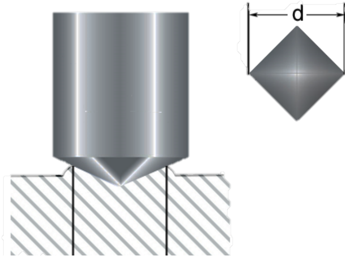
FIG. 1.1. Schematic figure for the micro-indentation hardness test.
