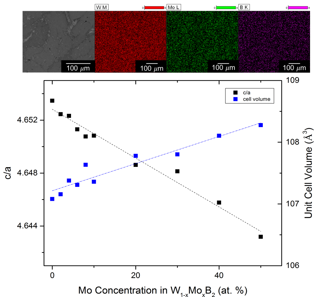
FIG. 2.2. (Top) SEM BSED image and elemental maps for tungsten (M line), molybdenum (L line), and boron (K line) for W_{0.70}Mo_{0.30}B_2 showing a uniform distribution of tungsten and molybdenum throughout the grains. (Bottom) Plot of (black) axial ratio, c/a , calculated from XRD cell refinement and (blue) unit cell volume calculated from W_{1-x}Mo_xB_2 lattice parameters versus Mo concentration in atomic percentage. Dashed lines represent linear trendlines as a function of Mo concentration. Unit cell parameters of all compositions are provided in Table S2.1 .
