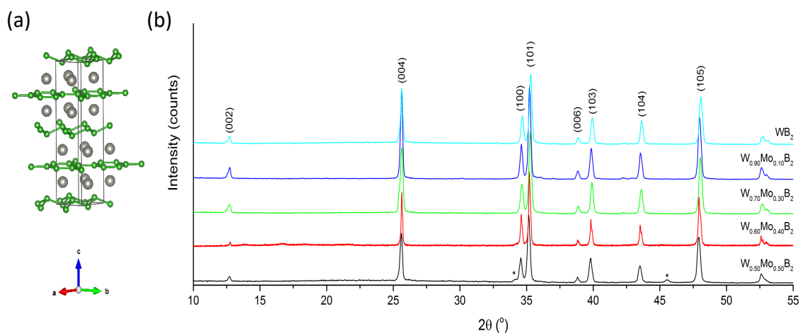
FIG. 2.1. (a) Crystal structure of tungsten diboride, WB_2 [ P6_3/mmc , Inorganic Crystal Structure Database (ICSD) 023716], where the unit cell is indicated by the black box. Boron atoms are represented in green as flat and puckered alternating sheets. Tungsten atoms are represented in gray. (b) Selected PXRD data of tungsten diboride ( WB_2 ) solid solutions with up to 50 at. % molybdenum (Mo). The solubility limit is below 40 at. % Mo. WB_2 (JCPDS 00-043-1386) is present at all concentrations of Mo, while \beta - MoB_2 (JCPDS 01-075-1046) appears in the 40 and 50 at. % Mo samples, denoted by an asterisk (*).
