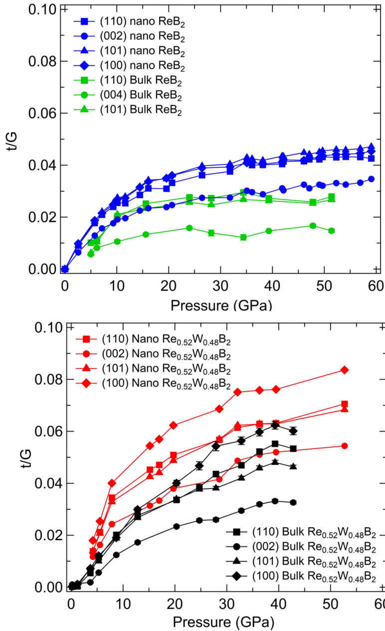
FIG. 6.6. (a) Comparison of the differential strain, given by the ratio of differential stress t to aggregate shear modulus G , as a function of pressure between nano- \text{ReB}_2 (blue) and bulk \text{ReB}_2 (green). (b) Differential strain as a function of pressure for nano- \text{Re}_{0.52}\text{W}_{0.48}\text{B}_2 (red) and bulk \text{Re}_{0.52}\text{W}_{0.48}\text{B}_2 (black).
