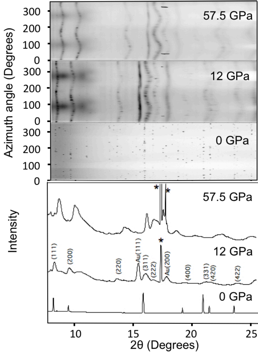
FIG. 5.3. Representative cake patterns (top) and 1-D diffraction patterns (bottom) of \text{Zr}_{0.5}\text{Y}_{0.25}\text{Gd}_{0.25}\text{B}_{12} at ambient, low and high pressure. The peaks in the 1-D full integrations broaden as the pressure increases because the integration is averaging over the varying stress states within the high pressure cell. The high intensity peak marked with an asterisk stems from the strong texture of the large grains in the sample.
