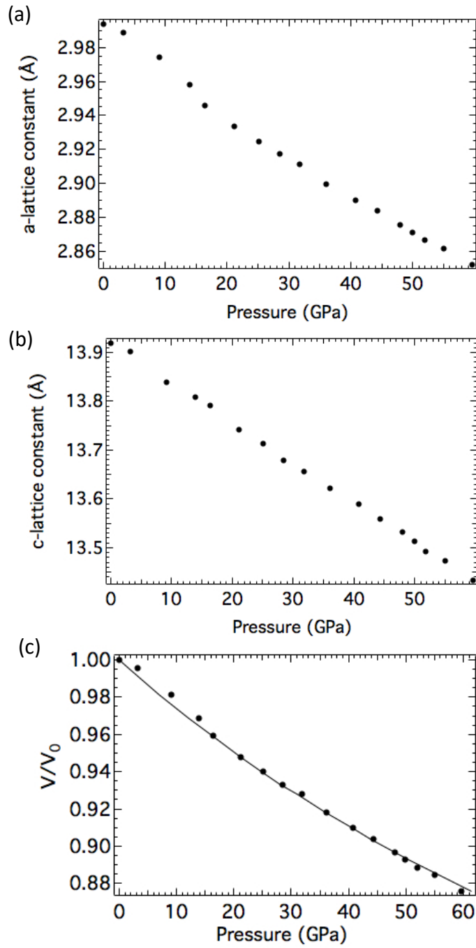
FIG. S2.2. Evolution of: (a) a-lattice constant, (b) c-lattice constant and (c) plot of volume change versus pressure for W_{0.70}Mo_{0.30}B_2 . The curve is calculated from the second order Birch-Murnaghan equation of state, where K_0' is fixed at 4.
