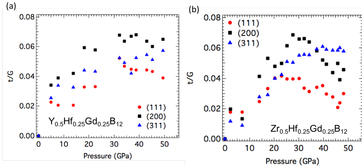
FIG. S5.4: Measure t/G vs. pressure for (a) Y_{0.5}Hf_{0.25}Gd_{0.25}B_{12} , and (b) Zr_{0.5}Hf_{0.25}Gd_{0.25}B_{12} .
