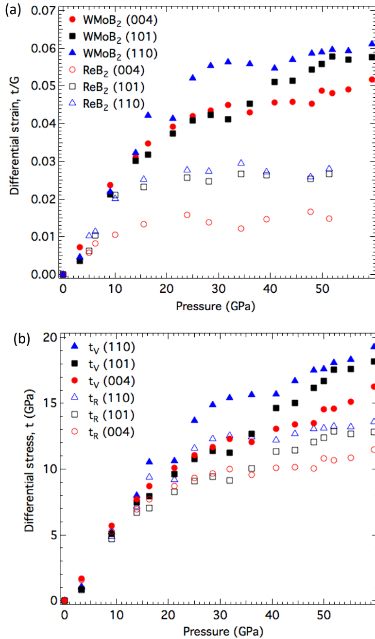
FIG. 2.6. (a) Comparison of the differential strain, given by the ratio of the differential stress ( t ) to shear modulus ( G ), as a function of pressure for both W_{0.70}Mo_{0.30}B_2 (W 0.70 Mo 0.30 B 2 ) and ReB 2 . (b) Differential stress ( t ) calculated under Reuss (isostress, t_R ) and Voigt (isostrain, t_V ) conditions for W 0.70 Mo 0.30 B 2 .
