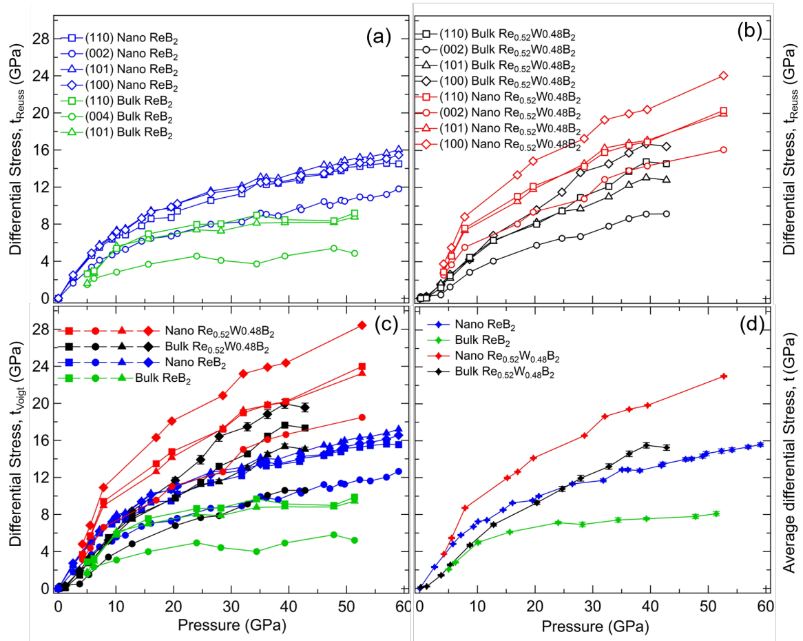
FIG. 6.7. Differential stress ( t ) calculated under the Reuss (iso-stress) condition (a), (b) and Voigt (iso-strain) condition (c). Part (a) compares bulk and nanoscale \text{ReB}_2 , while part (b) shows bulk and nanoscale \text{Re}_{0.52}\text{W}_{0.48}\text{B}_2 . Lattice planes are indicated on the figure. Part (c) compares all four samples, and the indexing is the same as that used in parts (a) and (b). Part (d) shows the evolution of the average differential stress over all observed lattice planes with pressure for the same four samples.
