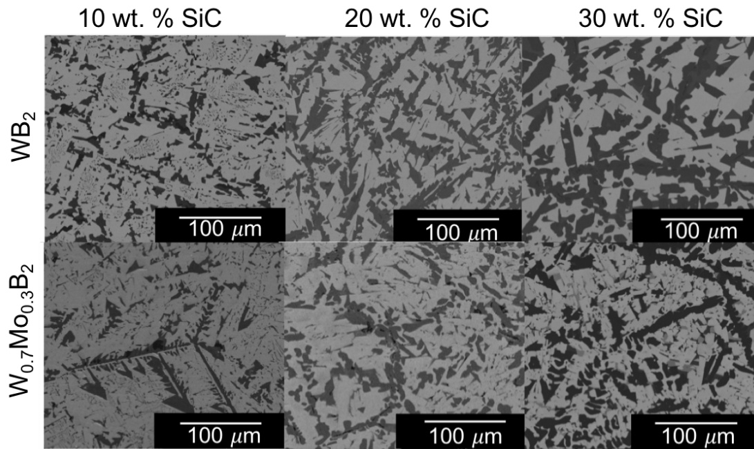
FIG. 2.7. SEM images of (top) WB_2 and (bottom) W_{0.7}Mo_{0.3}B_2 with 10, 20, and 30 wt. % SiC addition. Light gray regions represent areas of WB_2 and W_{0.7}Mo_{0.3}B_2 , while dark gray regions represent SiC grains.
