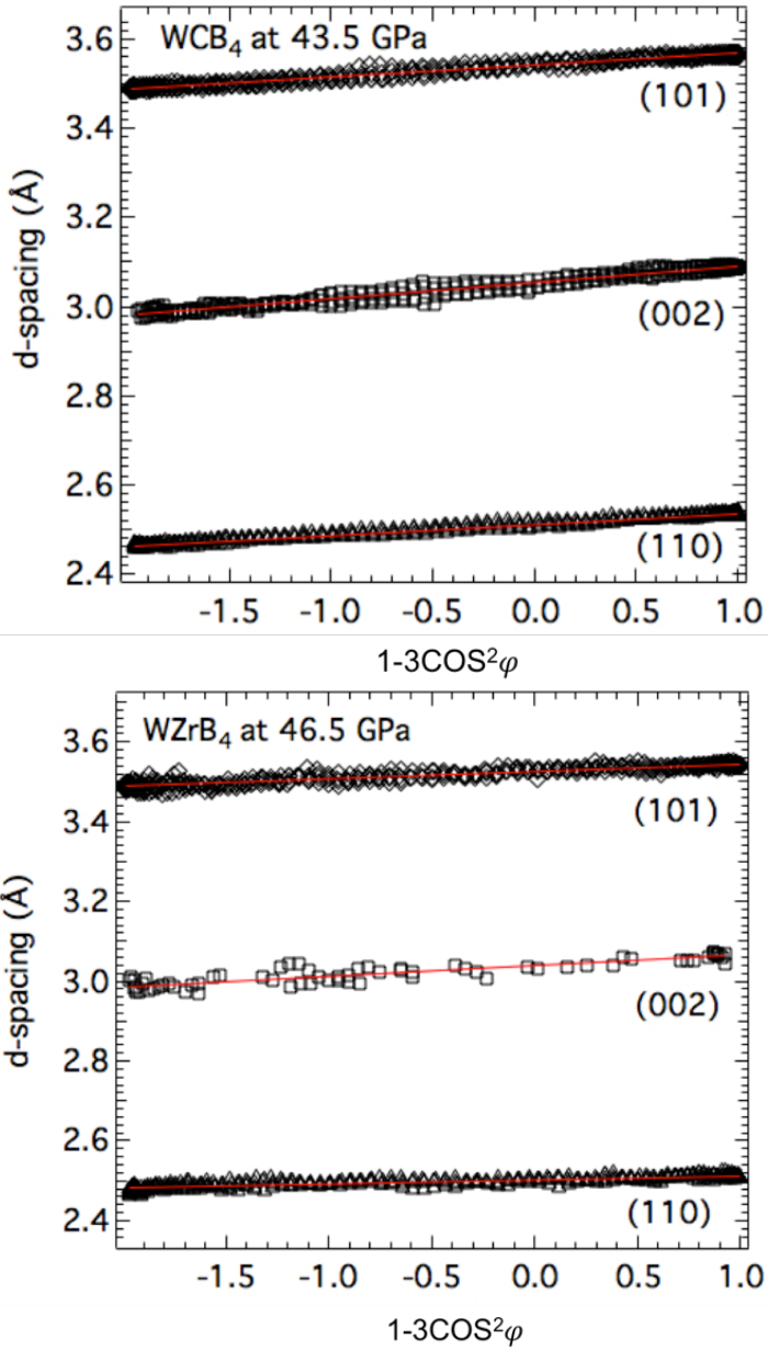
FIG. 4.9. Linearized plots of d spacings for W_{0.96}C_{0.04}B_4 (top) and W_{0.92}Zr_{0.08}B_4 (bottom) as a function of (1-3\cos^2\phi) at the highest pressure. Solid lines are the best linear fit to the data.
