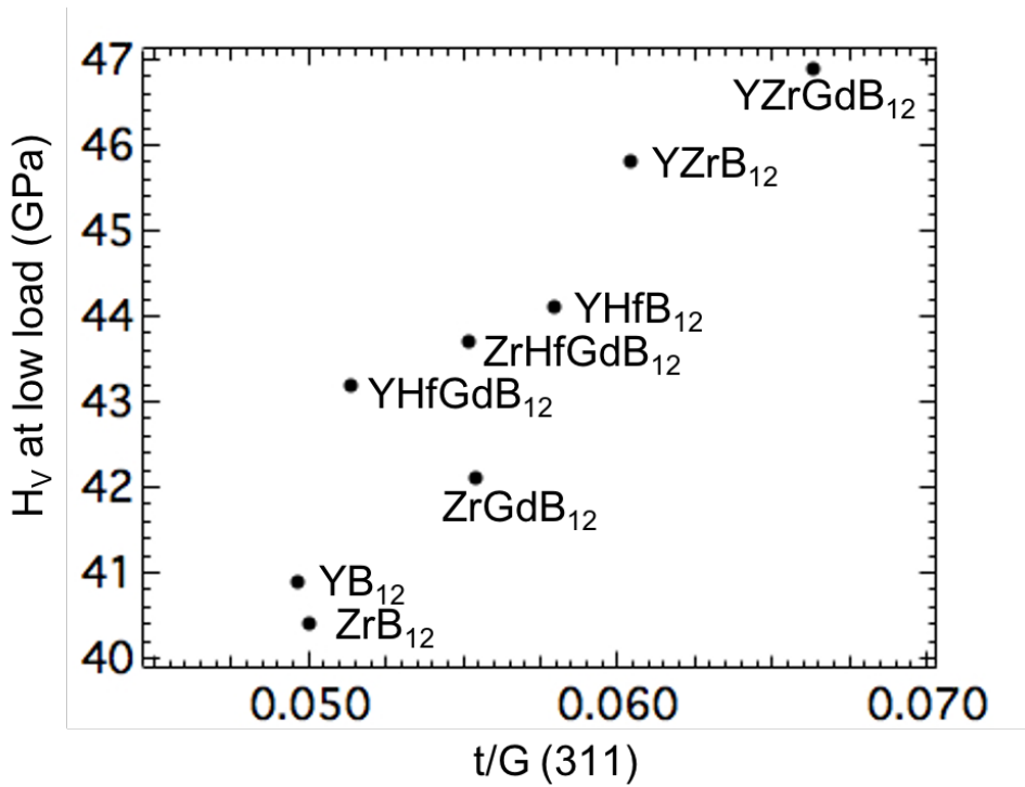
FIG. 5.6. Vickers hardness at low load (0.49 N) vs. the plateau value t/G of the (311) lattice plane for all MB_{12} samples ( ZrB_{12} , YB_{12} , Zr_{0.5}Y_{0.5}B_{12} , Y_{0.25}Hf_{0.75}B_{12} , Zr_{0.5}Gd_{0.5}B_{12} , Y_{0.5}Gd_{0.25}Hf_{0.25}B_{12} , Zr_{0.5}Gd_{0.25}Hf_{0.25}B_{12} and Y_{0.25}Zr_{0.5}Gd_{0.25}B_{12} ). The nominal composition of each MB_{12} solid solution is given for simplicity. A nearly linear correlation between plateau t/G value and Vickers hardness is observed.
