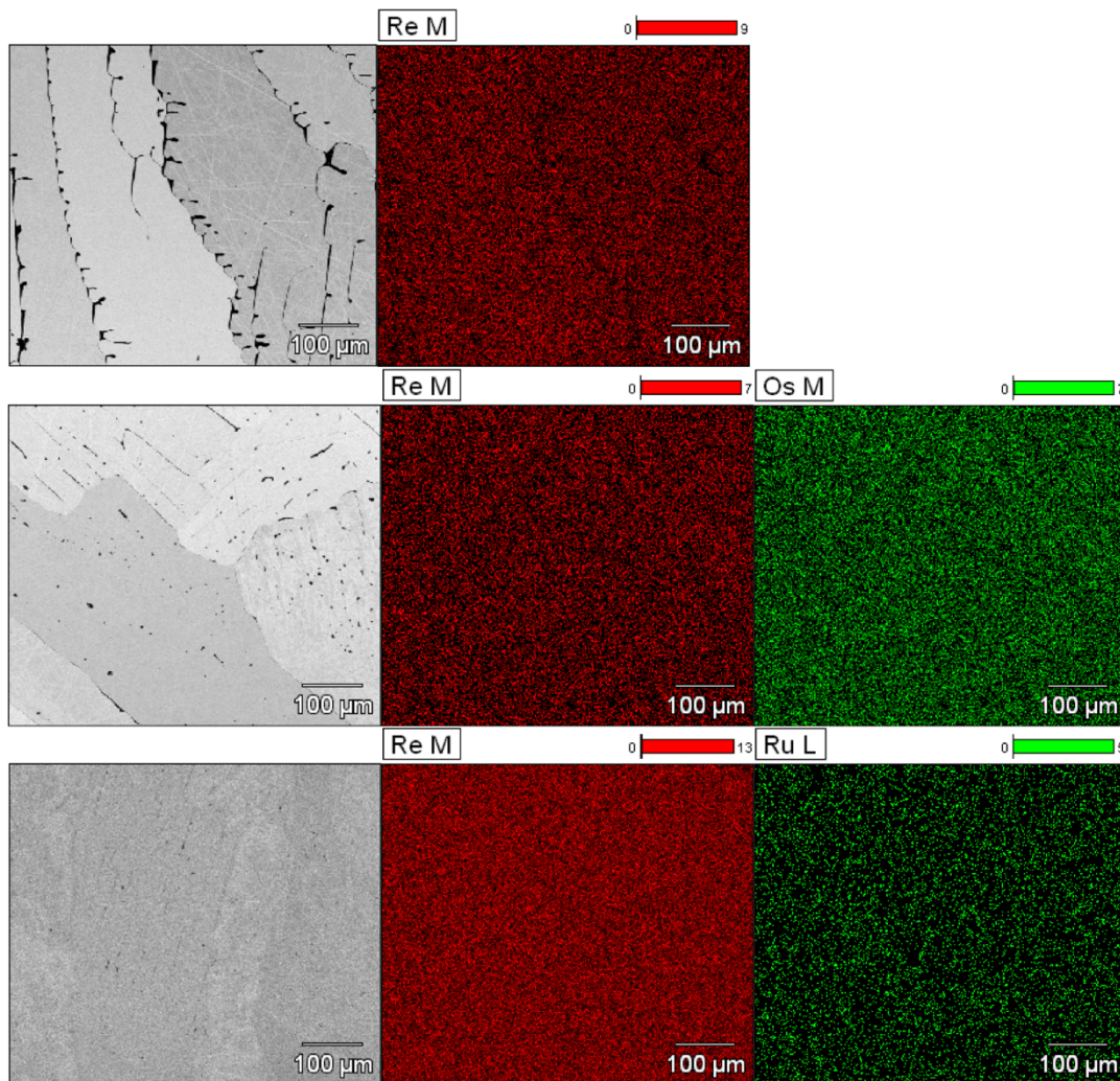
FIG. S3.2. SEM images and elemental maps for rhenium (M line), osmium (M line), and ruthenium (L line) for: (top) \text{ReB}_2 , (middle) \text{ReOsB}_2 , and (bottom) \text{ReRuB}_2 . The image and corresponding elemental maps were taken at 1000x magnification at 15 keV with scale bars of 100 \mu\text{m} .
