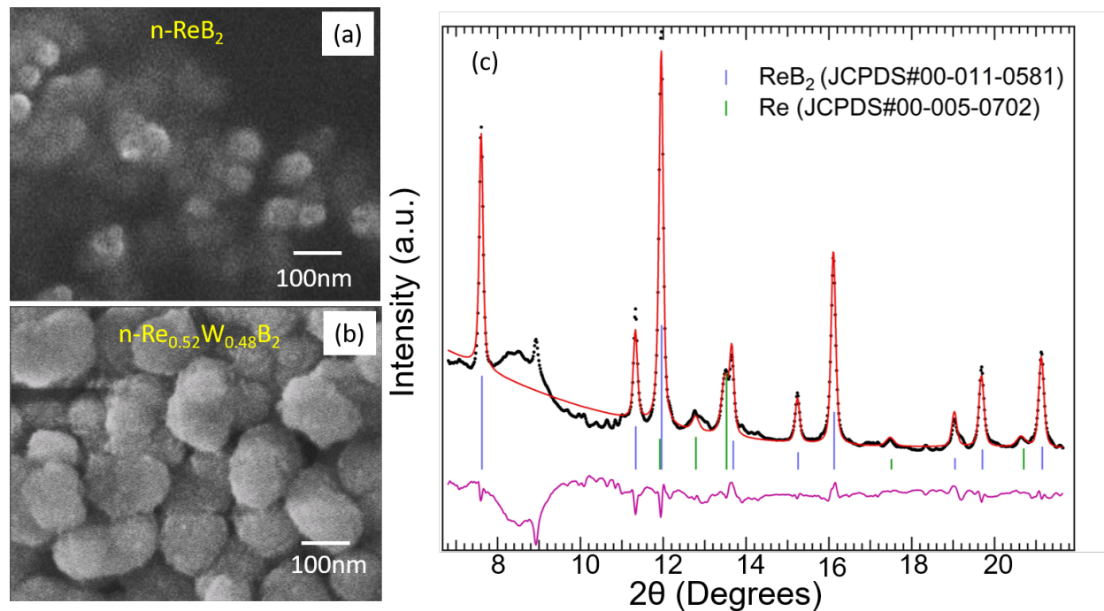
FIG. 6.3. Scanning electron microscopy images of (a) n\text{-ReB}_2 and (b) n\text{-Re}_{0.52}\text{W}_{0.48}\text{B}_2 prepared using an NaCl flux. Particle sizes range from \sim 40 to \sim 150 nm for the two samples. (c) Rietveld fitting of nano- \text{ReB}_2 at ambient pressure. The experimental spectrum is shown with a black dashed line, and the calculated fit is shown with a solid line in red. The difference pattern is shown in violet. Good agreement is found for all peaks other than those arising from the boron/epoxy gasket.
