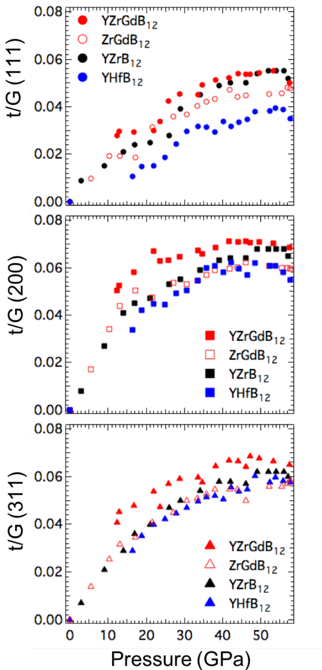
FIG. 5.5. Differential strain ( t/G ) as a function of pressure for Zr_{0.5}Gd_{0.5}B_{12} , Y_{0.5}Zr_{0.5}B_{12} , Y_{0.25}Zr_{0.5}Gd_{0.25}B_{12} , and Y_{0.25}Hf_{0.75}B_{12} . The nominal composition of each MB 12 solid solution is used in the legend for simplicity. Similar trends in the plateau value of the differential strain are found in all lattice planes.
