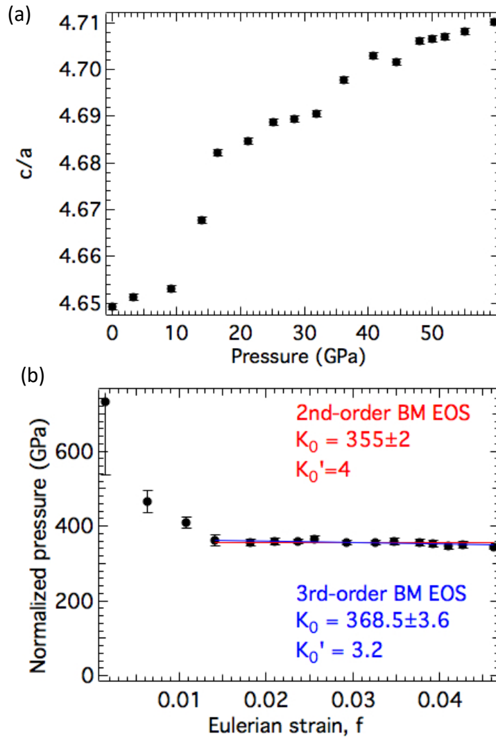
FIG. 2. 5. (a) Evolution of c/a upon pressure for W_{0.70}Mo_{0.30}B_2 obtained at the magic angle. (b) Normalized pressure ( F ) as a function of Eulerian strain ( f ). Second-order (red) and third-order (blue) Birch-Murnaghan equation-of-state fits.
