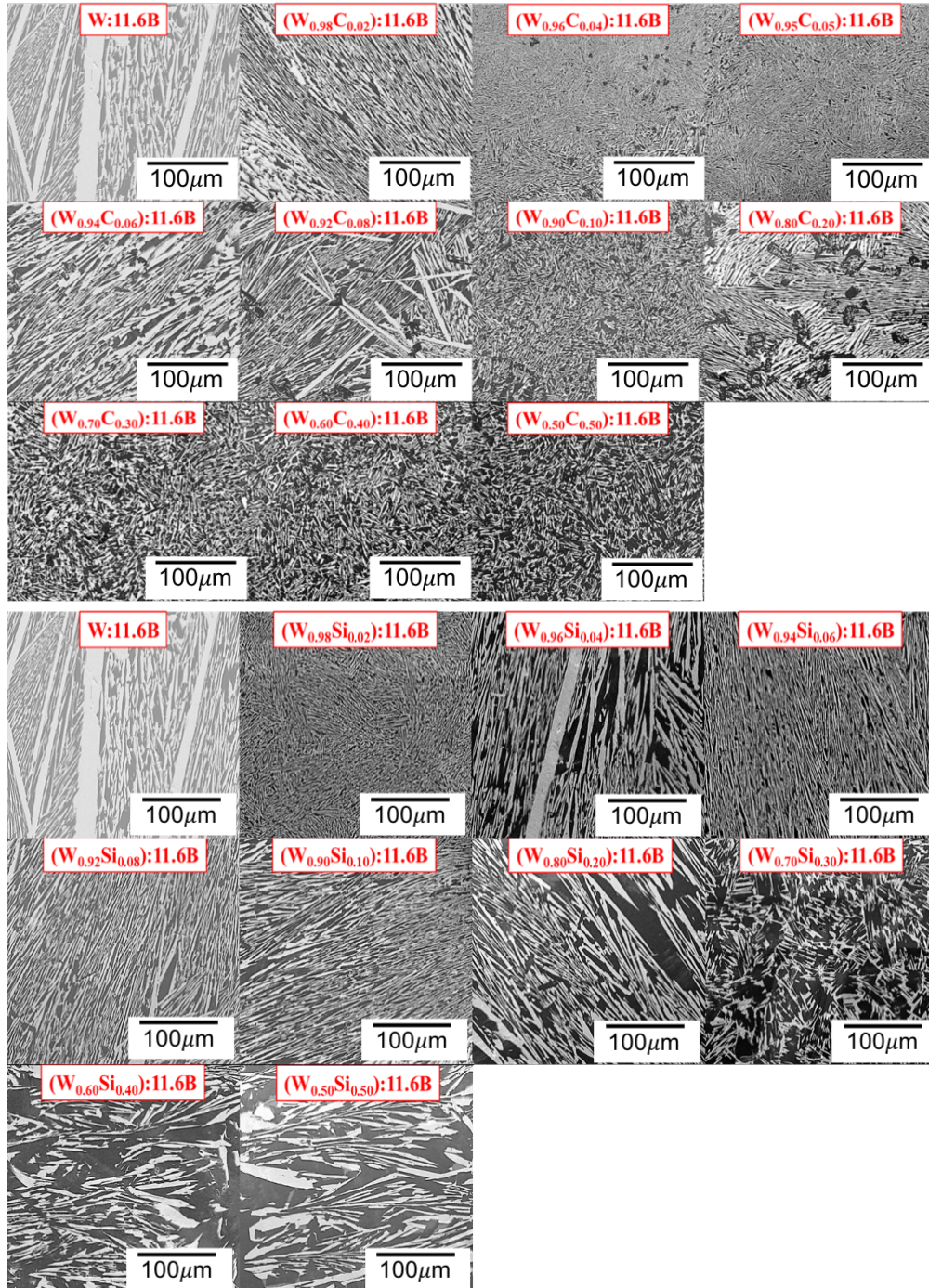
FIG. 4.5. SEM images for alloys of WB 4 with a nominal composition of (top) (W 1-x C x ): 11.6B and (bottom) (W 1-x Si x ): 11.6B showing a change in surface morphology associated with the effects of carbon and silicon and secondary phase formation. All SEM images were taken at 1000× magnification; the scale bars are 100 μm.
