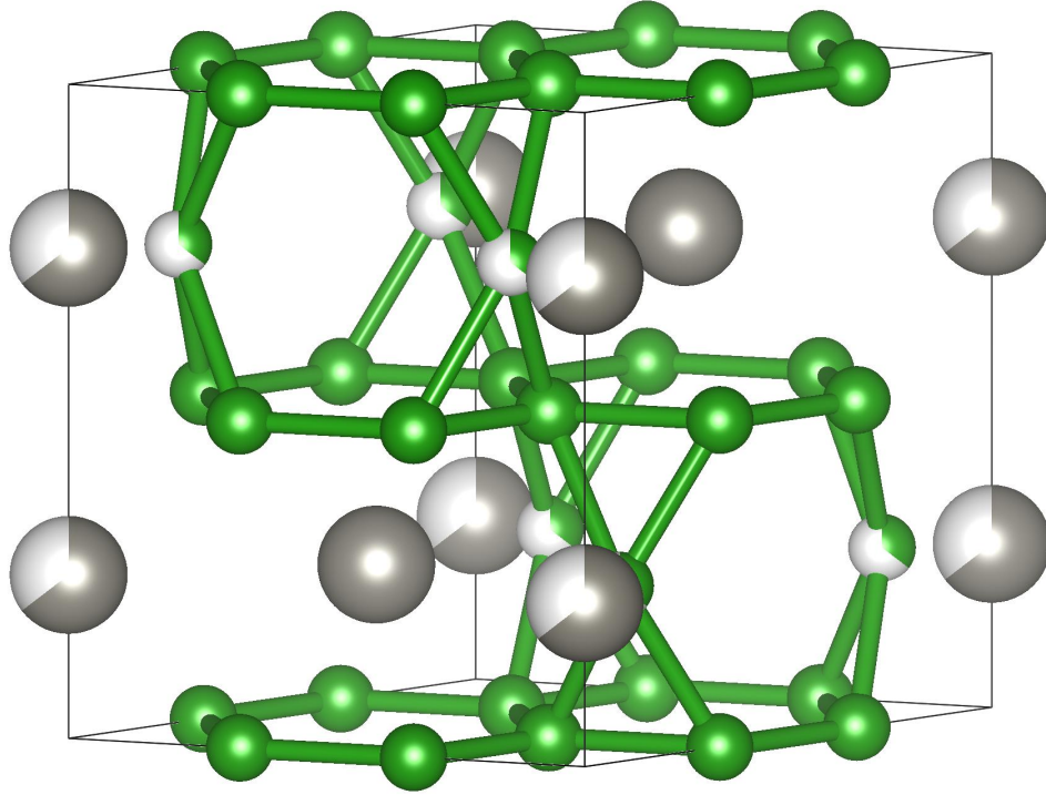
FIG. 4.1. Crystal structure of WB 4 with the P6_3/mmc space group (ICSD (Inorganic Crystal Structure Database) 291124). 51 Tungsten atoms are shown in gray, while boron atoms are in green; partially occupied positions are depicted by half-filled atoms.
