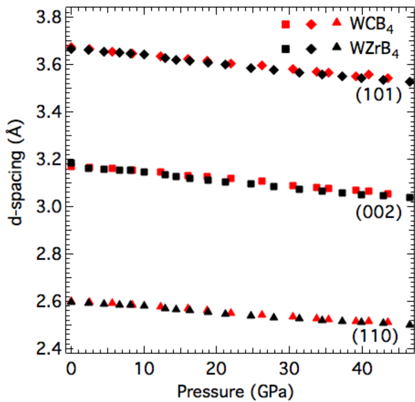
FIG. 4.8. Selected d spacings vs. pressure collected at \varphi = 54.7^\circ for W_{0.96}C_{0.04}B_4 and W_{0.92}Zr_{0.08}B_4 .
