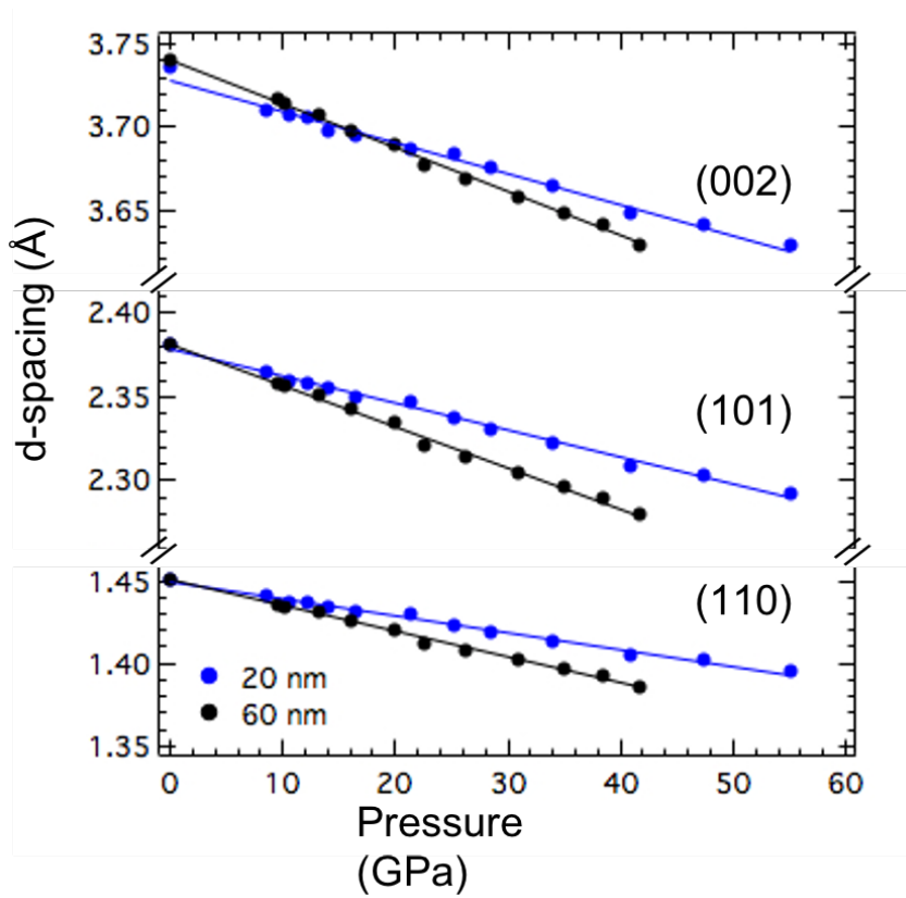
FIG. 7.3: Measured d-spacings for selected lattice planes of 20 nm- and 60 nm-ReB 2 as a function of pressure.
