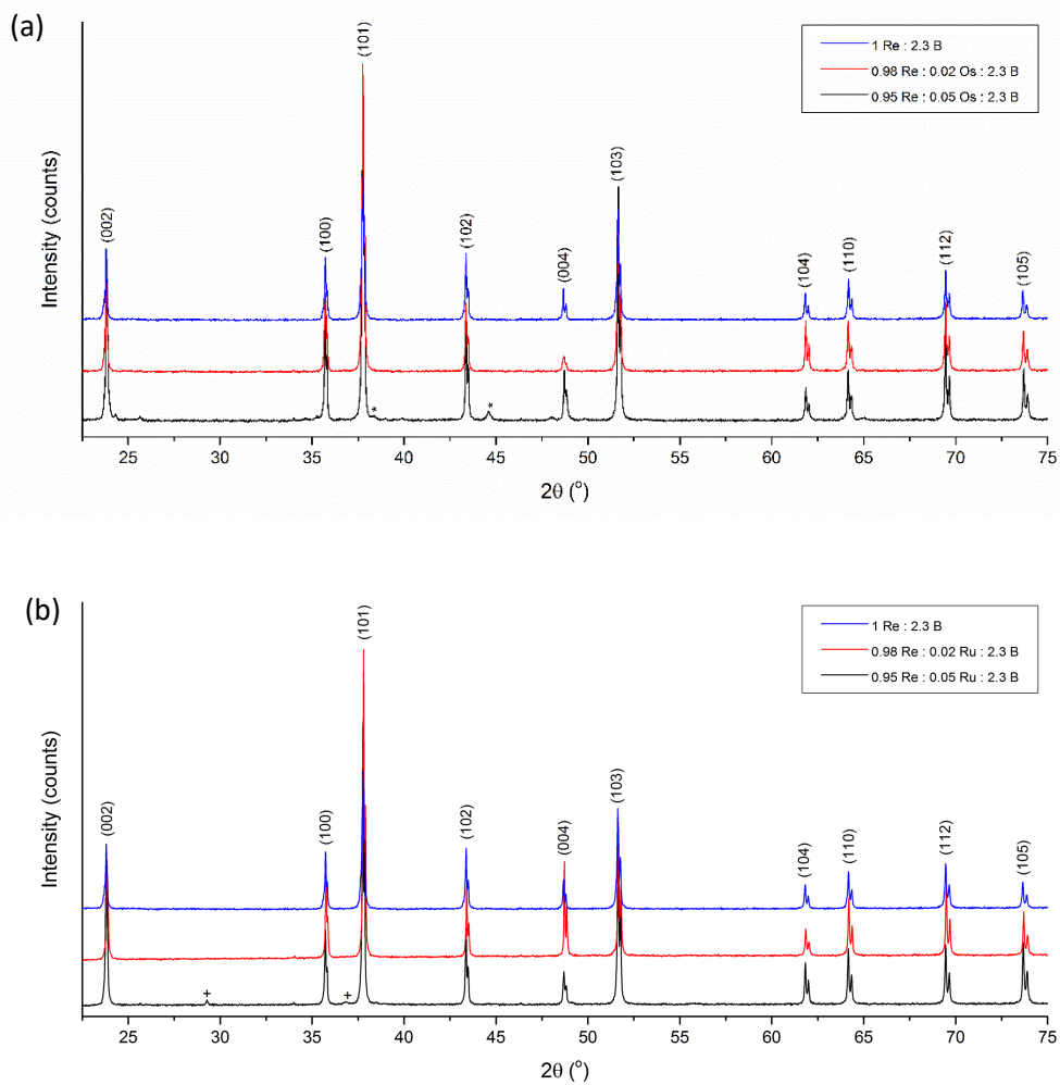
FIG. S3.1. PXRD data of: (a) \text{Re}_{1-x}\text{Os}_x\text{B}_2 and (b) \text{Re}_{1-x}\text{Ru}_x\text{B}_2 , where x = 0 - 0.05 and the total metal to boron ratio (M : B) used was 1 : 2.3. Peaks were assigned using \text{ReB}_2 (JCPDS 00-011-0581). Additional phases, \text{OsB}_2 (JCPDS 01-089-2672) and \text{RuB}_2 (JCPDS 01-089-2671) are denoted as (*) and (+), respectively.
