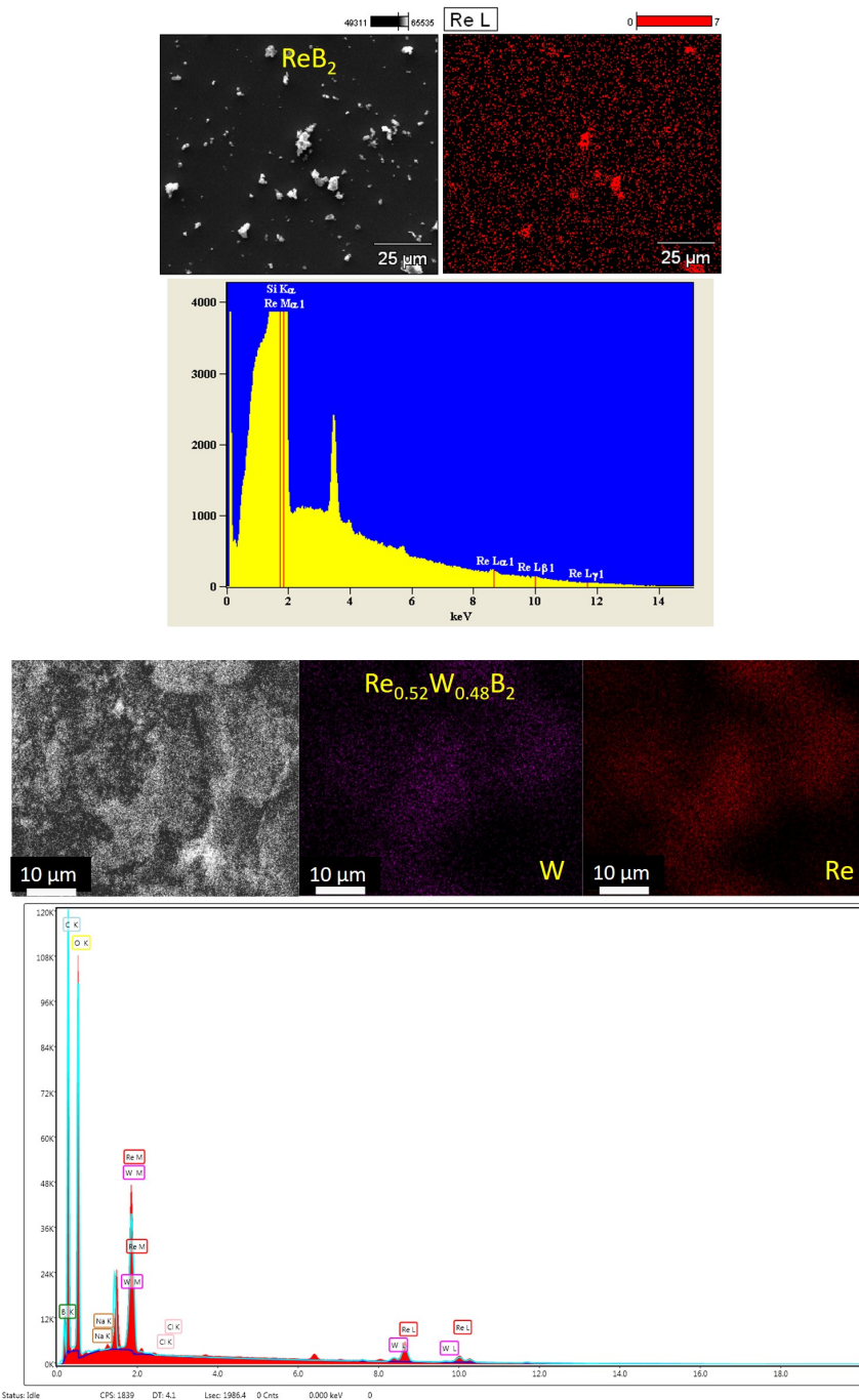
FIG. S6.3. SEM-EDS maps of \text{ReB}_2 and \text{Re}_{0.52}\text{W}_{0.48}\text{B}_2 . W and Re co-localize in the elemental maps, indicating alloyed material.
