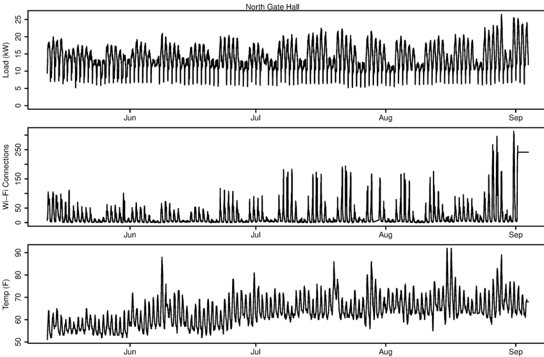
Figure 11. Load, Wi-Fi, and Temperature data for UC Berkeley North Gate Hall
