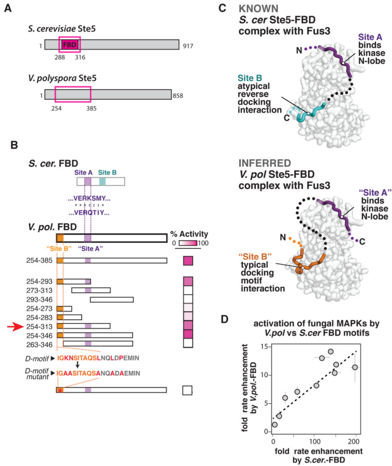
Figure 5. Dissection of the V. pol. Ste5-FBD motif with intermediate allosteric activity reveals alternative paths for coopting the same latent regulatory features (A) Position of minimal S. cer. Ste5-FBD sequence mapped previously (Bhattacharyya et al., 2006) and initial region of V. pol. Ste5 that showed FBD activity that serves as the starting point for further analysis. (B) Truncation mapping of the V. pol. Ste5-FBD fragment, showing the relative activity of an indicated truncation or fragment (see also Fig. S5). This analysis identifies two sites that are required for activity. One site (“Site A”) is similar to a sequence required for activity in the S. cer. Ste5-FBD fragment. A second site (“Site B”) resembles a traditional MAPK docking peptide sequence. (C) Comparison of the known structure of the S. cer. Ste5-FBD•Fus3 complex to the inferred structure based on homology and the truncation mapping from (B). The two kinases appear to use similar “Site A” sequences to bind the N-lobe of the kinase but use distinct mechanisms to engage the docking groove of the MAP kinase C-lobe. (D) A plot indicating the magnitude (mean ± SEM) of the S. cer. FBD effect and V. pol. FBD effect; each point corresponds to an individual kinases we inspected. The tight linear relationship between these effects suggests that both the S. cer. and V. pol. Ste5-FBD sequences target the same allosteric features and diversity present in the MAP kinases we inspected.
