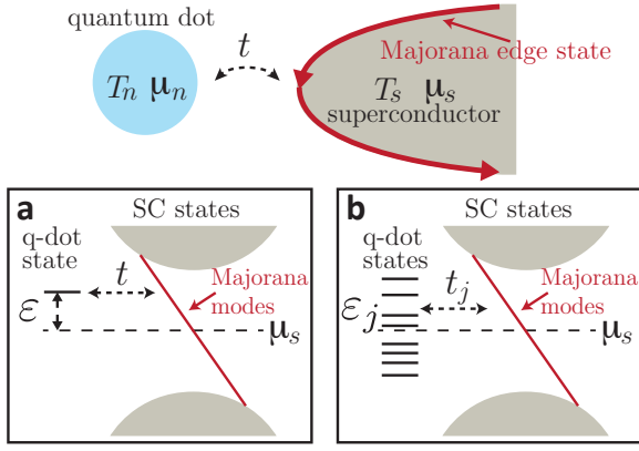
FIG. 1: The upper panel schematically depicts a quantum dot weakly coupling to a Majorana edge state. The temperature and chemical potential of the quantum dot are T_n and \mu_n , respectively, and those of the Majorana edge state are T_s and \mu_s . (a) A quantum dot with a single energy level \varepsilon is coupled to a Majorana edge state with tunneling strength t . (b) Multiple energy levels \varepsilon_j of a quantum dot are coupled to a Majorana edge state with tunneling strengths t_j for each state.
