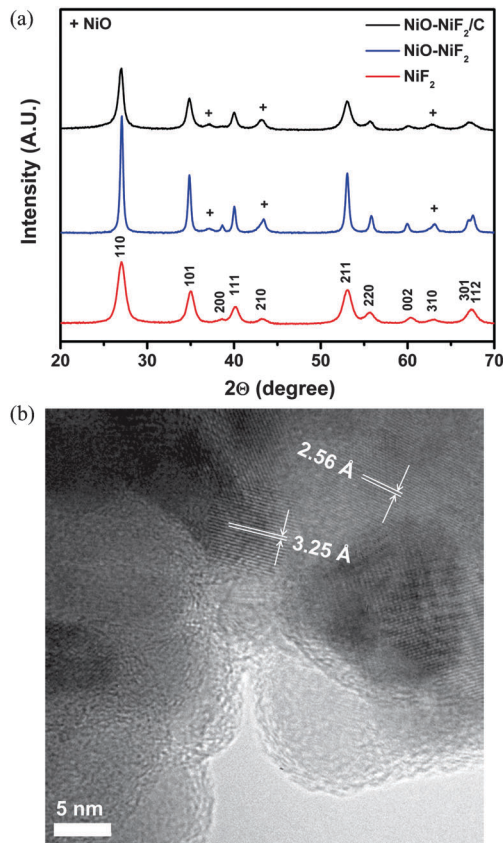
Fig. 1 (a) XRD patterns of NiO–NiF 2 –C (black), and pure NiF 2 (red) and NiO–NiF 2 (blue) for comparison. ( hkl ) marks the Bragg diffractions related to NiF 2 , P4_2/mnm and (+) indicates the NiO phase, and (b) TEM micrographs of as-prepared NiO–NiF 2 –C powder.
