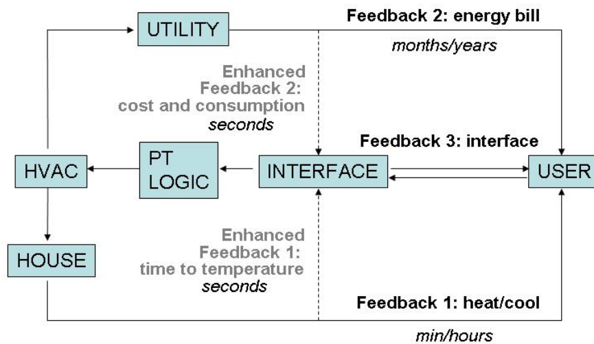
Figure 28: Human-thermostat interaction
