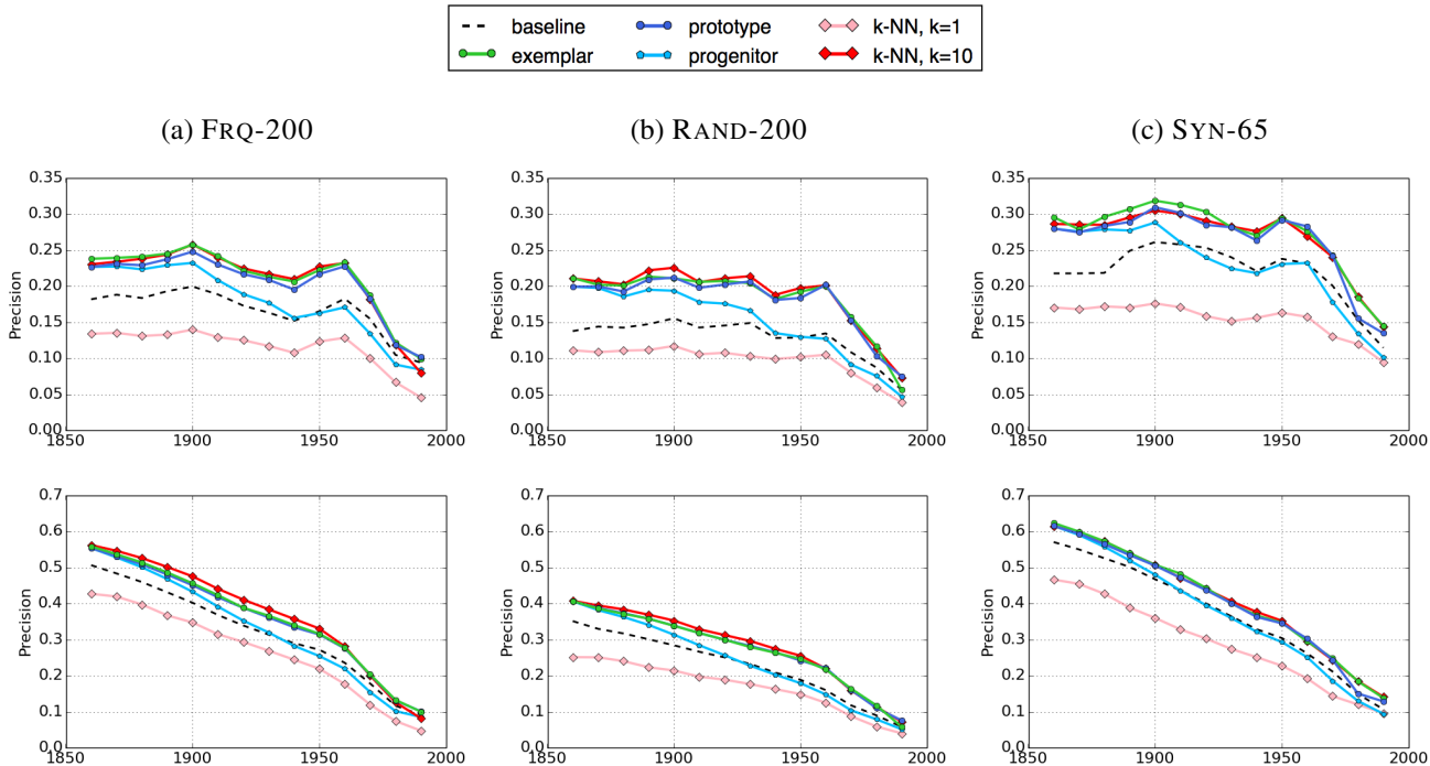
Figure 4: Model predictive accuracy on the FRQ-200, RAND-200, and SYN-65 adjective sets. Top row: Predictive accuracy when only novel adjective-noun pairs in the following decade are considered. Bottom row: Predictive accuracy when all future adjective extensions are considered.
