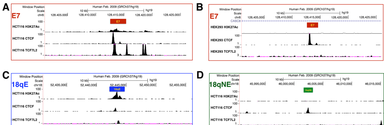
Figure 4. H3K27Ac, TCF7L2, and CTCF binding profiles of E7, E24, 18qE and 18qNE. Shown are the H3K27Ac, TCF7L2 and CTCF binding patterns at (A) the E7 enhancer in HCT116 cells, (B) the E7 enhancer in HEK293 cells, (C) 18qE, an intergenic H3K27Ac peak on chromosome 18, in HCT116 cells and (D) 18qNE, an intergenic region on chromosome 18 that lacks the H3K27Ac mark, in HCT116 cells. The Y-axis indicates the peak height and the X-axis indicates the genomic location; the boxes indicate the region deleted by the CRISPR/Cas9 method.
