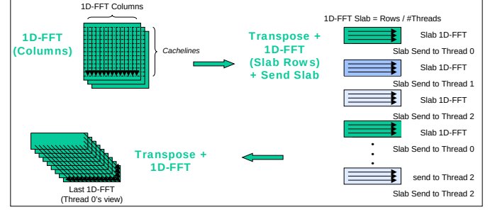
Figure 7. Illustration of the blocking exchange algorithm for communication in FT, used by the stock Fortran+MPI code, and the non-blocking overlapped slabs algorithm for communication in FT, which provided the best performance in the Titanium code.
