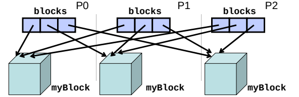
Figure 3. Distributed data structure built for MG.
