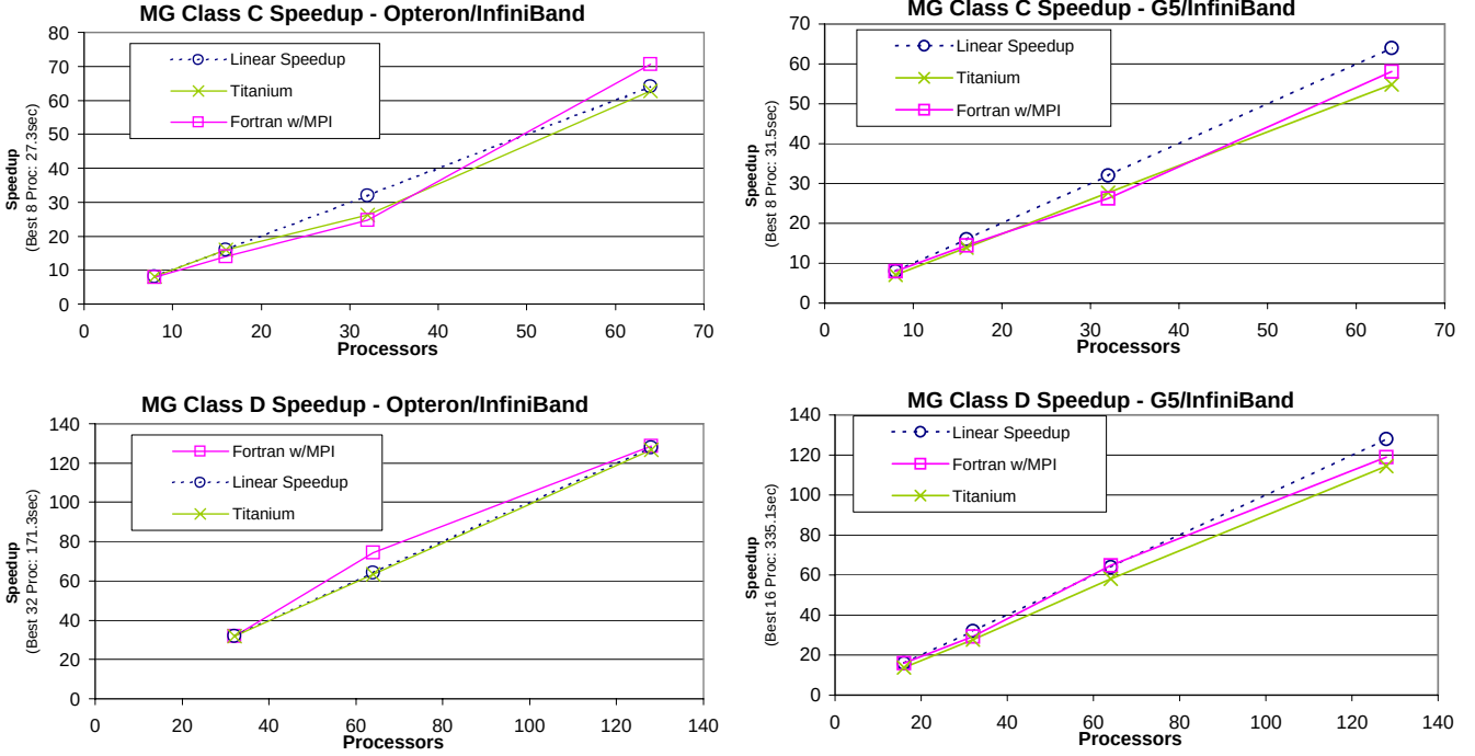
Figure 9. MG performance comparison
