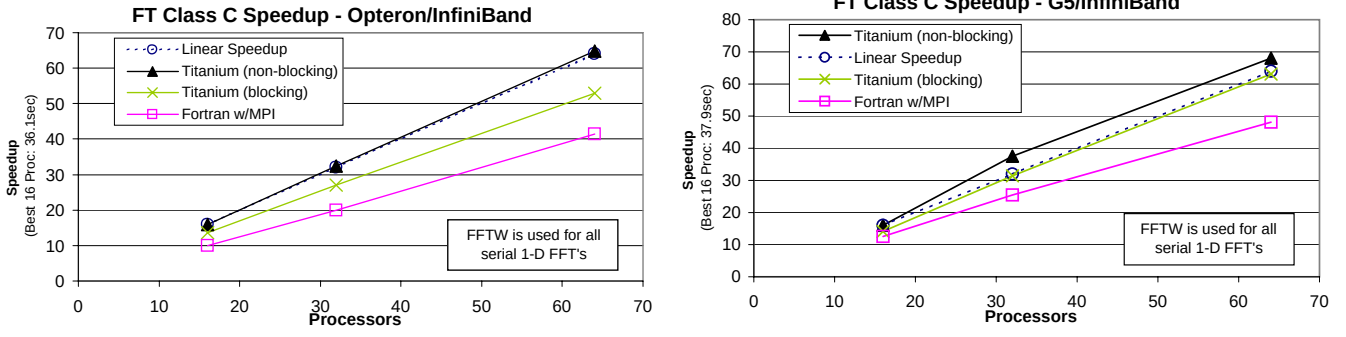
Figure 8. FT performance comparison
