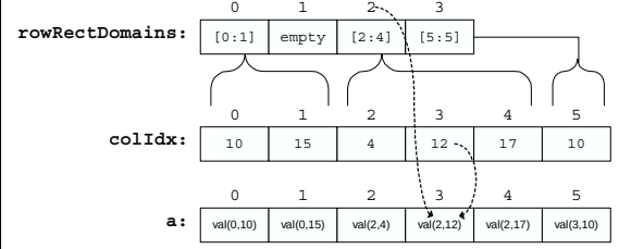
Figure 5. CSR format for sparse array data.
