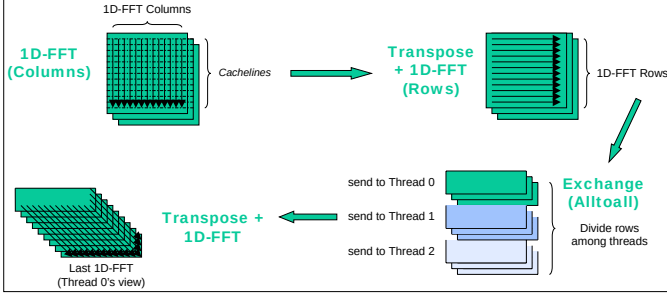
Figure 7. Illustration of the blocking exchange algorithm for communication in FT, used by the stock Fortran+MPI code, and the non-blocking overlapped slabs algorithm for communication in FT, which provided the best performance in the Titanium code.
