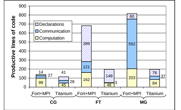
Figure 4. Timed region line count comparison
