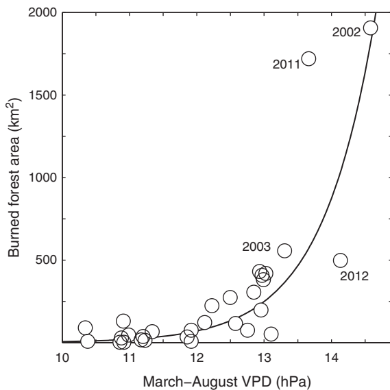
Fig. 6. Annual burned forest area v. mean March–August vapour pressure deficit (VPD) in forest during 1894–2013. As in Fig. 2a, but values are not adjusted for autocorrelation and y -axis is not on a log scale. The four largest burned area years are labelled.
