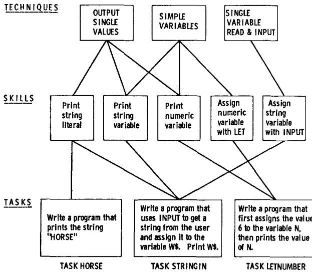
FIG. 2. A simplified portion of the curriculum network.
