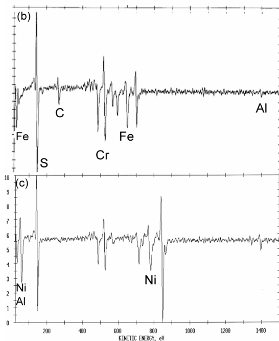
Figure 7: (a) S build up with oxidation time at \text{Al}_2\text{O}_3/\text{FeCrAl} interface. (b) Typical AES spectrum of the saturation level on most FeCrAl interfaces (shaded area) and (c), spectrum of the NiCrAl interface.
