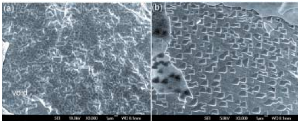
Figure 5: SEM micrographs showing the alloy surface of after scratch induced scale spallation. (a) Ni40Al, 1000^\circ\text{C} , 26h and (b) Ni-40Al(S), 1000^\circ\text{C} , 10min.
