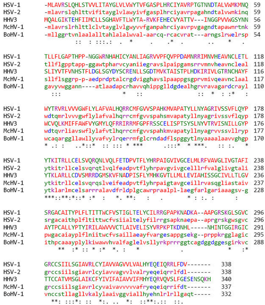
FIGURE 1 | gK protein sequence alignment in different strains of alphaherpes viruses. Protein sequence was aligned by clustal omega and percentage of amino acid homology was compared among different groups of Herpes viruses. HSV-1 has 85% homology with HSV-2, 66% homology with McHV-1, 34% homology with BoHV-1, and 28% homology with VZV. Stars (*) indicate that the amino acids sequences are the same.
