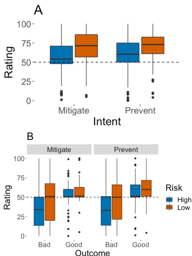
Figure 2. Results of Experiment 2. A) Prospective ratings. B) Retrospective ratings. The dashed line at 50 marks the point on the scale labeled "appropriate response".
